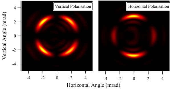
Figure 7. Vertically and Horizontally polarised components of visible SR from a 500 MeV electron beam crossing an undulator with 3 periods, K=1.3 , \lambda_u=12 cm. Simulated with SRW.
