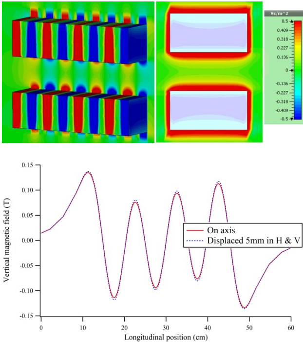
Figure 2. Field quality of an undulator with g = \lambda_u . Top left, vertical magnetic field B_y on centre plane of undulator. Top right, transverse map of B_y at longitudinal peak. Bottom, B_y along undulator axis (solid red line) and displaced by 5mm in H and V (dotted blue line).
