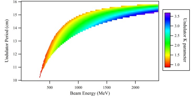
Figure 3. Undulator period and K parameter needed to produce 500 nm light at an opening angle of 2.5 mrad for different beam energies.
