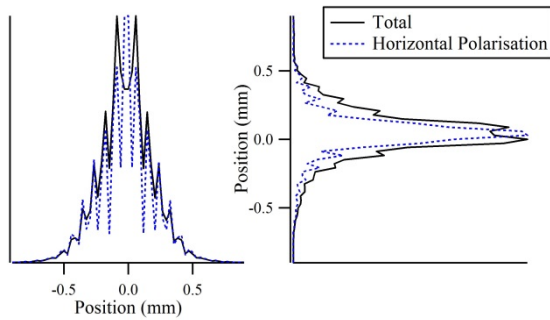
Figure 8. Horizontal and vertical size of the point spread function of visible SR from a 500 MeV electron beam crossing an undulator with 3 periods, K=1.3 , \lambda_u=12 cm. Simulated with SRW and ZEMAX.
