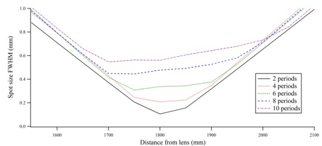
Figure 6. Focused beam waist of SR from undulators of different lengths. From ZEMAX simulation of a simple optical simple with 1:1 imaging.
