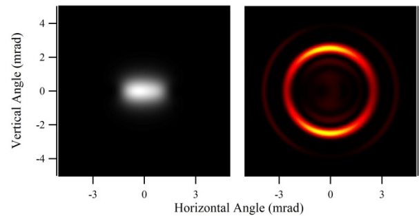
Figure 4. Total SR (left) and visible SR (right) from a 500 MeV electron beam crossing an undulator with 3 periods, K=1.3 , \lambda_u=12 cm. Simulated with SRW.
