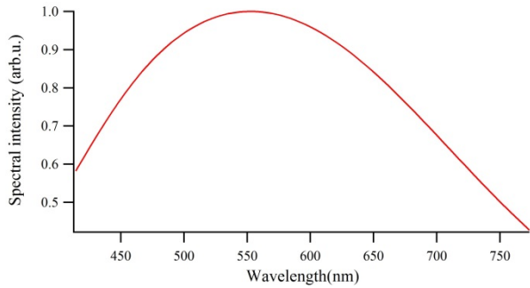
Figure 5. Spectrum of SR emitted with angle 2-3 mrad from a 500 MeV electron beam crossing an undulator with 3 periods, K=1.3 , \lambda_u=12 cm. Simulated with SRW.
