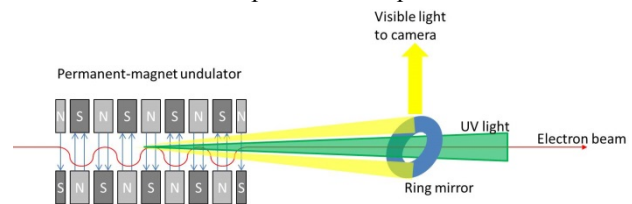
Figure 1. Schematic of off-axis SR observation
