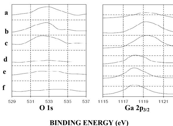
Figure 2: XPS spectra of the Ga 2p 3/2 and O 1s for: (a) the initial dirty sample; (b) after heating to 450 °C; (c) after heating to 500 °C; (d) after heating to 550 °C; (e) after heating to 600 °C and (f) after heating to 625 °C.
