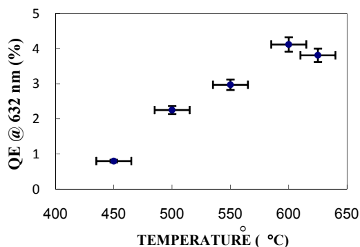
Figure 3: QE as a function of heat-cleaning temperature.
