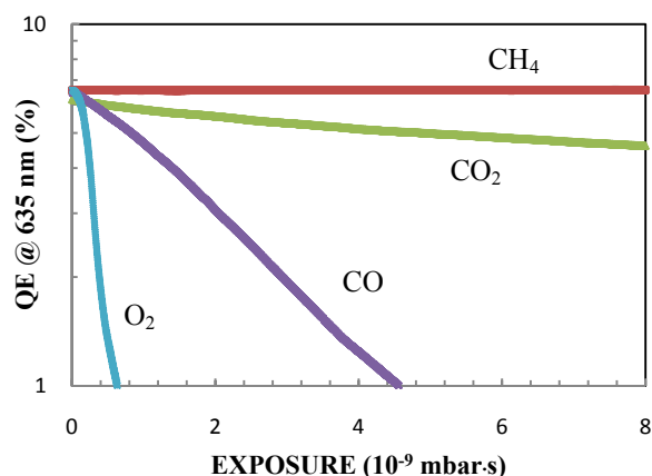
Figure 7: Decrease of QE of the photocathode due to exposure to different gasses.
