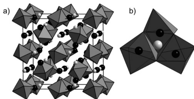
Figure 1. (a) Garnet structure of \text{Li}_5\text{La}_3\text{Ta}_2\text{O}_{12} contains lithium in both tetrahedral and octahedral coordinations. Octahedra represent \text{TeO}_6 units and dark and light spheres represent lanthanum and the tetrahedrally coordinated lithium, respectively. (b) The oxide tetrahedron housing \text{Li}^+ on the 24d site (light gray) shares each face with an oxide octahedron, accommodating additional \text{Li}^+ on the 48g site (dark gray).
