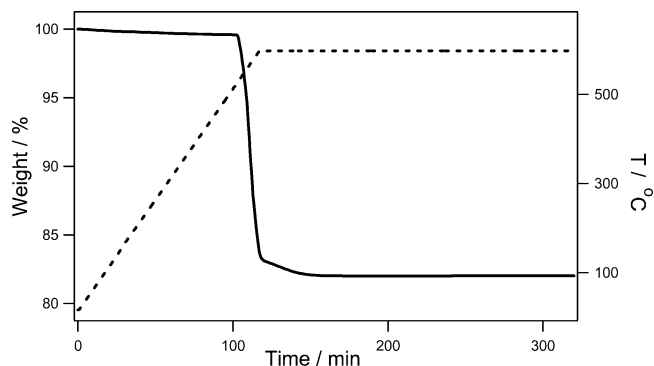
Figure 7. Variation in mass (solid line) as a function of temperature (dotted line) for \text{Li}_3\text{Nd}_3\text{Te}_2\text{O}_{12} heated under a flowing atmosphere of 5% \text{H}_2 in \text{N}_2 .
