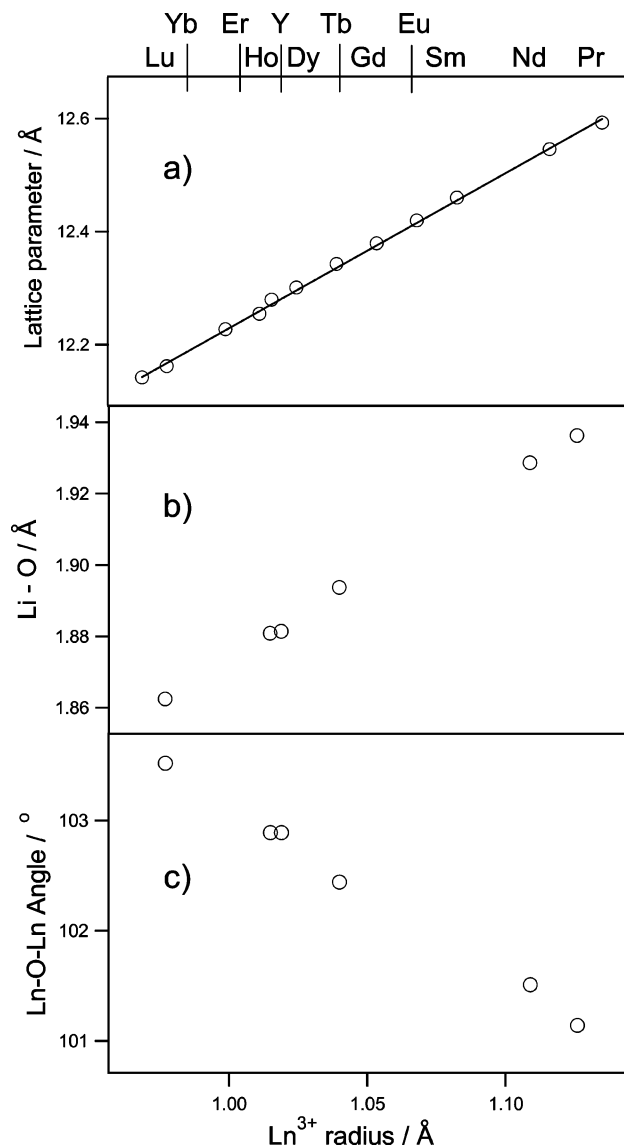
Figure 9. The variation in (a) lattice parameter, (b) lithium oxide bond length, and (c) \text{Ln}-\text{O}-\text{Ln} angle in \text{Li}_3\text{Ln}_3\text{Te}_2\text{O}_{12} as a function of the radius of \text{Ln}^{3+} . The fitted line shown in (a) illustrates that this series obeys Vegard's law.
