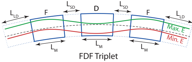
Figure 1: Geometry of the FFAG cell optimised in NORMA. Variable parameters were the cell length L_{cell}=2L_{LD}+3L_M+2L_{SD} , the triplet length L_{trip}=3L_M+2L_{SD} , and the packing factor \alpha=L_{trip}/L_{cell} .
