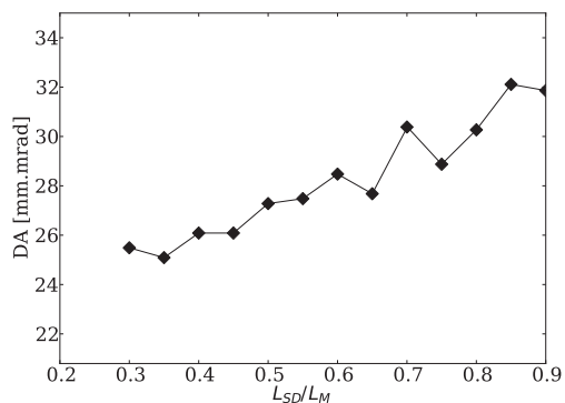
Figure 6: The variation of dynamic aperture in the NORMA ring when the ratio L_{SD}/L_M is changed and \alpha=0.62 .
