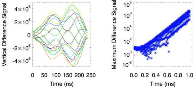
Figure 9: Left - Simulated vertical difference signal over the last 20 turns. Right - Maximum vertical offset over 800 turns (blue) with exponential fit (red) for \xi = -0.82 ( \chi = 5.31 \text{ rad} ).
