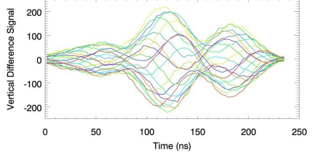
Figure 5: Simulated vertical difference signal over the last 20 turns of the simulation with nominal tune at 1 ms.
