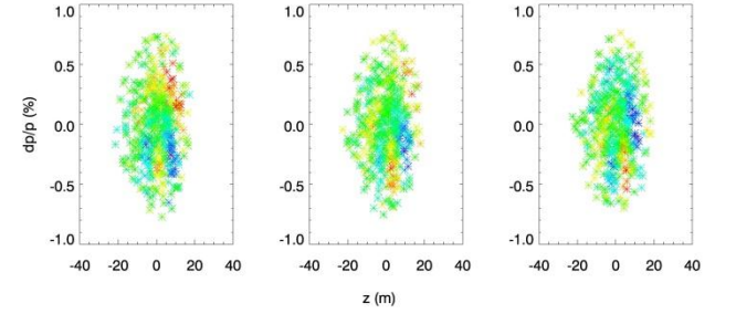
Figure 12: Longitudinal phase space on turn 780 (left), 790 (centre) and 800 (right) for \xi = -1.2 . Colour denotes vertical offset for 2000 sample particles from negative (blue) to positive (red) with respect to centre.
