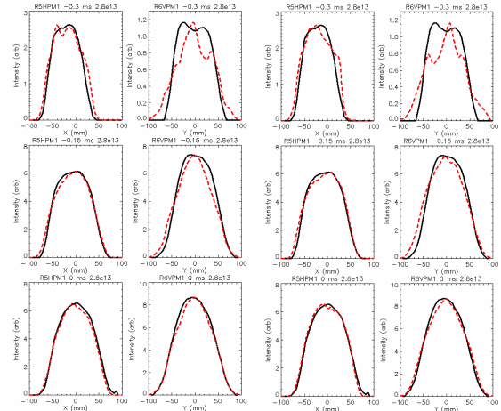
Fig 3: Measured (black) and Simulated (red) profiles at 3 machine time points. Left two columns, normal ISIS lattice. Right two columns, ISIS lattice with half integer driving terms.
