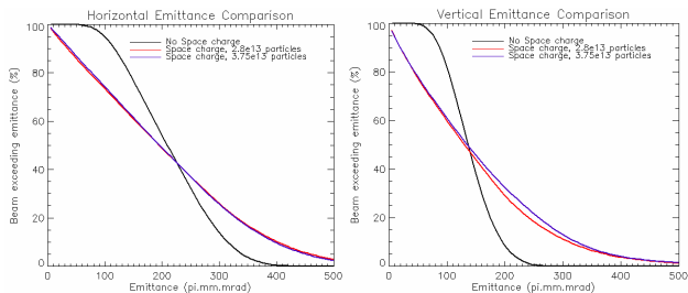
Figure 10. Emittance occupancy for ‘Anti-correlated’ painting as a function of simulated intensity.
