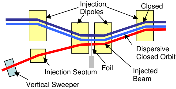
Fig 1: Schematic layout of ISIS injection system.
