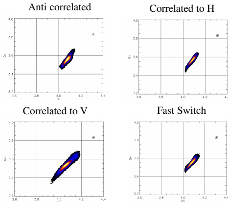
Fig 7: Single Particle Tune Diagrams at 2.8 \times 10^{13} ppp.
