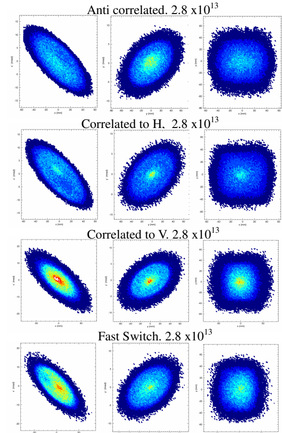
Fig 6: Phase Space and Real space distributions a 0 ms. Colour indicates particle density with same scale in all four cases.
