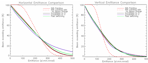
Fig 8 : Emittance occupancy for each painting case.
