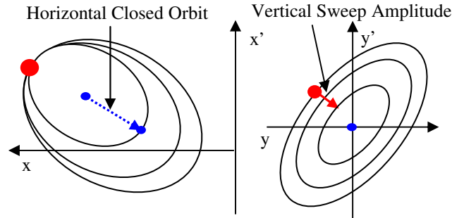
Fig 2: Phase space painting at Foil. Closed orbits in blue
