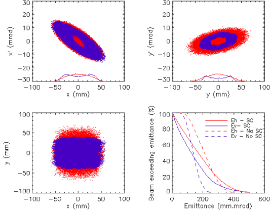
Fig 4: Phase space, Real space and Emittance occupancy of ISIS simulation at 0ms with and without space charge.
