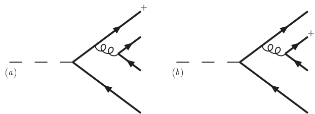
Figure 5: One of the diagrams contributing to the b\bar{b}b\bar{b} final state at \mathcal{O}(\alpha_S^2) . The dashed line represents either the axial or vector current. The cross indicates which of the two b quarks is triggered on: both contributions must be summed.
