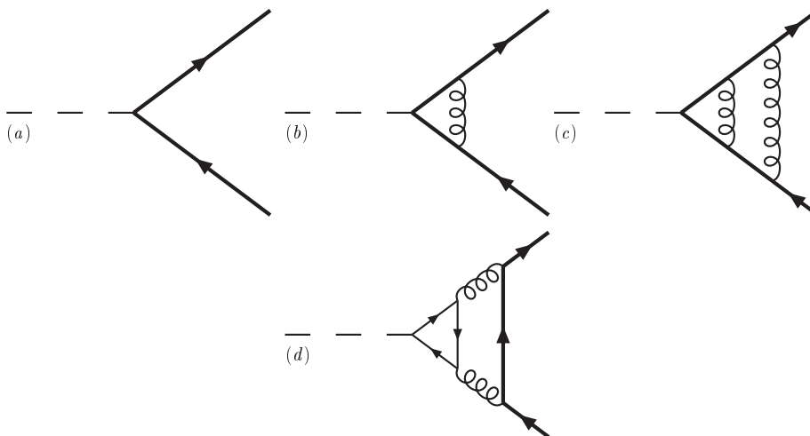
Figure 1: Some of the diagrams contributing to the b\bar{b} final state up to \mathcal{O}(\alpha_S^2) . The dashed line represents either the axial or vector current, the thick line the b and the thin line another quark q , which must be summed over flavours, including the b - and t -quark contributions.
