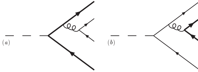
Figure 4: Some of the diagrams contributing to the b\bar{b}q\bar{q} final state at \mathcal{O}(\alpha_S^2) . The dashed line represents either the axial or vector current, the thick line the b and the thin line some other quark flavour q , with q \neq b .
