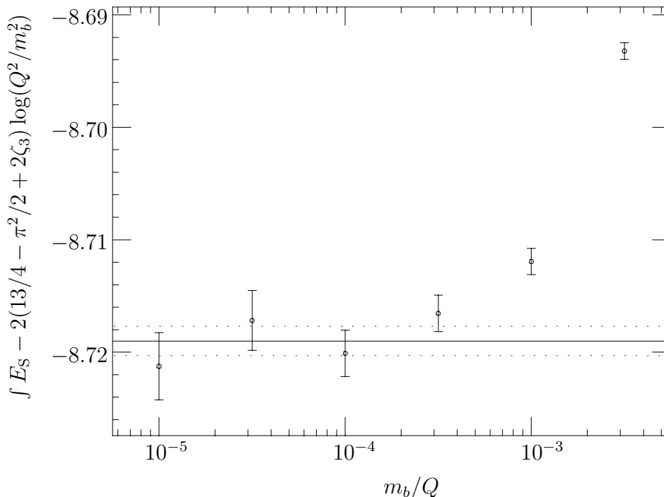
Figure 6: The term c in eq. (B.4) as a function of mass. The errors are purely from Monte Carlo statistics. The solid line is our fit to the limiting value and the dotted lines its error.
