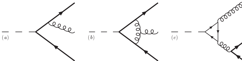
Figure 2: Some of the diagrams contributing to the b\bar{b}g final state up to \mathcal{O}(\alpha_S^2) . The dashed line represents either the axial or vector current, the thick line the b and the thin line another quark q , which must be summed over flavours, including the b - and t -quark contributions.
