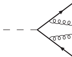
Figure 3: One of the diagrams contributing to the b\bar{b}gg final state at \mathcal{O}(\alpha_S^2) . The dashed line represents either the axial or vector current.
