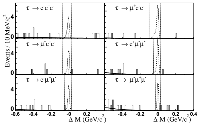
FIG. 2: Distribution of \Delta M for data (solid histogram) and background PDFs (solid curves) for events with \Delta E in the signal region indicated in Fig. 1. Expected signal distributions are shown (dashed histogram) for a branching fraction of 10^{-6} .
