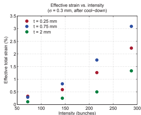
Figure 6: Peak residual effective strain after cool-down.
