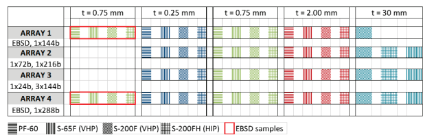
Figure 4: Test matrix illustrating the specimen type, size, grade, and incident beam intensities ( 1.7 \times 10^{11} protons per bunch).
