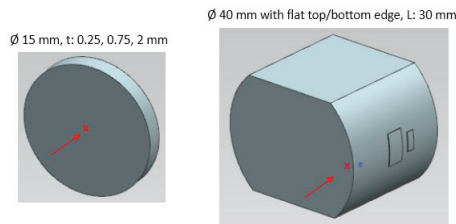
Figure 3: Specimen types: thin discs and slugs.
