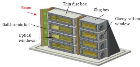
Figure 2: Interior of experiment chamber.
