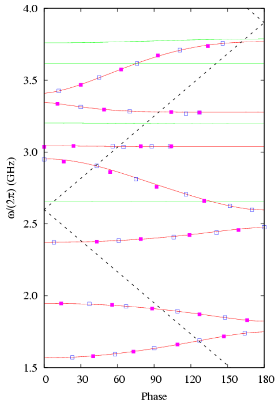
Figure 2: Brillouin diagram for 7 dipole bands. The light line is shown dashed.
