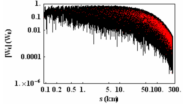
Figure 5: Transverse wakefield for 9-cell RE cavity ( W_0=0.19 V/pC/mm/m and, Q = 10^6 for all modes).
