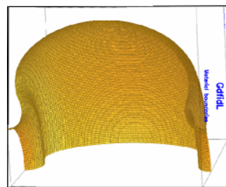
Figure 3: GdfidL mesh consisting of 1.45 \times 10^6 elements for a quarter section of a single RE cell. Each mesh element is separated from its neighbour by 1mm.
