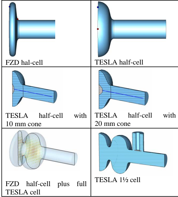
Figure 2: RF design of the first \frac{1}{2} cell and complete cavities that have been assessed
