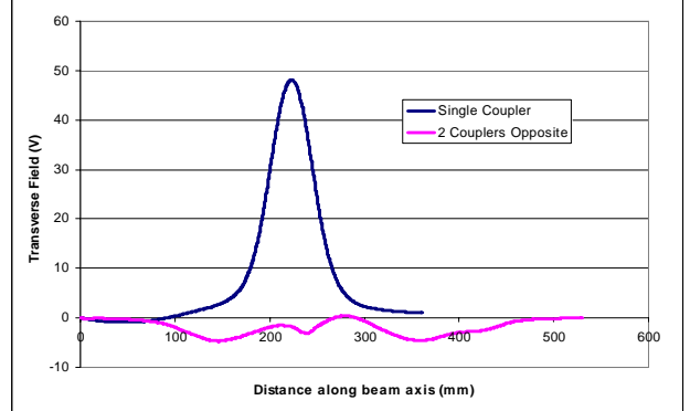
Figure 3: Transverse electric fields in the coupler's region
