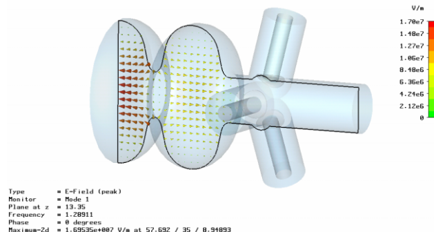
Figure 7: Electric field contours in a TESLA 1\frac{1}{2} cell cavity
