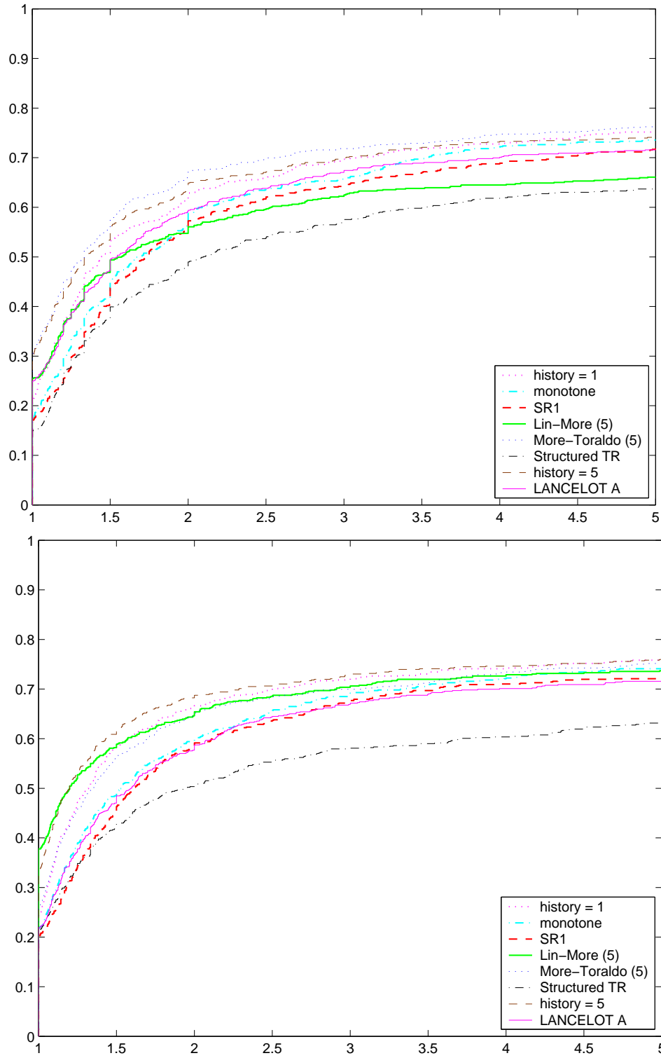
Figure 2.1: Performance profile for LANCELOT options: CPU times (top) and number of function evaluations (bottom). The horizontal axis is gives the argument \sigma , while the vertical axis records p_i(\sigma) for each of the competing options, i .
