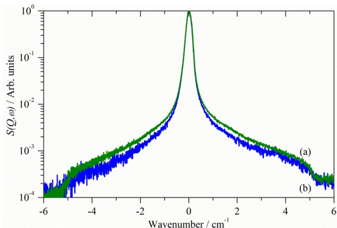
Fig. 4 Comparison of the QENS spectra at 2 K of \eta -alumina (olive) and (b) \gamma -alumina (blue) after reaction with methanol to generate methoxy.
