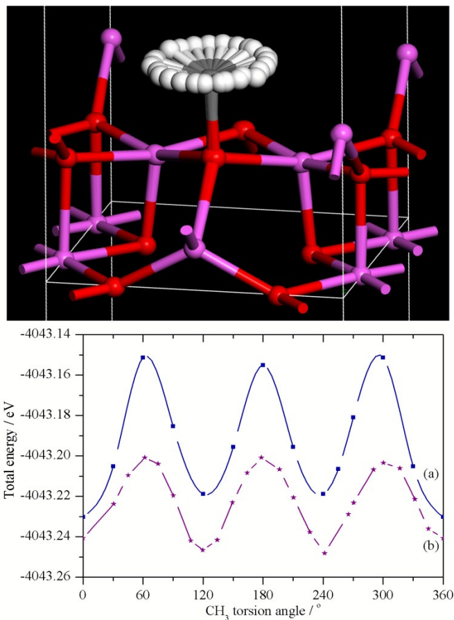
Fig. 8 Upper: model of methoxy on \eta\text{-Al}_2\text{O}_3 used to generate the rotational potential. (Magenta = Al, red = O, grey = C, white = H). Lower: rotational potential when: (a) the methyl group is held rigid and (b) when it is allowed to relax. Computational details are given in the ESI.
