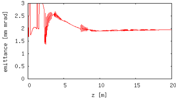
Figure 1: Evolution of emittance along the DC injector.
