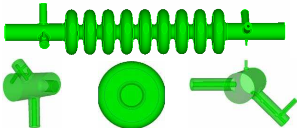
Figure 1: Model of the FNAL deflecting mode cavity with input and HOM couplers at left end and SOM and LOM couplers at right end.
