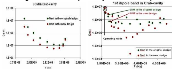
Figure 7: Omega3P damping results for the cavity with new LOM and HOM coupler designs.
