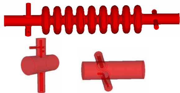
Figure 5: Model of the new deflecting mode cavity.
