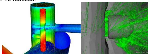
Figure 9: Resonant particle trajectories in the HOM coupler using Track3P.
