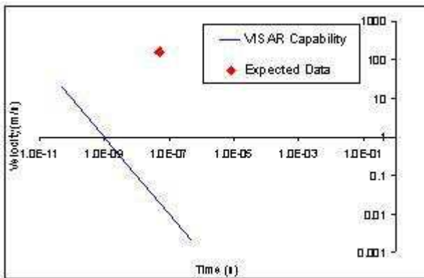
Figure 3: Comparison of VISAR measurement technique capability [11] with expected surface motion parameters determined from FEA simulations, for second stage of ATF damage test. (The data in the figure is from the same manufacturer as the VISAR owned by STFC).
