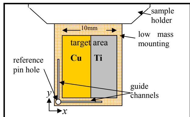
Figure 1: Spoiler target test sample
