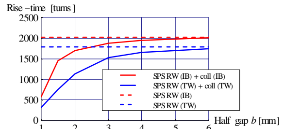
Figure 9: Predicted rise-times (in SPS turns) for 1 batch of 72 bunches ( 1.15 \times 10^{11} p/b). IB stands for Inductive-Bypass (i.e. low-frequency regime), while TW stands for Thick-Wall formula.
