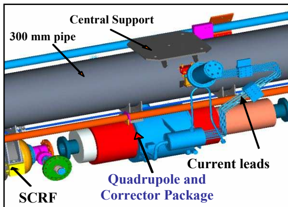
Figure 2: Conceptual layout of a quadrupole-corrector-BPM assembly mounted at the center of a cryomodel.
