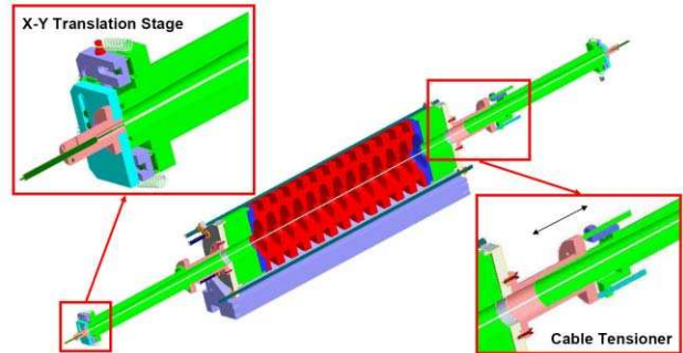
Figure 2: Schematic of the stretched-wire apparatus.
