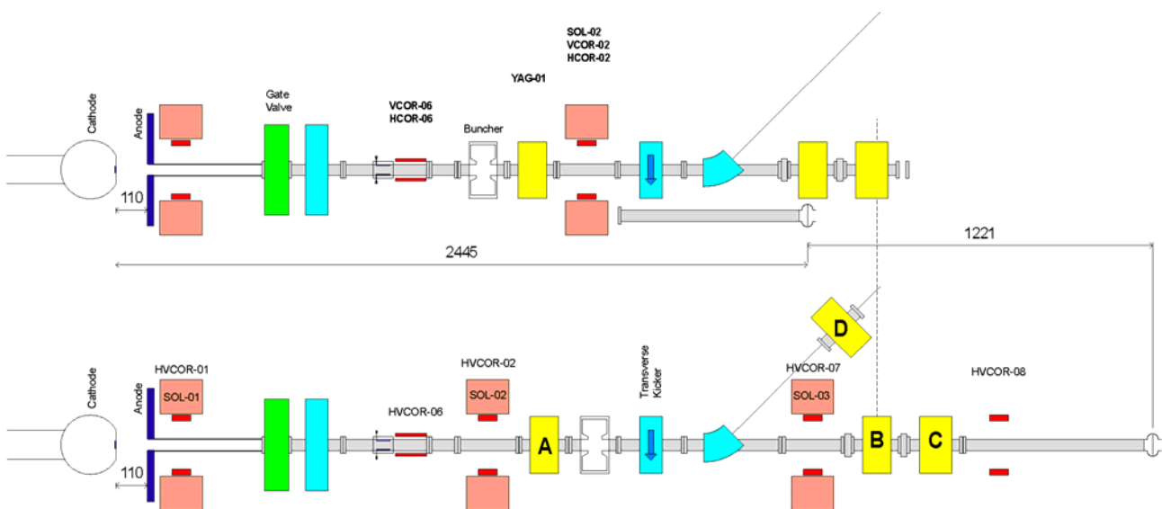
Figure 1: Schematic of the ALICE gun commissioning beamline (top) marking the position where diagnostic sections were removed and the booster linac added. The bottom shows the schematic of the extended ALICE injector up to the entrance of the first cell of the booster.
