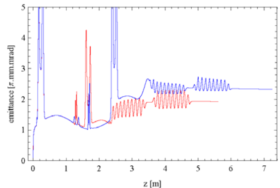
Figure 3: Normalised transverse emittance (rms) along the existing (red) and extended (blue) injector beamlines.
