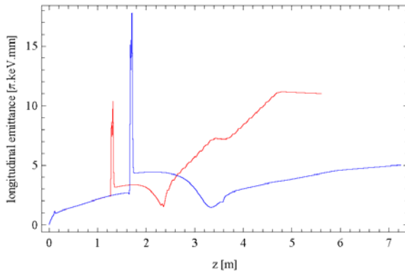
Figure 5: Longitudinal emittance (rms) along the existing (red) and extended (blue) injector beamlines.
