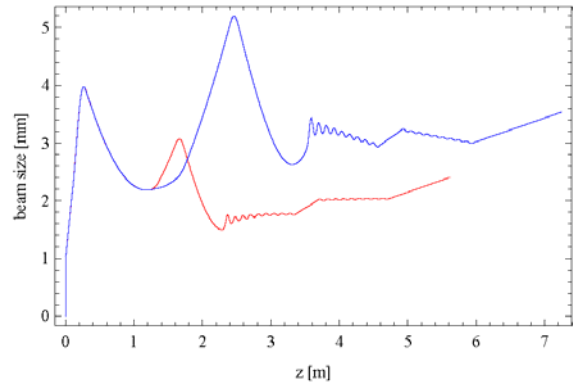
Figure 2: Transverse beam size (rms) along the existing (red) and extended (blue) injector beamlines.
