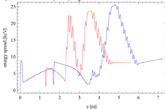
Figure 6: Energy spread (rms) along the existing (red) and extended (blue) injector beamlines.
