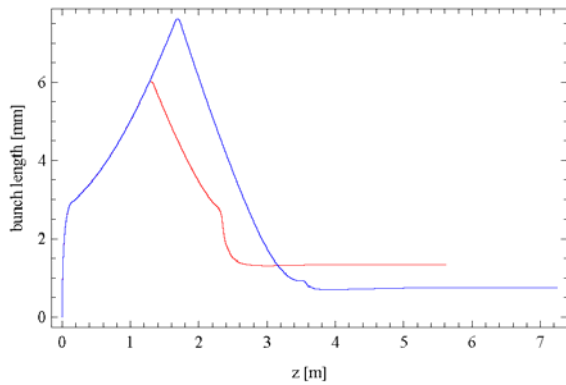
Figure 4: Bunch length (rms) along the existing (red) and extended (blue) injector beamlines.
