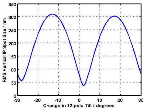
Figure 1: Lucretia model of vertical IP waist size vs. tilt of QF1FF 12-pole component away from measured value of +2 degrees. These results are for a normalised horizontal emittance of 6\mu\text{m} .
