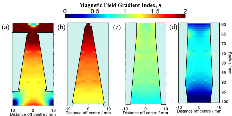
FIGURE 3. Contour plots of n for (a) the standard ISIS pole pieces; (b) ISIS pole pieces with wider radial extent; (c) n = 1 poles; (d) n = 0.75 poles with enlarged shims at the outer radius.
