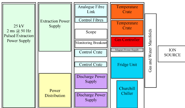
FIGURE 10: The layout ancillary equipment racks for FETS.
