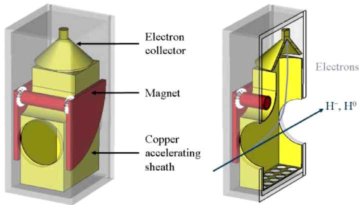
FIGURE 8: The electron collection system for the laser wire profile measurement system.
