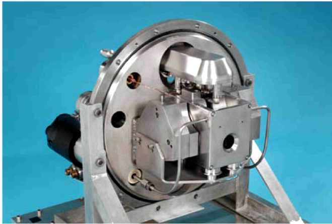
FIGURE 2. The FETS ion source.
