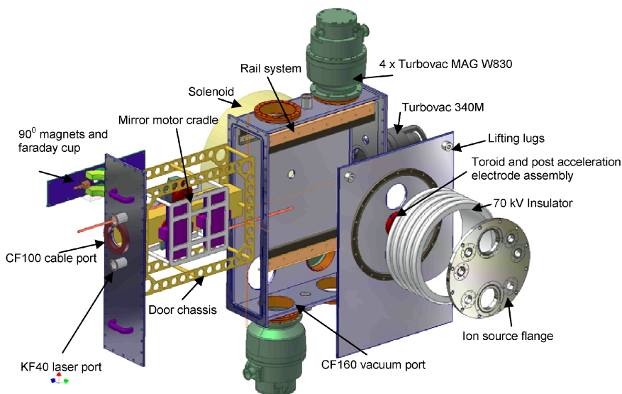
FIGURE 6: Exploded view of the beam profile measurement system inside the ion source vessel.
