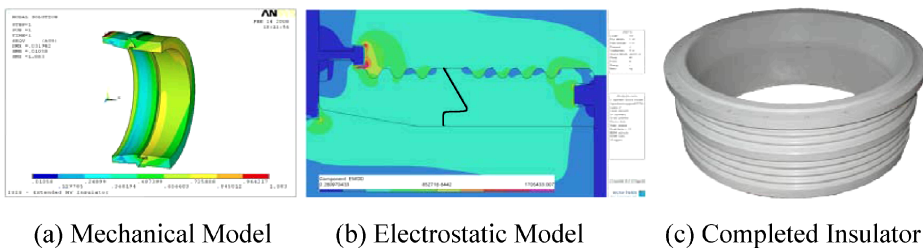
FIGURE 4: The 70 kV insulator.
