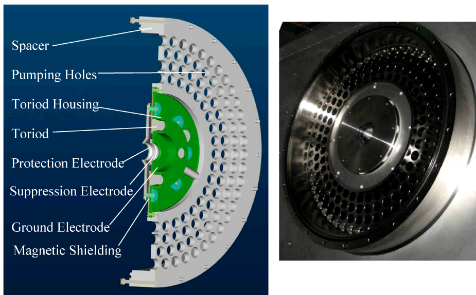
FIGURE 5: The post extraction acceleration electrode assembly.
