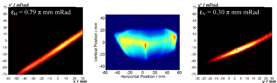
FIGURE 12. Beam emittance and profile from n = 1.0 pole pieces with 17kV extraction voltage.
