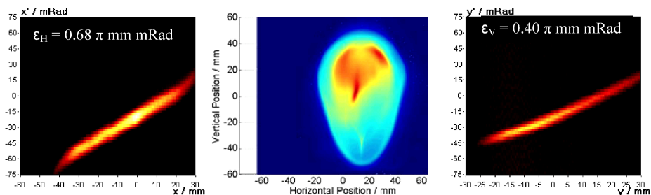
FIGURE 11. Beam emittance and profile from widened ISIS pole pieces with 17kV extraction voltage.
