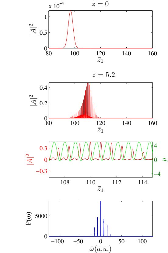
Figure 8: Simulation results for the mode-locked amplifier FEL with a filtered HHG seed. From top: scaled power at the beginning of the interaction, power near to saturation after 26 undulator-chicane modules, detail near to saturation, and the scaled spectral power, for S_e = 4 and an energy modulation of \pm 0.5\%
