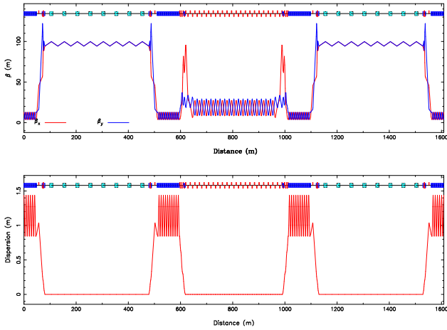
Figure 5: Optical functions of the isosceles ring
