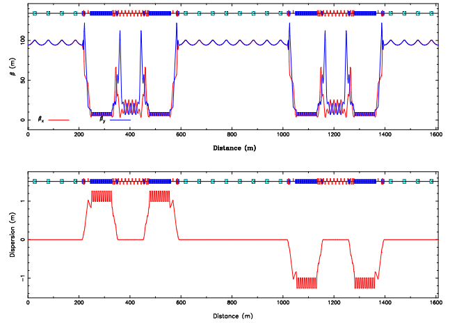
Figure 7: Optical functions of the bow-tie ring
