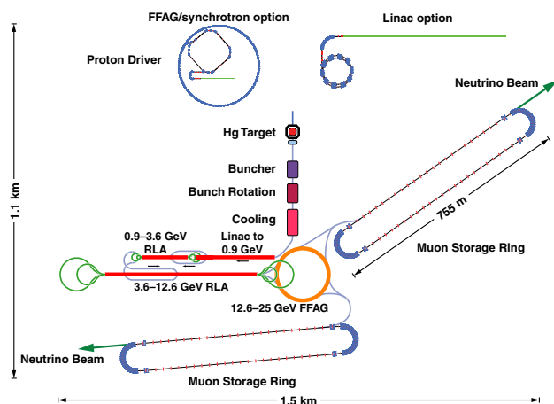
Figure 1: IDS baseline scenario for a Neutrino Factory
