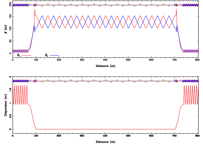
Figure 3: Optical functions for the racetrack ring
