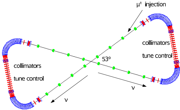
Figure 6: Layout of bow-tie ring
