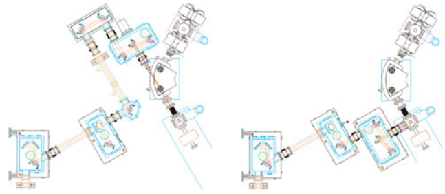
Fig. 9. (Color online) Experimental setup for head-on collision (left) and transverse collision (right).
