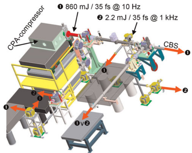
Fig. 4. (Color online) Laser beam lines from the laser front-end system (2.2 mJ @ 1 kHz) and from 4-pass Ti:Sa power amplifier through the CPA compressor to several application stations.
