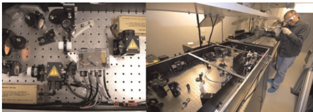
Fig. 2. (Color online) Installation of the regenerative amplifier front end including pulse-picker and kHz compressor.
