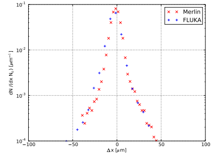
Figure 1: The distribution of change in proton position after scattering through 0.5 m of Copper collimator.
