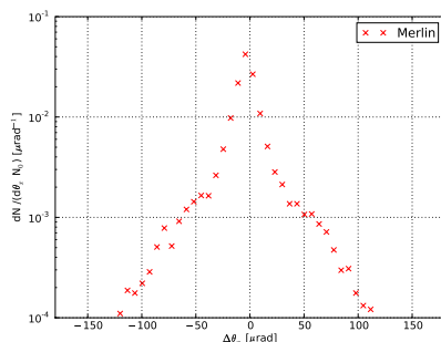
Figure 4: The distribution of change in proton direction after scattering through 1 m of Carbon collimator.
