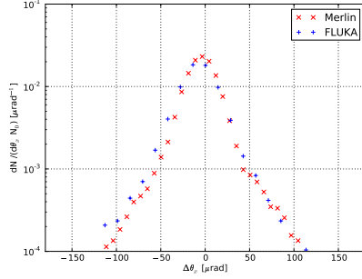
Figure 2: The distribution of change in proton direction after scattering through 0.5 m of Copper collimator.
