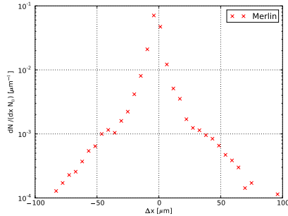
Figure 3: The distribution of change in proton position after scattering through 1 m of Carbon collimator.
