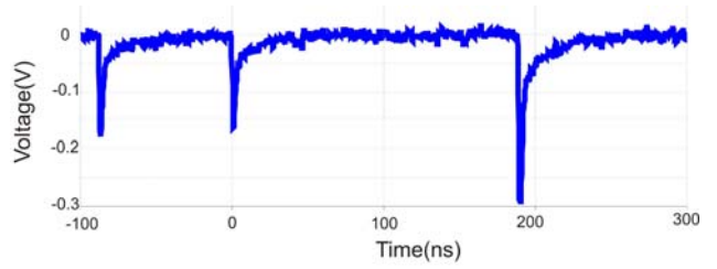
Figure 2: Example of a typical SiPM signal that illustrates the recovery time of a single cell after a signal peak.
