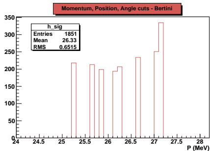
Figure 5: Surface muon production for the ISIS muon target using Bertini model after applying cuts in momentum, position and angle. The simulation used 10^{12} protons on target.
