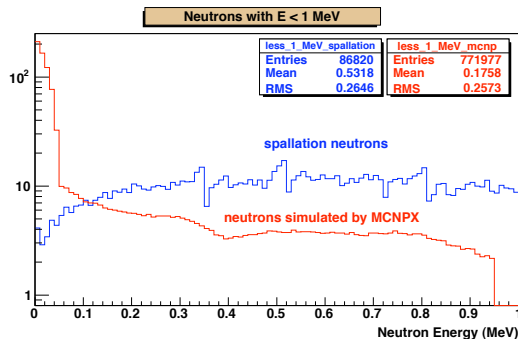
Figure 2: Energy spectra for neutrons with energy less than 1 MeV.
