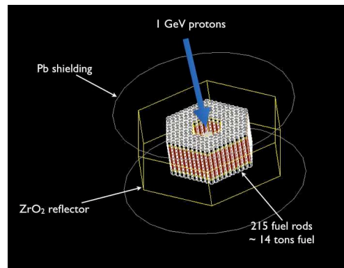
Figure 1: Reactor geometry implementation into GEANT4.
