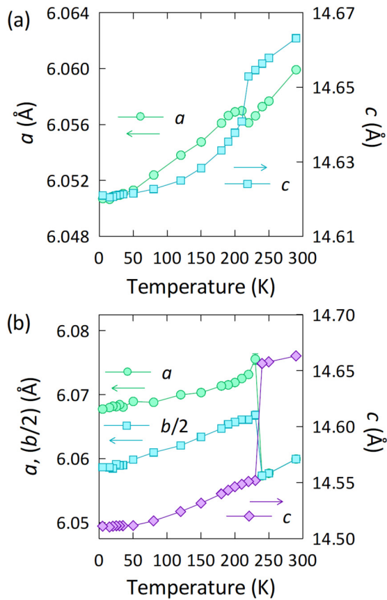
FIG. 5. Variation of lattice parameters with temperature for the (a) P6_3/m and (b) P2_1/m phases. Cell parameters for the P2_1/m phase have been normalized with respect to the parent P6_3/m structure for purposes of comparison. Where not apparent, error bars are smaller than the data points.
