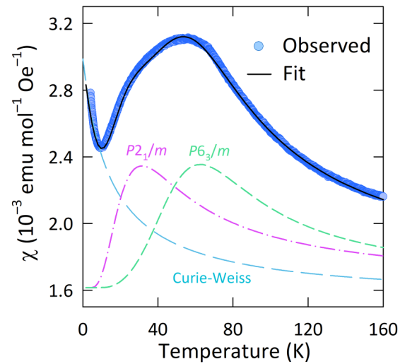
FIG. 8. Zero-field-cooled dc magnetic susceptibility ( \chi ) of Ba_3SrMo_2O_9 under an applied field of H = 100 Oe. Observed data points are given in blue, the fit to the interacting two-dimer model is given by the solid black line, and contributions from the two phases and the Curie-Weiss tail are given by the dashed lines; R^2 = 0.998\ 93 .
