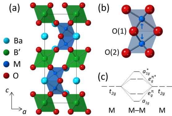
FIG. 1. (a) The crystal structure of Ba_3B'M_2O_9 depicted in the conventional P6_3/mmc space group and projected down [100] . (b) Close-up view of the M_2O_9 dimers: the octahedra are trigonally distorted, displacing each M cation away from the center of their respective octahedron (as indicated by the arrows) and resulting in two crystallographically inequivalent oxygen sites. (c) Partial energy level diagram for strongly interacting M_2O_9 dimers, highlighting the consequent splitting of hybridized t_{2g} orbitals in a trigonally distorted environment.
