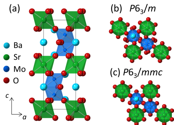
FIG. 2. (a) The 290 K crystal structure of Ba_3SrMo_2O_9 , crystallizing in the P6_3/m space group as viewed down the [100] direction. (b) View of the P6_3/m structure down the [001] direction to highlight the presence of octahedral tilting distortions. (c) Equivalent [001] view of the parent P6_3/mmc structure, showing the lack of any analogous distortions compared to the P6_3/m structure.
