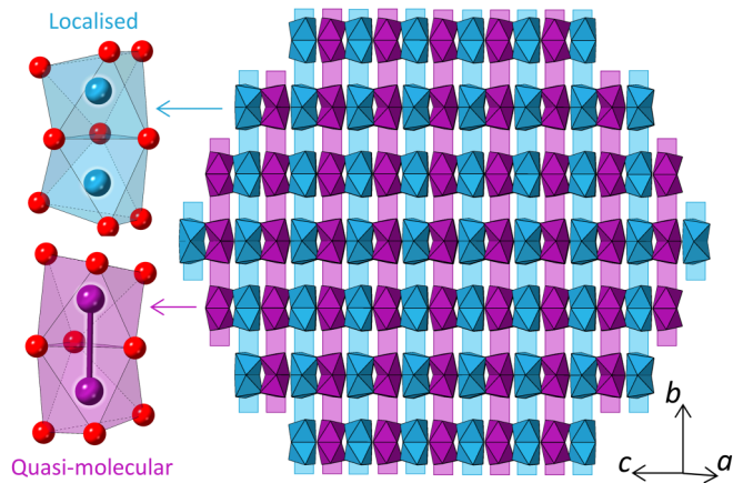
FIG. 9. Expanded view of the P2_1/m phase, showing how stripes of quasimolecular \text{Mo}_2\text{O}_9 clusters alternate with localized \text{Mo}_2\text{O}_9 spin dimers along the monoclinic [001] direction.
