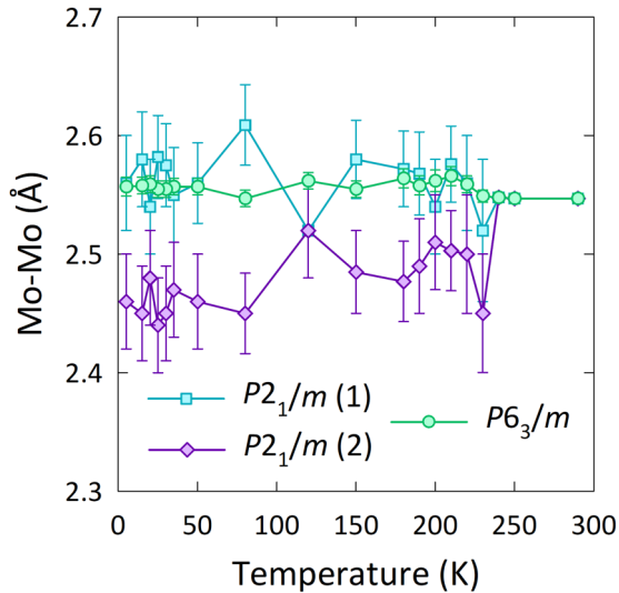
FIG. 7. Variation of Mo–Mo distances with temperature evidencing an orbital-ordering transition at T_{PS} = 230 K.
