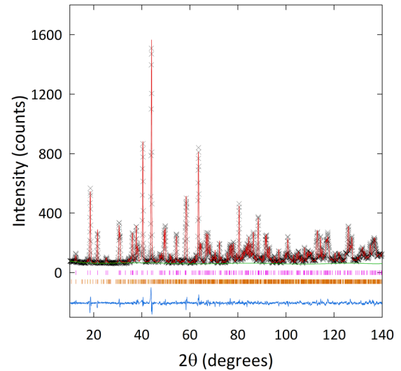
FIG. 4. The Rietveld fit to the two-phase P6_3/m (upper reflections) and P2_1/m (lower reflections) model from D2B NPD data collected at 5 K.
