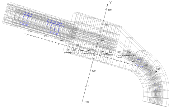
Figure 3: Illustration of how the ring geometry was split in multiple sectors and parts to provide a correct distribution of the electric field. Shown is a region of ELISA with quadrupoles, a 10^\circ parallel plate deflector and part of the 160^\circ bend.
