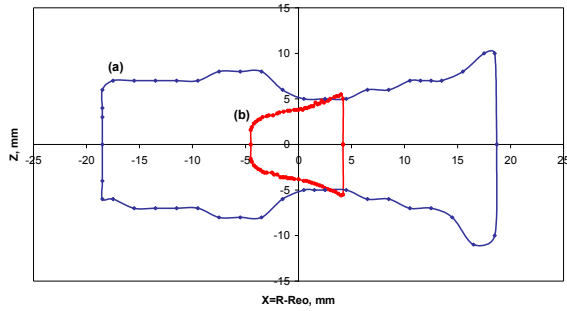
Figure 4: Dynamic aperture of the ring with cylinder deflectors. OPERA-TOSCA simulations: a) Middle of long straight section, azimuth \theta=0^\circ , b) middle of 160^\circ bend, azimuth \theta=90^\circ .
