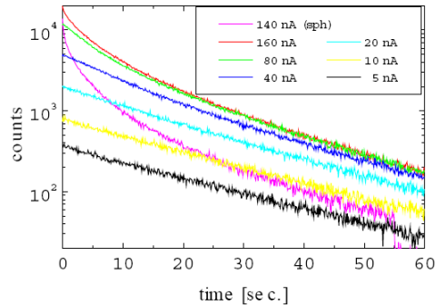
Figure 1: Decay of stored O - beams at 22 keV [3].
