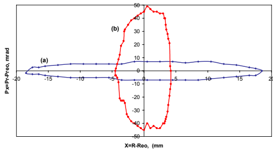
Figure 5: Radial acceptance of the ring with cylinder deflectors. OPERA-TOSCA simulations: a) Middle of long straight section, azimuth \theta=0^\circ , b) middle of 160^\circ bend, azimuth \theta=90^\circ .
