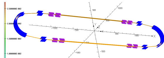
Figure 2: Model of the ELISA ring in OPERA3D. The Dimensions and distances were taken from [12]. All particles were tracked over 700 turns.
