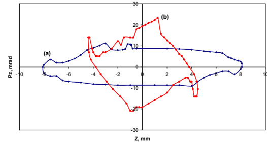
Figure 6: Vertical ring acceptance with cylinder deflectors. OPERA-TOSCA simulations: a) Middle of long straight section, azimuth \theta=0^\circ , b) middle of 160^\circ bend, azimuth \theta=90^\circ .
