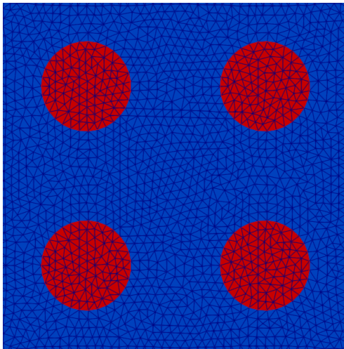
FIG. D.1. Geometry and mesh used for the cookie problem (D.1) with N = 5 .
