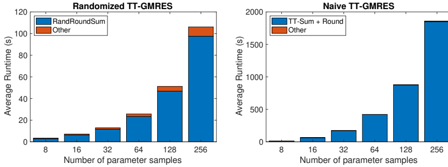
FIG. 4.3. Illustration of the timings using the deterministic and randomized summation and rounding algorithms within the TT -GMRES algorithm to solve problem (D.1).
