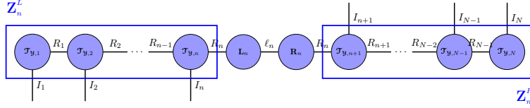
FIG. B.3. Internal left and right factors in the Two-Sided-Randomization (Generalized Nyström) Algorithm 3.3.
