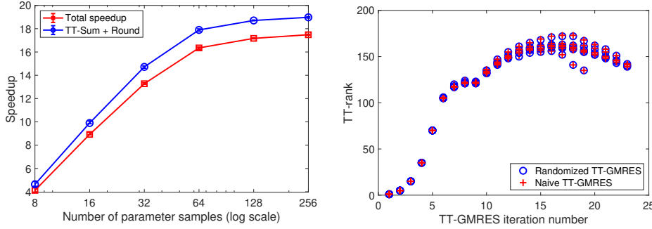
FIG. 4.2. Illustration of the speedups (left) and TT -ranks of the Krylov basis vectors (right) obtained by the deterministic and randomized summation and rounding algorithms within the TT -GMRES algorithm to solve problem (D.1).
