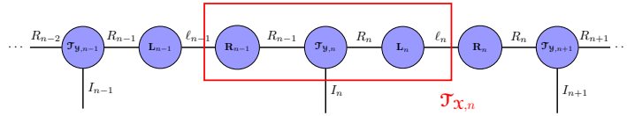
FIG. B.4. Left and right factors distributions within the Two-Sided-Randomization (Generalized Nyström) Algorithm 3.2.
