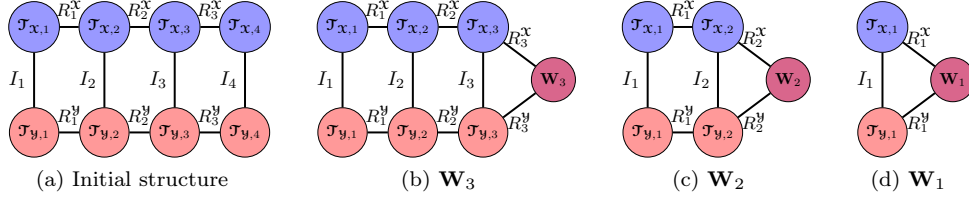
FIG. 2.3. Right-to-Left partial contraction steps for N = 4 .
