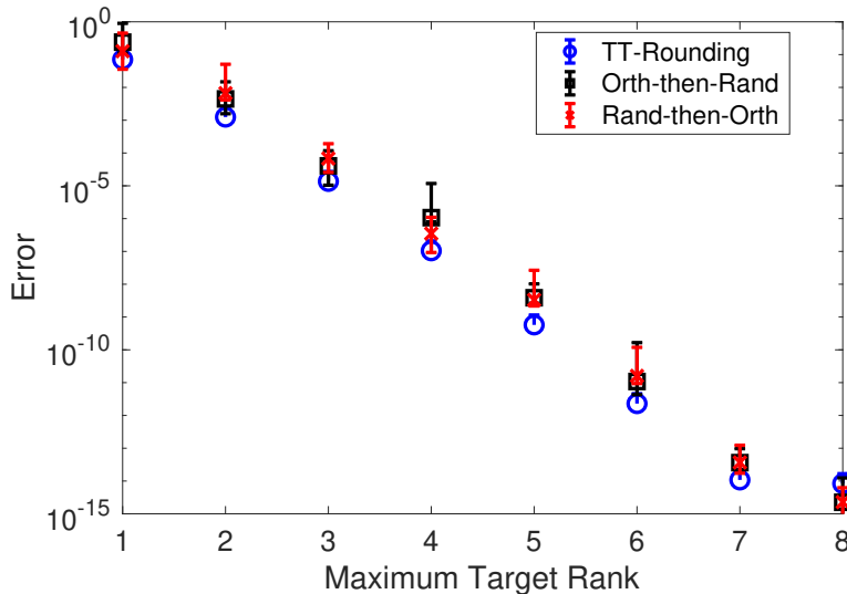
FIG. C.1. Hilbert TT-tensor truncation. Relative Error between a low rank approximation obtained via deterministic or randomized TT-rounding, and a full rank Hilbert TT-tensor.
