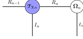
FIG. B.1. Random projection steps for Orthogonalize-then-Randomize Algorithm 3.1.
