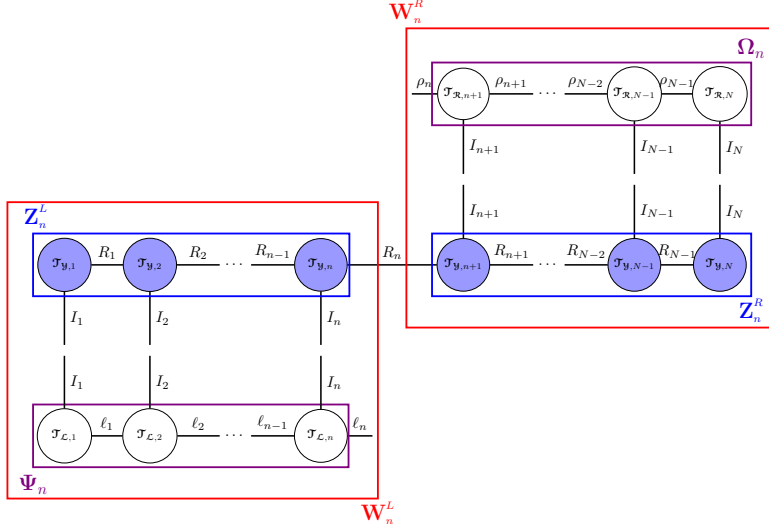
FIG. B.2. Random projections for Two-Sided-Randomization (Generalized Nyström) Algorithm 3.3.
