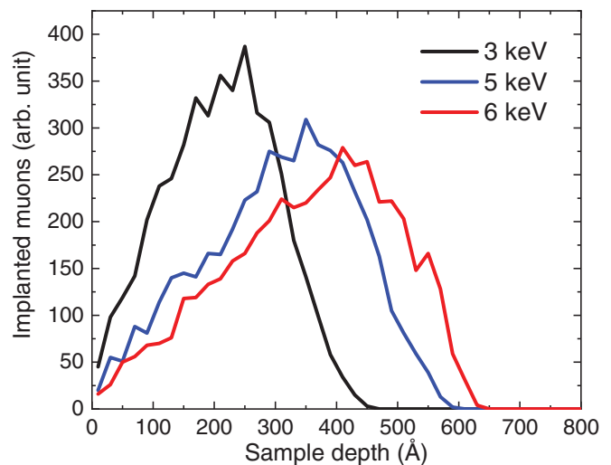
FIG. 8. Muon stopping profiles as a function of sample depth for the implantation energies used in this paper. A depth of 0 Å denotes the sample surface.
