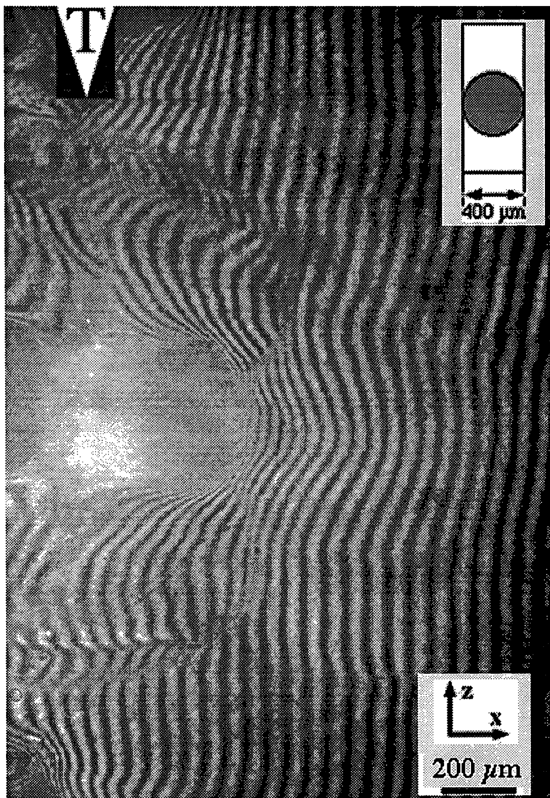
Fig.1 Interferogram taken 3 ns after the peak of the heating pulses using a 100 ps probe pulse. The target was a Al disk (400 μm diameter) on a narrow plastic stripe. The heating irradiance was 5 \cdot 10^{13} \text{ W/cm}^2 on each side of the target. The original target position is shown by a T-wedge.
