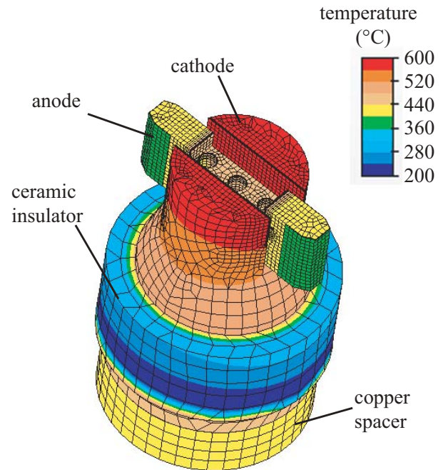
Figure 2: Component temperatures from the steady state model.
