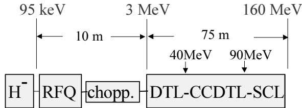
Figure 1: Schematic Linac4 layout.
