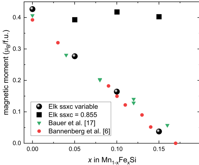
FIG. 7. Ordered magnetic moment of \text{Mn}_{1-x}\text{Fe}_x\text{Si} from experiment (triangles [17], dots [6]) and calculated values applying a fixed (squares) and a variable sssc factor (spheres).
