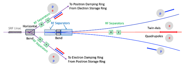
Figure 4: The Linac-Chicane Interface.
