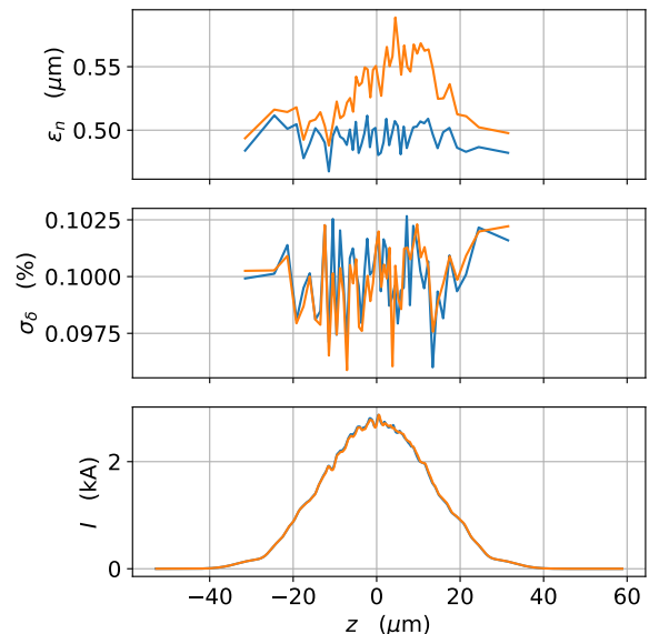
Figure 5: The slice properties of the gaussian bunch before (blue) and after (orange) tracking through FEL-6 of the UK-XFEL spreader. Shown are the (top) horizontal emittance, (middle) energy spread and (bottom) current profile of the bunch.
