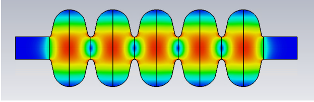
Figure 1: The c650 cavity adapted from the PIP-II HB650 [1] showing the accelerating \pi -mode E-field rendered in CST.
