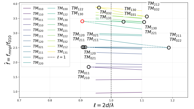
Figure 4: Results of the FM parameter sweep for the 3HC mid-cell. See caption for Fig. 2 for explanation. Shown here are the SHINE 3HC [10] results, although there was no appreciable difference between the EuXFEL and SHINE variants.
