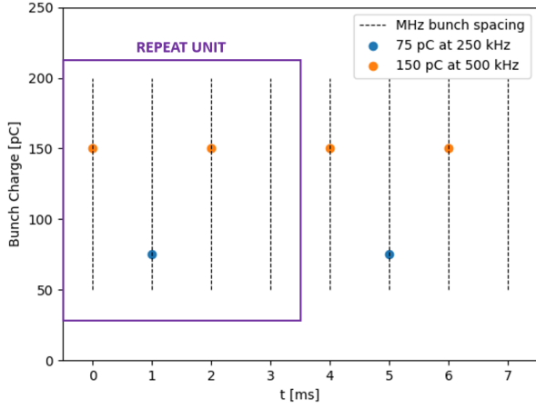
Figure 5: An illustration of the time/charge structure of the composite beam. Each repeat unit is comprised of three bunches and at the the end of a N -bunch simulation a 600 pC bunch is placed, embedded within the 1 MHz rhythm. The horizontal normalised emittance of this 600 pC bunch is tracked and reported in the results (Fig. 6).
