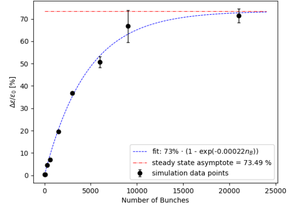
Figure 6: PLACET [6] results for the effect of the LRTW on \epsilon_n as a function of the number of bunches in a simulation. The error bars here display the standard deviation in the \Delta\epsilon/\epsilon_0 judged at the final ten elements in the lattice.
