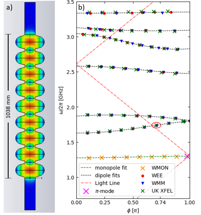
Figure 2: Benchmarking the CST model against known results [4] for the L-band TESLA cavity. a) The TM_{010} \pi -mode E-field distribution. b) The Brillouin diagram for the first monopole and first 6 dipole pass-bands. Results from [4] are depicted in the legend with the prefix 'W'.
