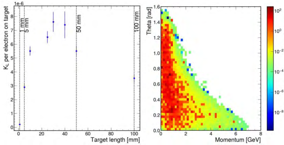
Figure 3.19: Left: number of K_L per electron impinging on target versus target length in mm. Right: distribution of K_L emission angle versus momentum for K_L produced from target
