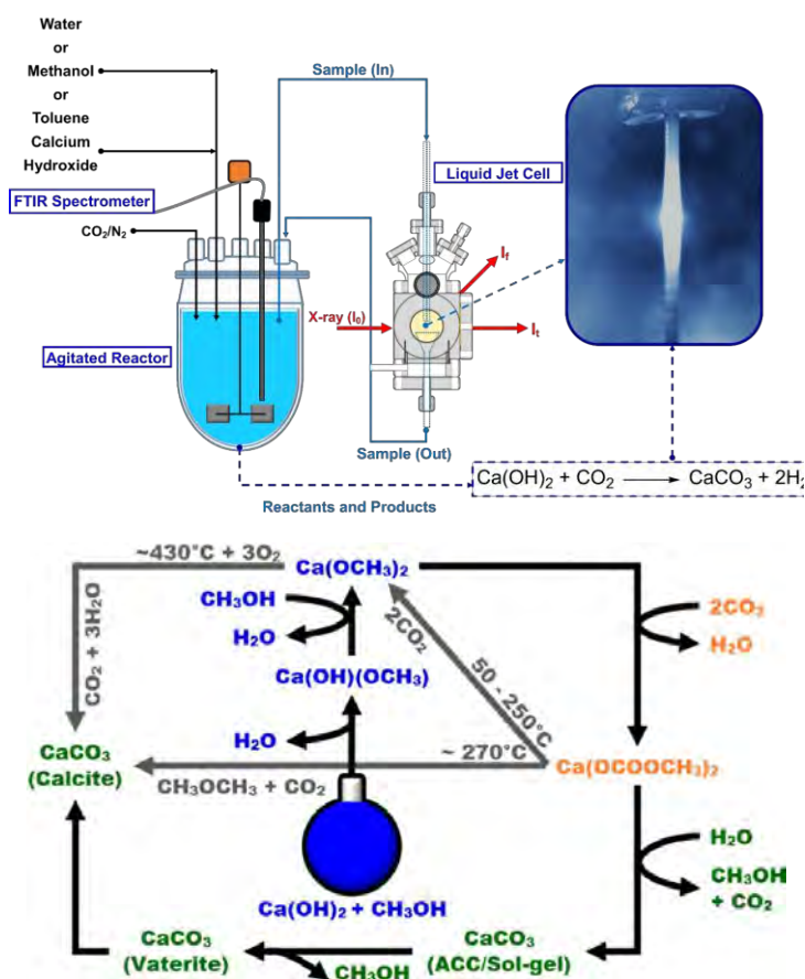
Figure 8.2: (Top) Liquid-jet time-resolved XAS operando probing of the multiphase-multicomponent synthesis of surfactant-stabilised CaCO 3 detergent particles.
