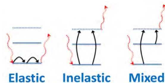
Figure 3.7: Schematic illustration of the components in X-ray scattering
