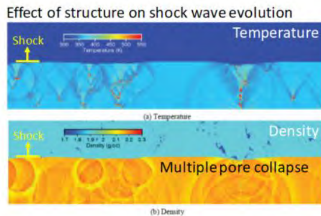
Figure 8.1: Shock propagation in an explosive (from Ref. 15 )
