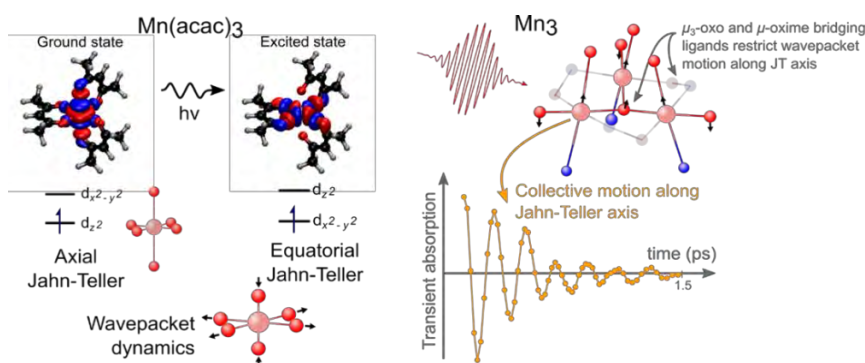
Figure 8.17: Photophysics of Mn^{3+} complexes. The antibonding nature of the e_g orbitals lead to a rapid switch of the JT distortion in the excited state of Mn(acac)_3 (left). In Mn_3 , the strong bonds in the triangle prevent equatorial expansion and the Mn ion (right). 88
