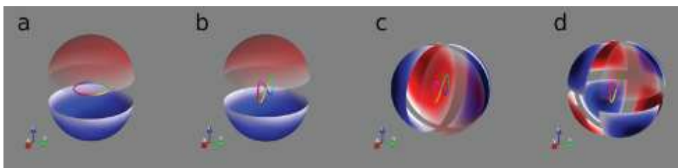
Figure 3.3: Chiral (a, c and d) and achiral (b) detection setups relative to electric fields with circular polarisation (a) and '8' polarisation (b,c,d), demonstrating detection of tensor observables for photoelectron emission from a chiral molecule.
