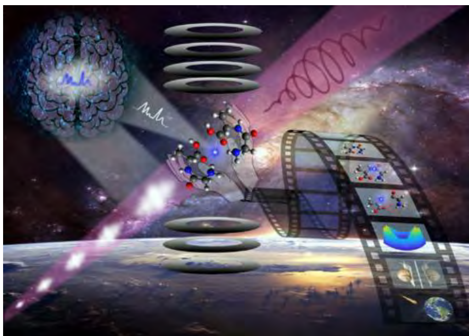
Figure 3.1: An artist’s impression of how optical and XFEL pulses can be combined to reveal and control chiral molecular dynamics, through optimisation of the pulse shape and polarisation
