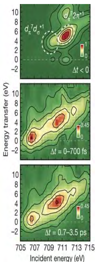
Figure 6.13: Time-resolved RIXS at the Fe L_3 edge sheds light on the ligand exchange dynamics of \text{Fe}(\text{CO})_5 . Measured Fe L_3 -RIXS intensities versus energy transfer and incident photon energy. Top: ground-state \text{Fe}(\text{CO})_5 . Middle and bottom: difference intensities for delay intervals of 0–700 fs and 0.7–3.5 ps, respectively. 9
