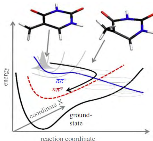
Figure 6.5: Photochemistry of DNA TR-AES and TR-NEXAFS reveals possible relaxation paths a \pi\pi^* state of thymine populated by UV-pulse, to the dark n\pi^* state and to the ground state via conical intersections. 29
