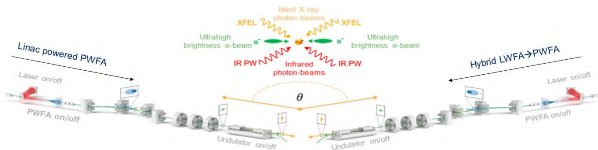
Figure 3.16: Future possibility of colliding extreme beams at a next-generation XFEL facility. Adapted from Ref. [264,265]
