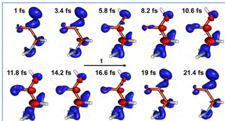
Ultrafast charge motion in suddenly ionised glycine calculated via ADC(2) theory and measured with few femtosecond resolution
