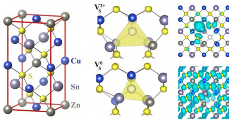
Figure 8.14: (Left) The atomic structure of the Kesterite like \text{Cu}_2\text{ZnSnS}_4 (CZTS) system; (Right) Key defects proposed to be responsible for nonradiative electron-hole recombination and charge density associated with them. 195
