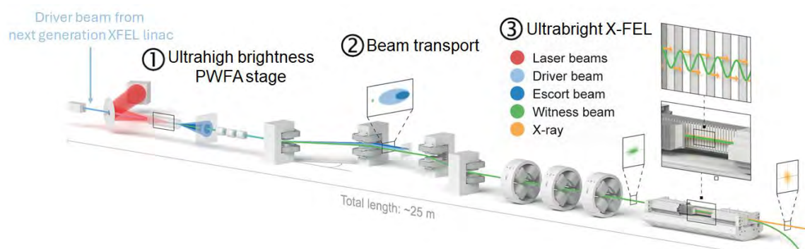
Figure A2.1: PWFA energy and brightness booster stage for a next-generation XFEL
