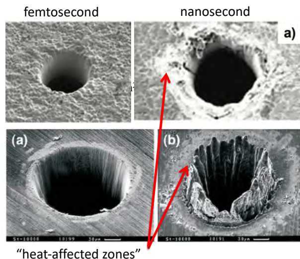
Figure 8.8: Comparisons of the results of fs and ns laser machining, in thin sheets of aluminium 71 and steel 72
