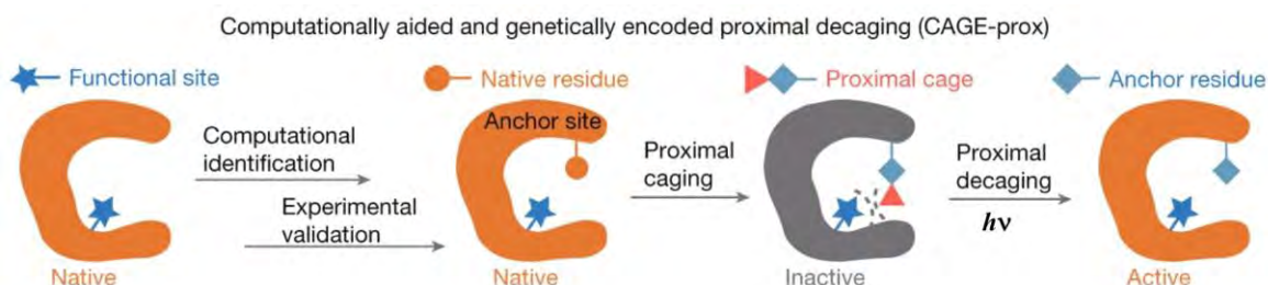
Figure 7.11: Schematic concept of the CAGE-prox strategy
