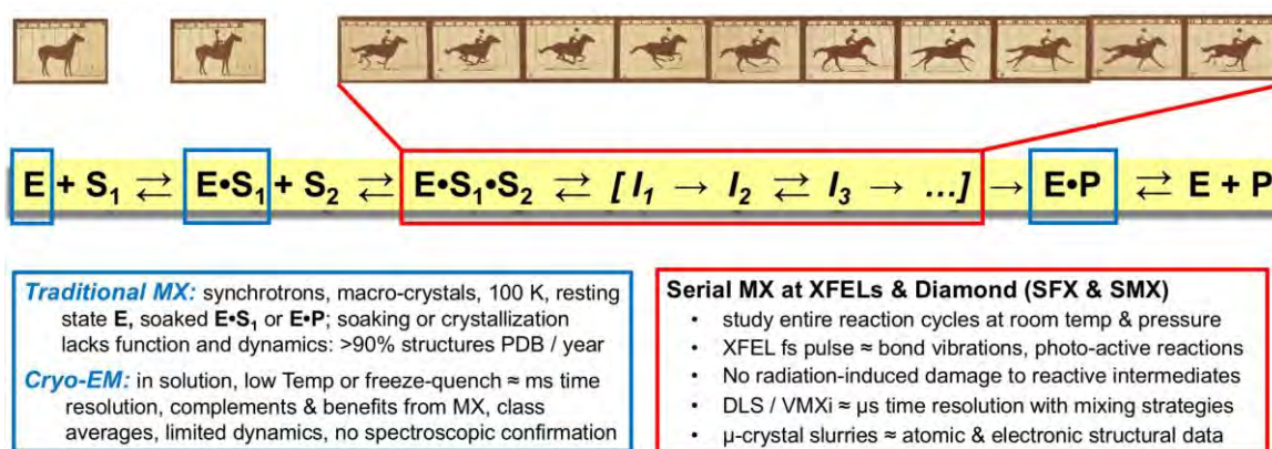
Figure 7.13: Concepts of time-resolved structural biology.
