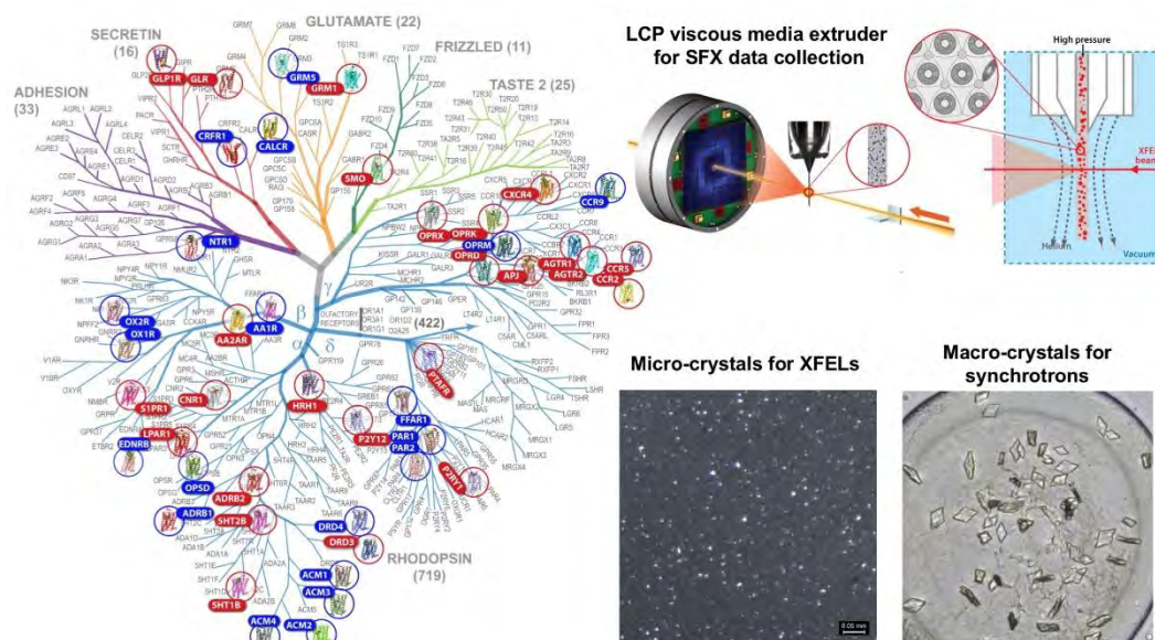
Figure 8.12: (Left) High-resolution crystal structures of GPCRs in 2019 superimposed upon the phylogenomic family tree. (Top right) SFX data collection strategy using an LCP injector at XFELs and microcrystal. (Bottom right) Comparison of micro- and macro-crystals.
