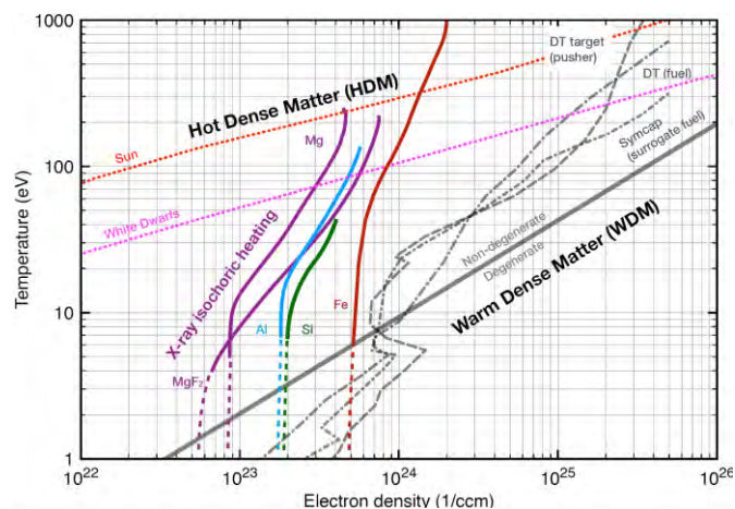
Figure 4.2: Temperatures and densities accessible in the laboratory using x-ray FEL isochoric heating: we can study a broad spectrum of extreme conditions, from planetary cores to stellar interiors. High energy compression drivers will allow us to investigate the unexplored regions at higher densities where quantum effects and correlations persist up to high temperatures.
