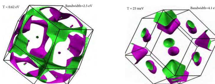
Fermi surface of two spin-down bands at electronic temperatures of 0.025 and 0.62 eV plotted inside the first BZ of the BCC structure. Increasing the electronic temperature reduces the bandwidth and localises the band near the Fermi surface. Figure reproduced from ref. [4].
