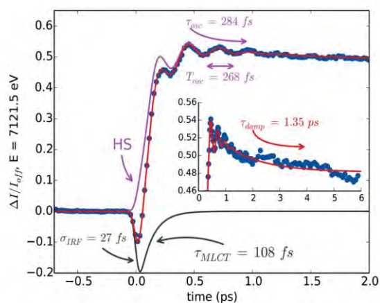
Figure 6.12: Fit to the femtosecond transient XANES of [\text{Fe}(\text{bpy})_3]^{2+} measured at 7121.5 eV, showing the contribution of the MLCT and of the oscillating high spin state. 14
