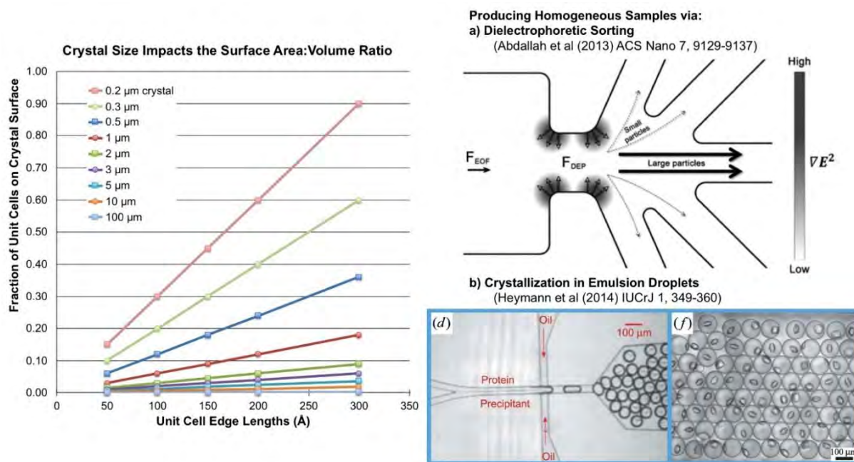
Figure 8.4: (Left) The fraction of unit cells on the surface of a crystal increases with smaller crystal size. (Right) Some methods to produce uniform slurries of microcrystal that are suitable for time-resolved SFX studies.
