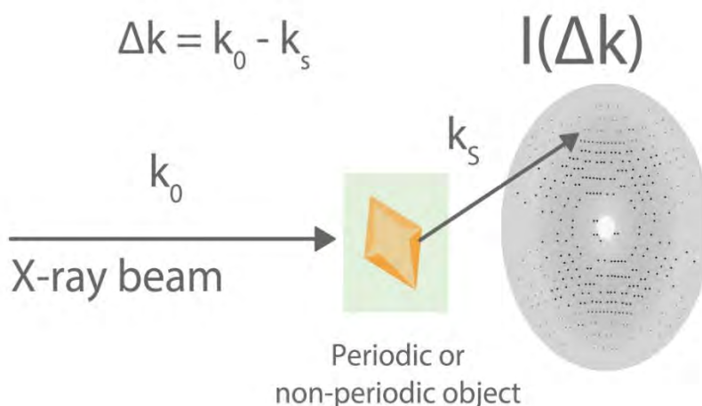
Figure 2.2: X-ray scattering, from either a crystal or a non-periodic object, leads to a distinct diffraction pattern from which the structure can be reconstructed. Through the high temporal resolution now available at XFELs, structural dynamics can be followed in full detail.
