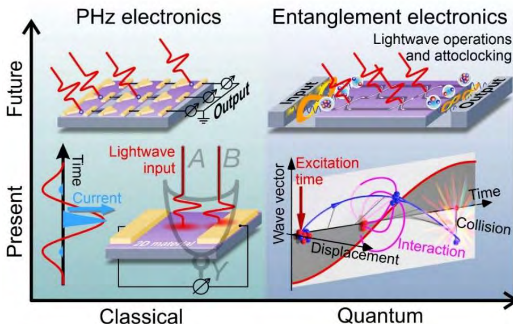
Figure 5.10: The emerging field of lightwave electronics
