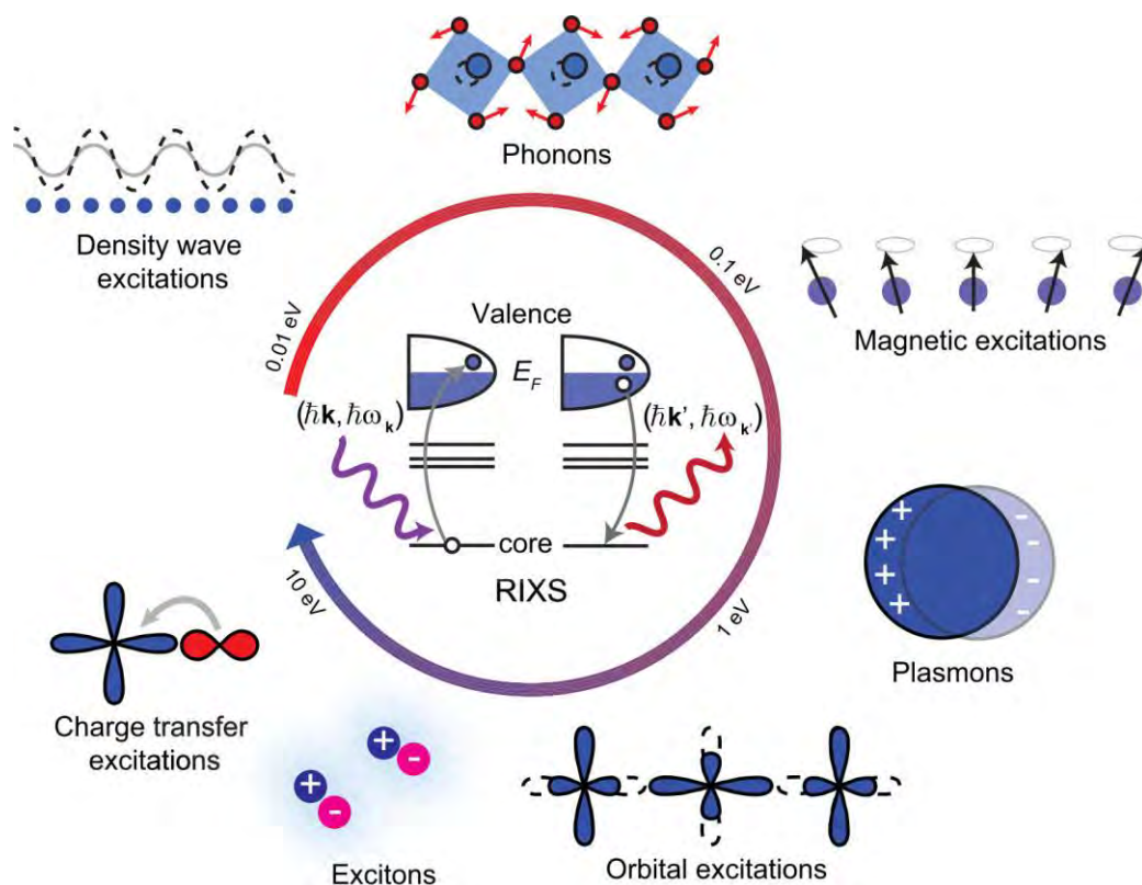
Figure 5.1: The resonant scattering process, shown in the centre, involves the resonant absorption of an X-ray photon, creating an intermediate state with a core hole and a valence excitation, before the hole is filled via the emission of another X-ray photon. Measuring the momentum-change of the scattering, in a so-called resonant diffraction experiment, can probe electronic order parameters such as magnetic order. By measuring the energy and momentum change of the X rays in a resonant inelastic X-ray scattering (RIXS) experiment, one can infer the properties of the excitations created in the material. The many different types of excitation that RIXS can probe are shown around the outside. 6
