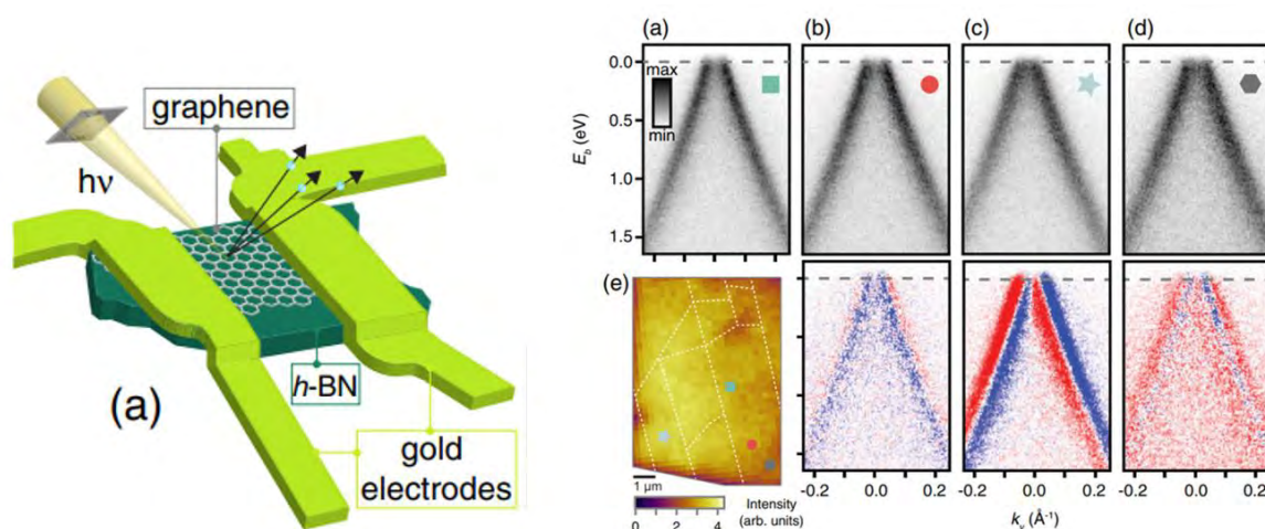
Left: Graphene on h -BN with gold source-drain electrodes to inject ‘transport current’ at THz frequencies. Right: Intensity of the Dirac cone spectra taken in different locations of the device, as given by the corresponding markers in (e) [reproduced with permission from 3].
