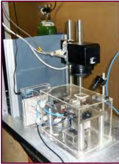
Figure 8.7: Example additive manufacturing platform that can fit within the experimental facilities, the 'shoe box' laser additive manufacturing system which was used by Bidare et al. in monitoring the process using high-speed imaging
