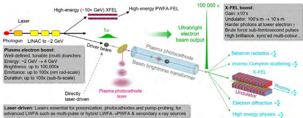
Figure A2.2: Schematic diagram of the capabilities enabled by combining XFEL beamlines and plasma accelerators
