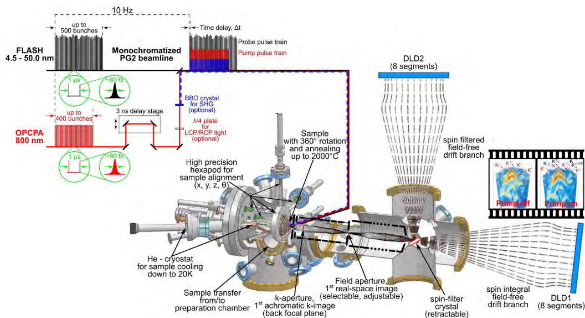
Figure 5.9: Simplified overview of the FLASH pulse structure, the PG2 beamline with synchronised pump laser (top left) and the experimental setup (middle) used to perform time-resolved momentum microscopy and acquire volumetric band-mapping movies (right inset) by means of a multidimensional recording scheme. 78
