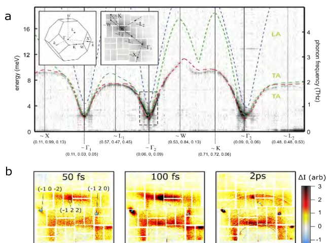
Figure 5.4: Time-resolved diffuse X-ray scattering. a Fourier Transform inelastic X-ray scattering is now able to measure phonon dynamics in Ge throughout the entire Brillouin Zone with sub meV energy resolution. 40 b Time-resolved diffuse scattering changes during a structural phase transition in VO 2 , showing that lattice disorder dominates at early timescales. 41
