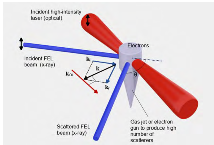
Figure 3.13: Schematic of the setup for the proposed experiment to detect Unruh radiation. The black arrows indicate the polarisation direction of the optical laser and XFEL beams (both vertical in the figure).
