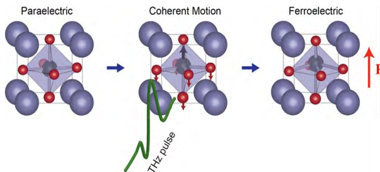
Figure 6.9: A single-cycle THz electric field which moves all the ions it encounters toward their positions in a new ferroelectric crystalline phase. In \text{STO} , the initial high-symmetry configuration around each \text{Ti}^{4+} ion has no dipole moment and the crystal is paraelectric. The incident field drives the “soft” lattice vibrational mode, moving the ions along the directions indicated into a lower-symmetry geometry with a dipole moment. 52 This ion movement can be probed directly with X-rays.
