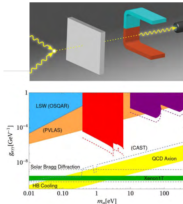
Figure 3.12: Top: Probing production of dark matter with the coherent interaction of two laser beams (from Physics 13 , s59, 2020; APS/Alan Stonebraker). Bottom: Exclusion plot for axion parameter space. We included the mass interval which can be probed when considering frequency doubled beams. The dashed red line indicates the improvement for a 15 kJ laser. The purple region on the right shows the projected bounds for the collision of an optical and an XFEL 239 .
