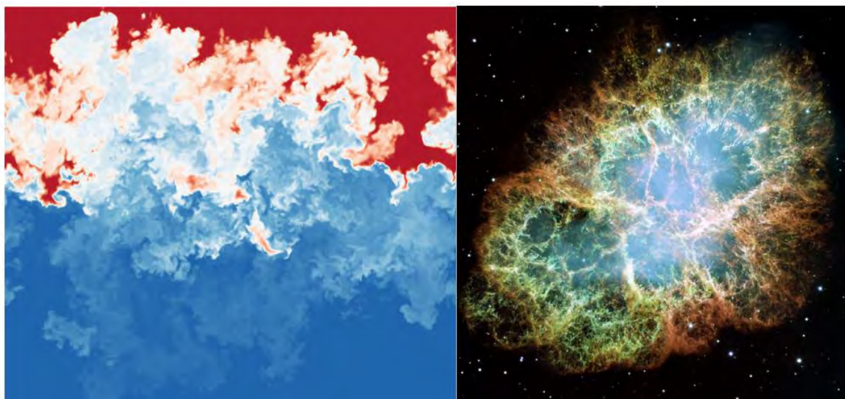
Left: Simulation of a turbulent fluid mixing during shock-compression of an imperfect interface from [1]. Right: A composite Hubble Space Telescope image of the Crab Nebula. © NASA
