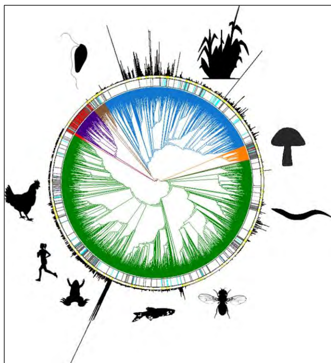
Figure reproduced from H.A. Lewin et al. Proc. Natl. Acad. Sci. USA 115 , 4325-4333. Copyright (2018) National Academy of Sciences DOI: 10.1073/pnas.1720115115
