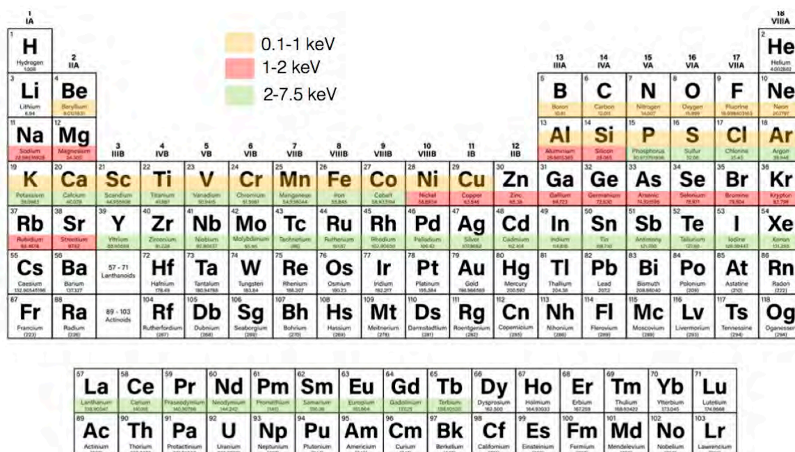
Figure 6.1: The Periodic Table showing energy ranges of X-rays for key absorption edges
