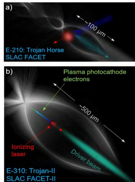
Figure 3.14: The "Trojan Horse" experiment scheme Adapted from Ref. [263]
