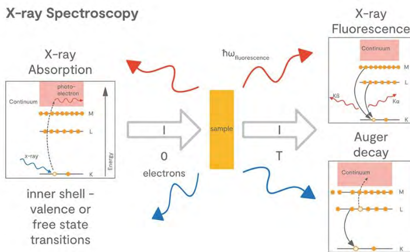
Figure 2.3: X-ray spectroscopy is sensitive to the electronic states, their energies, populations, symmetries and interactions. Utilising the specificity afforded by atomic X-ray absorption edges, time-resolved X-ray spectroscopy can give access to the local evolution of states in space and time
