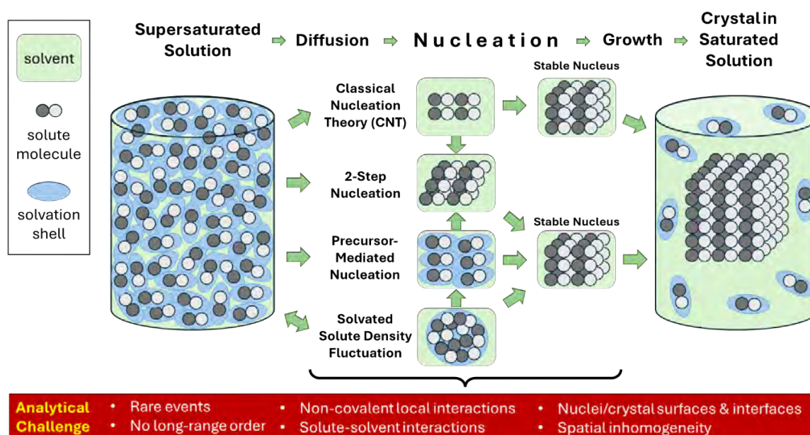
Figure 8.3: Classical nucleation theory and alternative mechanistic pathways in crystallisation, highlighting the experimental challenges in nucleation science
