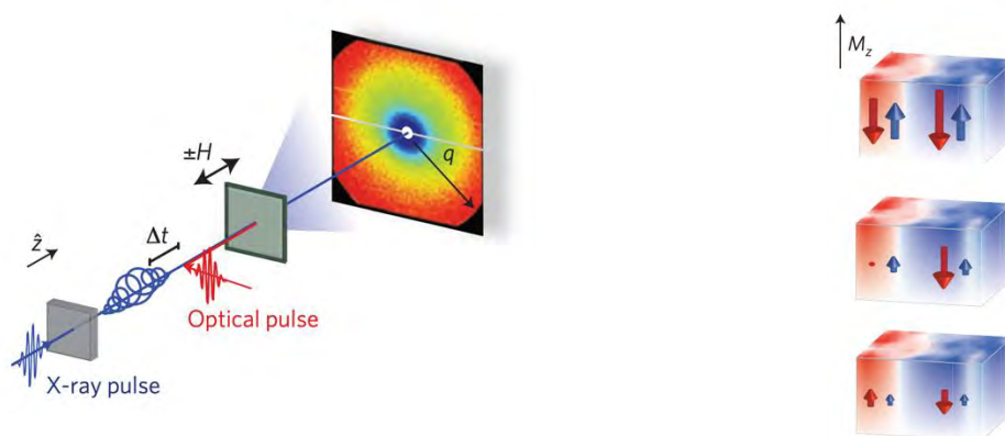
Figure 5.2: Magnetic domain dynamics. Left the experimental setup for magnetic diffraction from domains. Right an illustration of the evolution of iron and gadolinium moments out of equilibrium. 8
