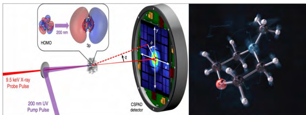
Figure 3.5: (Left) Schematic of the first experiment to directly observe an excited electronic state in a molecule using ultrafast X-ray scattering. (Right) A recent experiment has been able to accurately measure bond distances in an excited molecule undergoing harmonic vibration. 96
