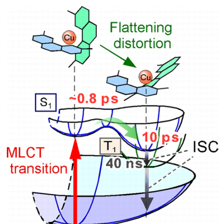
Figure 6.7: Light-triggered distortion in a Cu-complex. Ultrafast nuclear, spin and electronic, dynamics are convolved. 37
