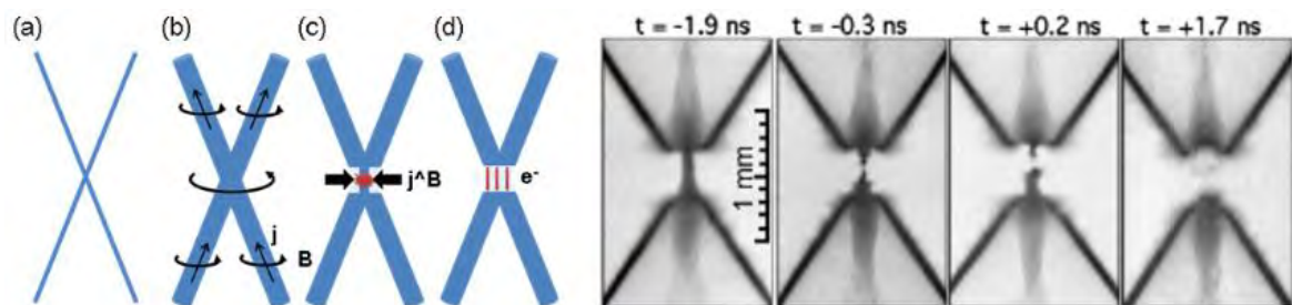
Left: Implosion of an X-pinch showing initial expansion of the wires into dense plasmas (b), m=0 development at the crossing point and emission of X-ray burst (c), break up of column and micro-diode formation (d). Right: Radiographs of different X-pinch experiments show the evolution of the X-pinch at the neck region driven by the m=0 instability occurs on the ns – sub ns timescale.
