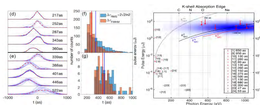
Figure 3.8: Results from LCLS showing (left) the measured 200 – 500 attosecond pulses in the SXR region, and (right) the comparison to HHG attosecond sources 118
