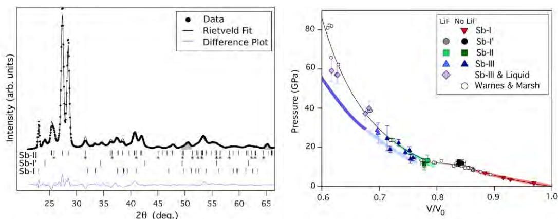
Figure 4.1: Examples of synchrotron quality diffraction data from an ordered incommensurate host-guest structure (left) and complex phase evolution with pressure (right) in shock compressed antimony 7
