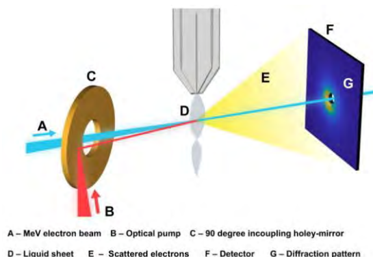
Figure A1.4: Schematic representation of the liquid-phase MeV UED experimental setup
