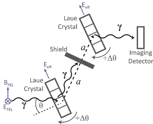
Figure 3.10: Diagram of the setup in the European XFEL experiment; the X-ray beam propagates from left to right. Here, B_{FEL} is the magnetic field in the XFEL beam, and E_{eff} is the crystalline electric field. Axion production and photon regeneration are expected to take place via the Primakoff effect within a pair of monolithic crystals, Ge(220) in Laue geometry. The shield is a 1 mm thick titanium sheet. The polarisation of the X-ray beam maximises the value of B_{FEL} \cdot E_{eff} and thus the probability of axion production.
