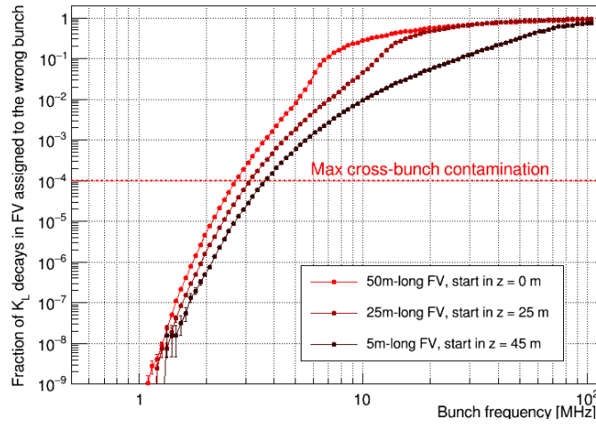
Figure 3.21: Fraction of K_L decays in fiducial volume assigned to the wrong bunch, as a function of bunch frequency in MHz, for three different definitions of fiducial volume. The maximum acceptable cross-bunch contamination is indicated by the red line.
