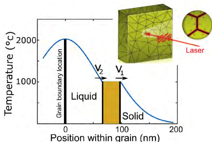
Figure 8.9: Model of the behaviour seen in laser pump, XFEL X-ray probe measurements of the spatial of melting of a 300 nm gold thin film near a grain boundary 73
