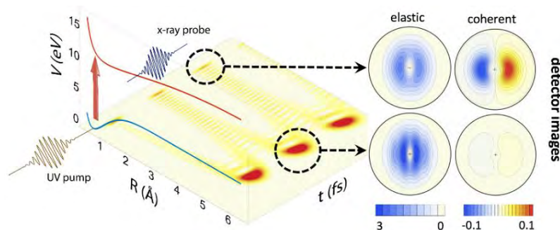
Figure 3.6: Coherent mixed scattering appears as a consequence of coherent electron dynamics and may help characterise complex dynamic processes in matter. On the left-hand side, an optically pumped wavepacket is shown, with the X-ray scattering detector images showing elastic and coherent mixed scattering shown on the right 100
