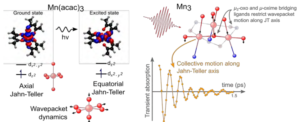
Figure 6.10: Photophysics of \text{Mn}^{3+} complexes. The antibonding nature of the e_g orbitals lead to a rapid switch of the JT distortion in the excited state of \text{Mn}(\text{acac})_3 (left). In \text{Mn}_3 , the strong bonds in the triangle prevent equatorial expansion and the Mn ion (right). 87
