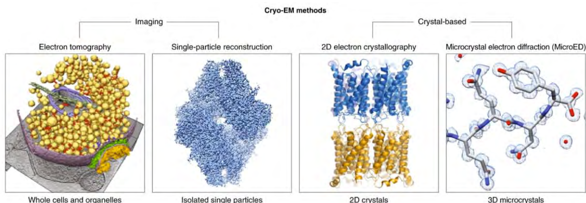
Figure A1.1: The diverse imaging-based and diffraction-based techniques used in cryo-EM can provide structural information from a wide range of samples
