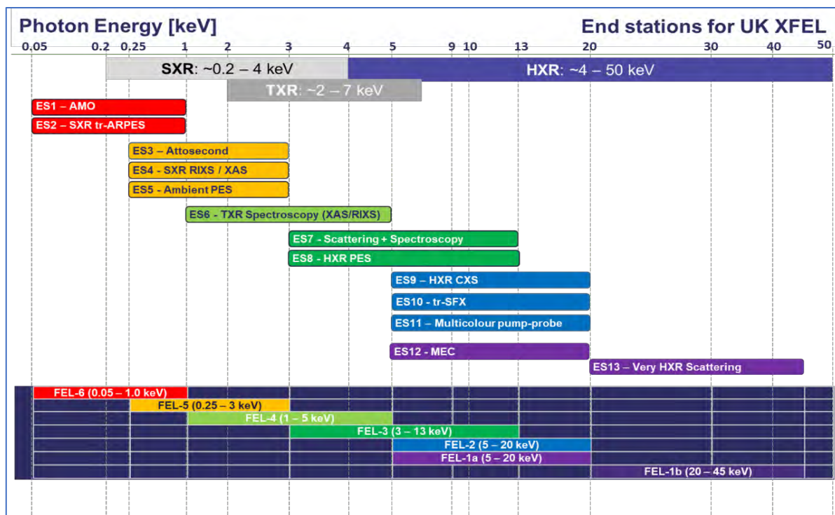
Figure 9.2: Overview of end-stations from the Conceptual Design process, with mapping to science and technology areas
