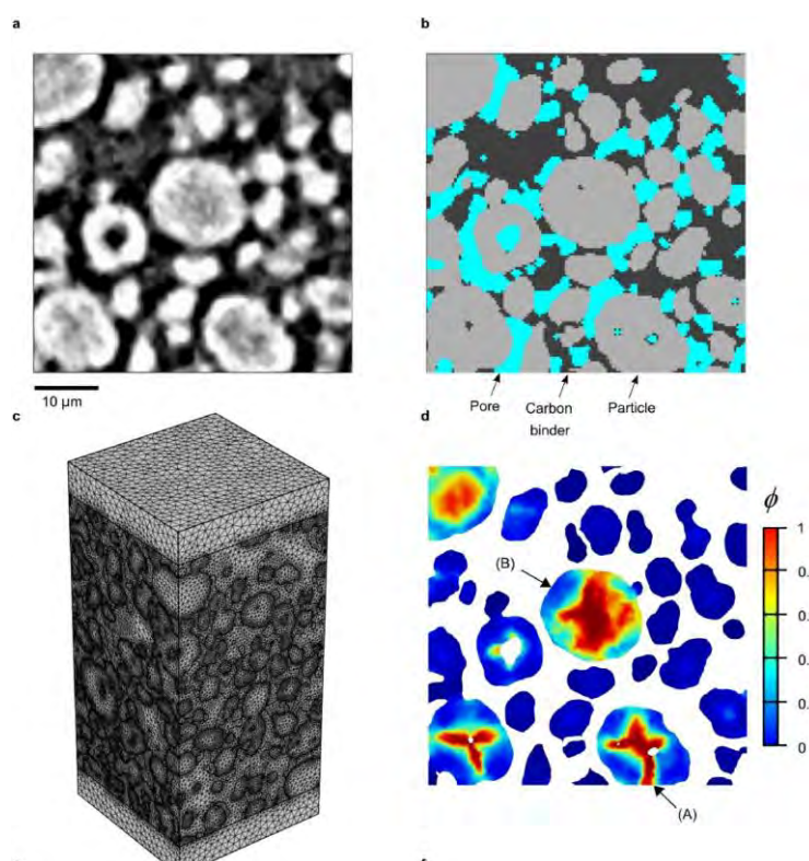
Figure 8.16: X-ray tomography, segmentation, meshing and simulation of an electrode. a) Tomogram of cropped three-phase image, b) segmentation of CT image, c) computational mesh of segmented 3D volume, d) example of model output showing fracture at a slice equivalent to a) and b).
