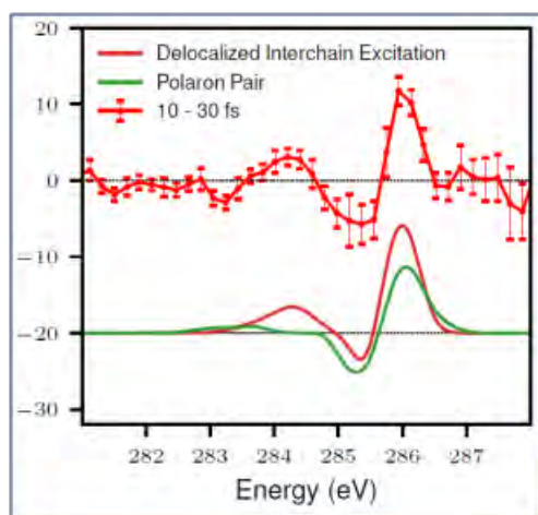
Figure 8.15: Experimental time-resolved XAS of P3HT \Delta A (mOD) at the carbon K edge. 209
