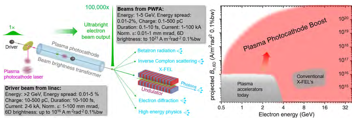
Figure 3.15: Layout for a plasma photocathode based PWFA (left) and the potential beam brightness boost (right)
