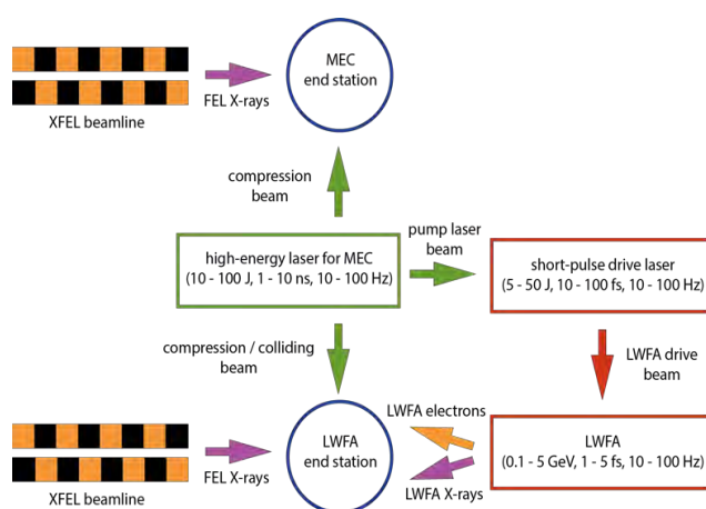
Figure 4.3: Schematic diagram illustrating how auxiliary lasers at an XFEL could drive a LWFA
