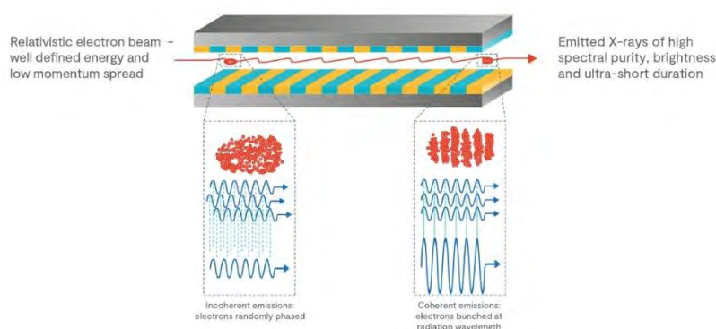
Figure 2.1: Principle of operation of a SASE X-ray free electron laser
