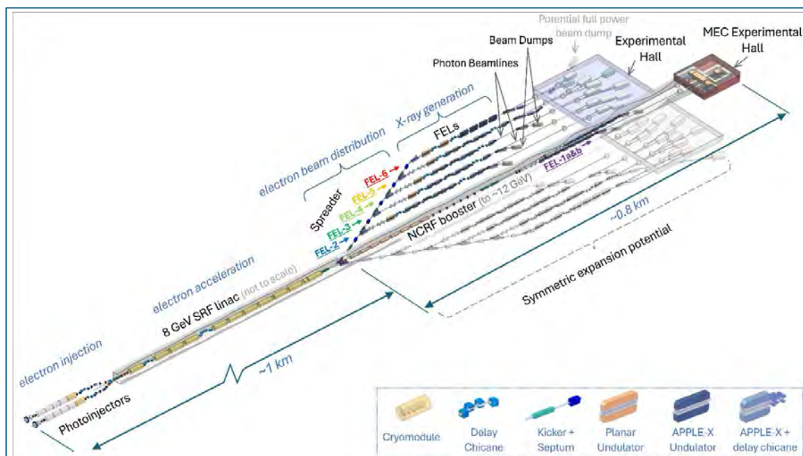
Figure 1.1: An outline of the conceptual design for a next-generation XFEL that would provide a unique combination of capabilities, able to deliver the opportunities discussed in this Case
