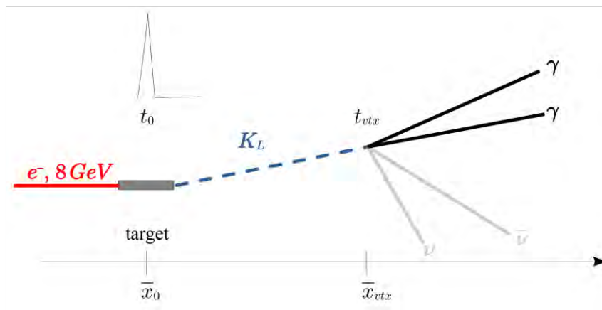
Figure 3.17: Conceptual illustration of the time-of-flight method
