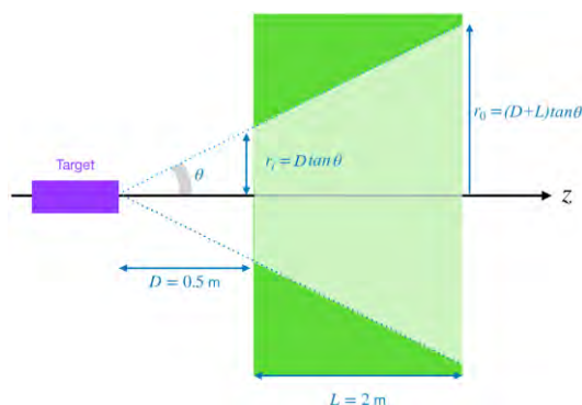
Figure 3.22: Conceptual illustration of a collimator device
