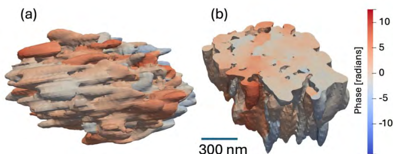
(a) External surface of a 1600 nm sized \text{Li}_3\text{Ti}_2(\text{PO}_4)_3 crystal measured by BCDI on a 110 Bragg peak. The cigar shaped domains are oriented along the hexagonal crystal's c-axis, horizontally on the page. (b) Cross section perpendicular to the c-axis showing a network of phase domains. Ion diffusion is expected to take place along the domain boundaries.
