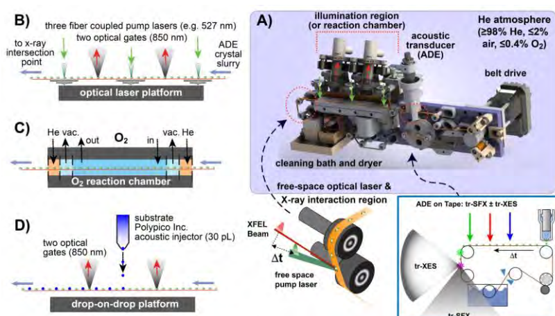
Figure 7.9: Acoustic tape drive system for pump-probe time-resolved SFX and XES measurements of PS-II (A & B) and options for O 2 dependent reactions (C) or drop-on-drop ligand additions (D). See also Fuller et al. (2017) Nature Methods 14 , 443-449.
