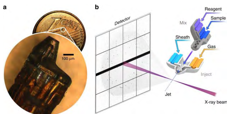
Figure 7.14: A microfluidic device for time-resolved SFX. a) Through micro-3D-printing Knoška et al fabricate microfluidic devices of a few 100 µm in size. Magnified view of a nozzle placed on a 1 cent coin for scale reference. b) This technique can realise integrated nozzle assemblies to jet protein crystal suspension into the X-ray interaction region for diffractive imaging.
