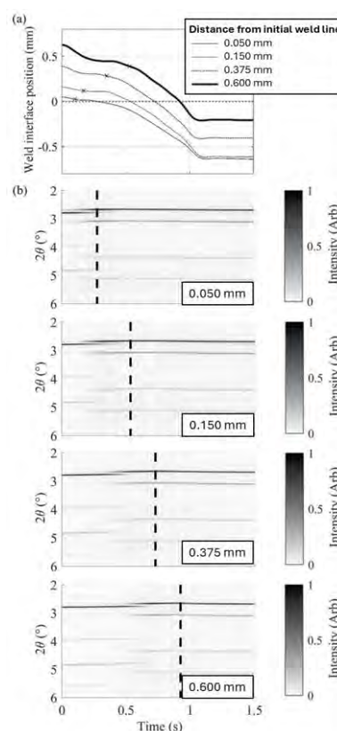
Figure 8.5: In situ high speed synchrotron X-ray diffraction analysis of phase evolution during inertia friction welding of high-carbon steel
