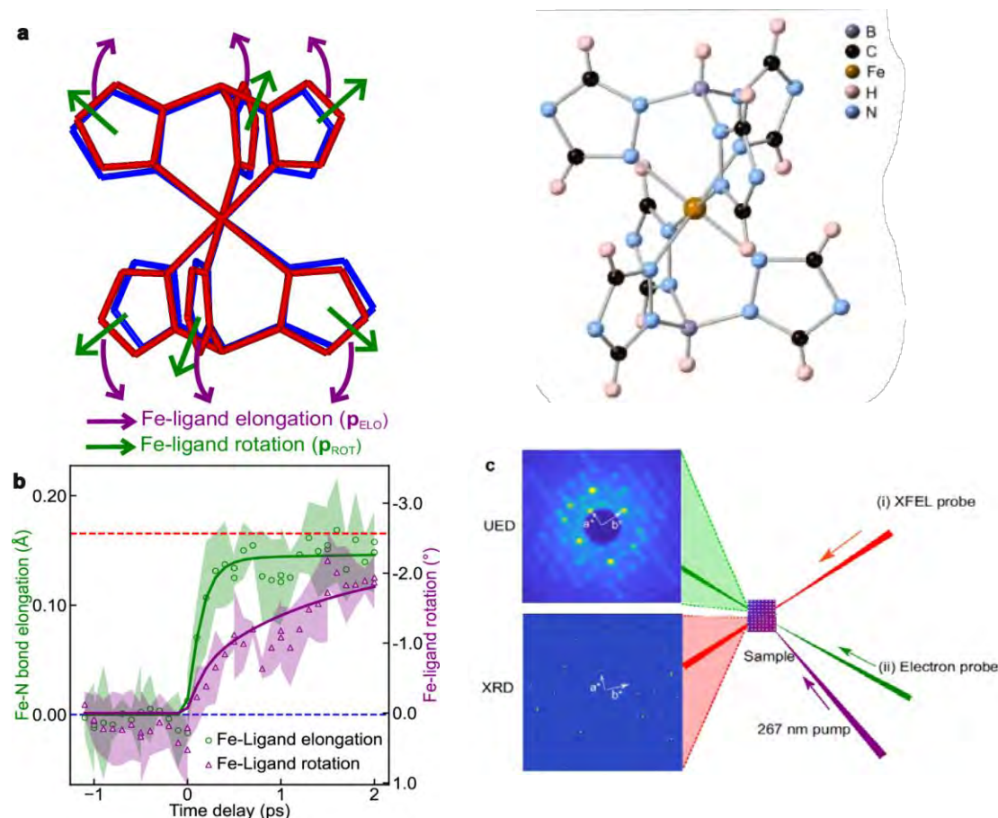
Figure 6.11: Capturing ultrafast molecular motions and lattice dynamics in spin crossover film using femtosecond diffraction methods
