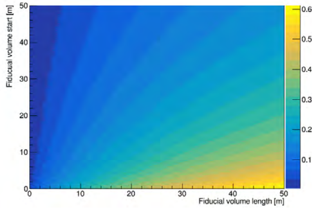
Figure 3.20: Fraction of K_L decays in fiducial volume, as a function of the start position (y-axis) and length (x-axis) of the fiducial volume
