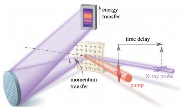
Figure 5.3: Time-resolved RIXS as recently realised in 17,25,27 . The momentum transfer is determined by the angle between the incident and scattered X-rays from the sample, along with the wavelength of the X-ray. The energy of the scattered photons is resolved by dispersing the X-rays with a grating or crystal analyser onto a two-dimensional detector. In tr-RIXS, a second pump laser pulse is used which arrives at a controllable time ahead of the incident X-rays.
