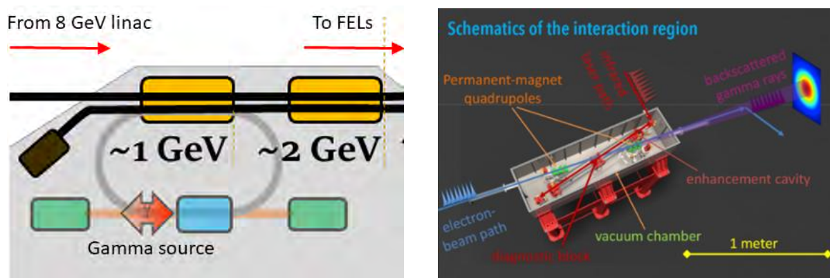
Figure A2.3: (Left) Illustration of ERL-driven ICS gamma source located within a full next-generation XFEL facility and (right) details of example laser-electron interaction point, comprising high finesse four-mirror bowtie laser cavity and permanent magnet quadrupole focused electron spot
