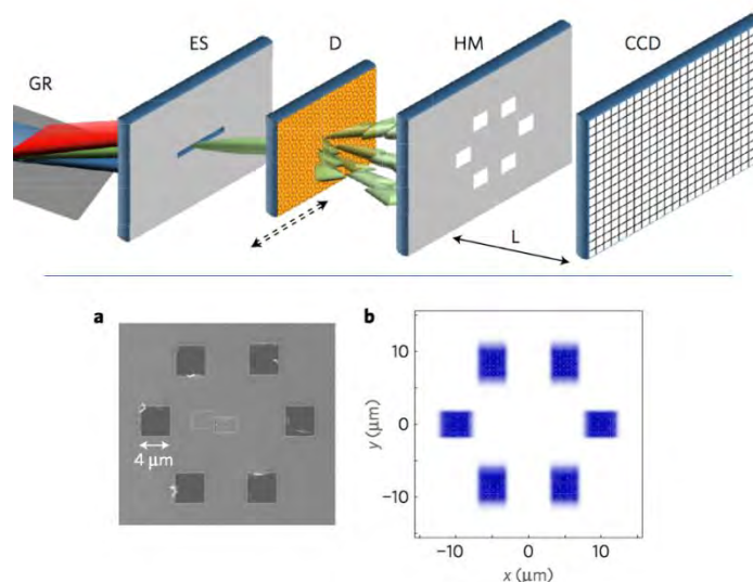
Figure 3.4: The first demonstration of incoherent diffraction using a microscale patterned mask at the FLASH XFEL. 85 (Top) Experimental setup with grating (GR), exit slit (ES), diffusor (D), hole mask (HM), and a CCD detector. a) Hole mask, b) reconstructed image.
