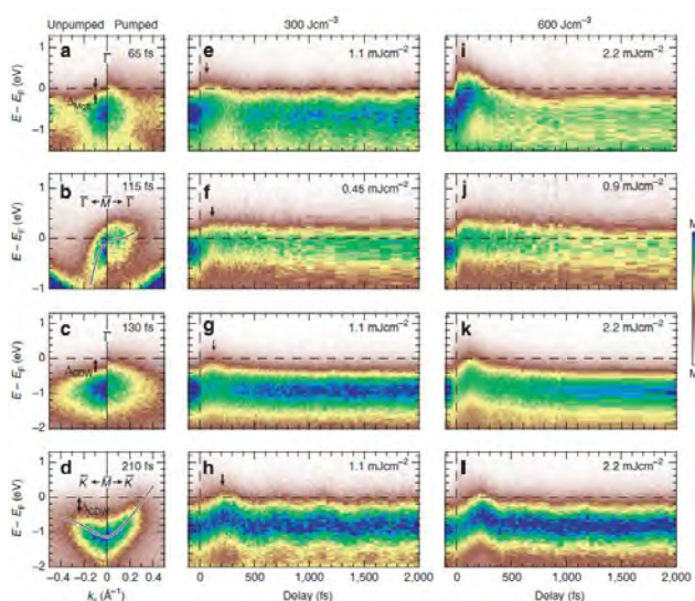
Figure 5.8: Time-resolved momentum-space view of the electronic structure in layered charge-density-wave compounds, including 1T-TaS 2 , 1T-TiSe 2 , and 1T-TaS 2 . 86
