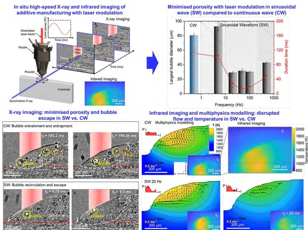
Figure 8.6: In situ high speed synchrotron X-ray and infrared imaging analysis of a laser additive manufacturing process with a nickel-based superalloy
