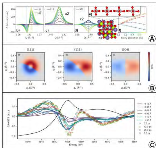
Left: Simulations and experiments of polaron (electronic charge carrier) formation in \text{Li}_x\text{Mn}_2\text{O}_4 a key electrode material. From UltraBat Consortium [4] .
