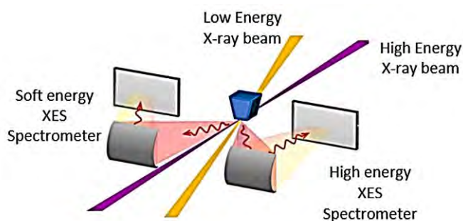
Figure 6.16: Schematic of a XES experiment performed in the soft and the hard X-ray regime simultaneously (adapted from 127 ).
