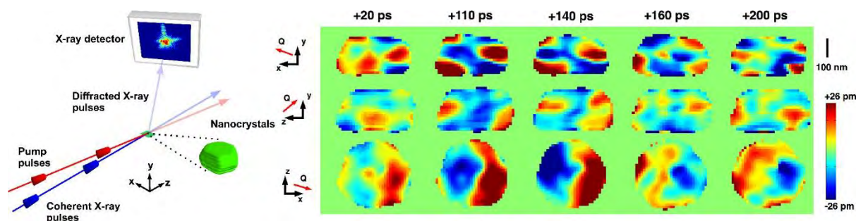
Figure 5.6: (Left) Schematic of the setup for ultrafast time resolved Bragg coherent diffraction imaging. Optical pulses (red) perturb the sample, generating phonons. Coherent X-ray pulses (generated from an XFEL) arrive a short time later where the diffracted pulses are recorded using an area detector. (Right) Imaging of acoustic phonons in a nanocrystal. Orthogonal cut planes through the nanocrystal showing the projected displacement as a function of delay time. For each delay time orthogonal slices taken from the centre of the nanocrystal are shown. The direction of the displacement field is given by the Q-vector in red. 68
