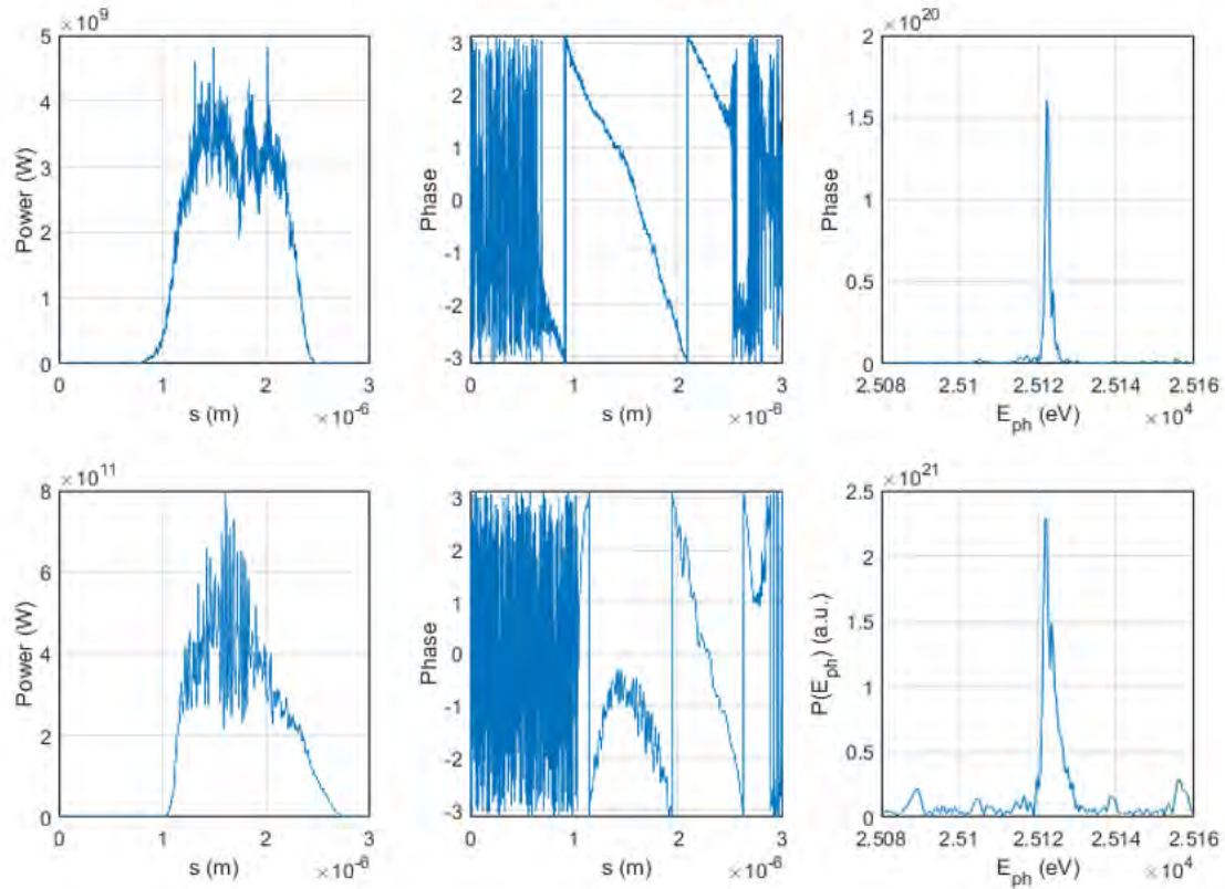
Figure 6.26: Example of HB-SASE at 25 keV (not baseline parameters) where post-saturation tapering has been applied, extending the undulator length by 80 m. Top row: the pulse profile, radiation phase and spectrum at the nominal saturation point. Bottom row: the output after tapering. The pulse peak power is 700 GW, the pulse energy is 1.6 mJ, the pulse duration is 2.6 fs, the FWHM bandwidth is 1 \times 10^{-4} and the time bandwidth product is \Delta\nu\Delta t \approx 1.5 .
