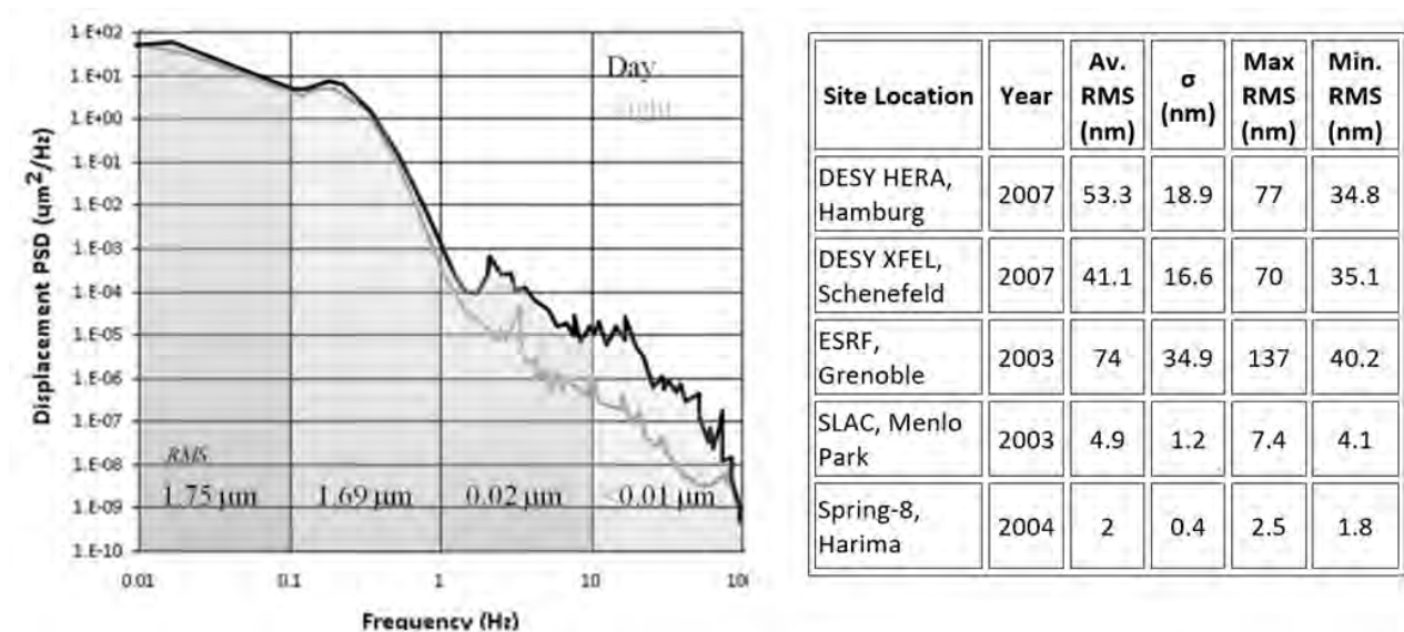
Figure 13.23: (a) Left, Generic ground noise spectrum of a typical quiet site. (b) Right, RMS ground vibration results for f > 1 Hz at various sites, [25]
