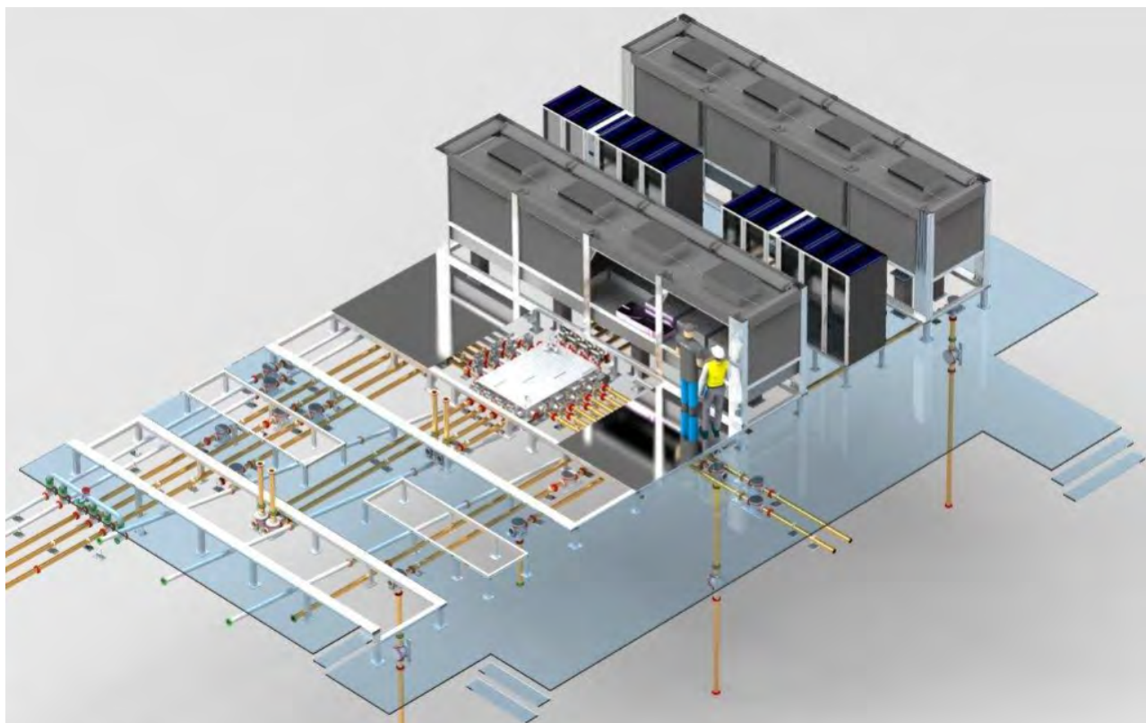
Figure 9.7: LCLS NEH laser hall and switch yard. The hall is a class 10000 clean room, with laser bays achieving class 100. The transport pipes and the central reconfigurable switchbox lie underneath the floor.
