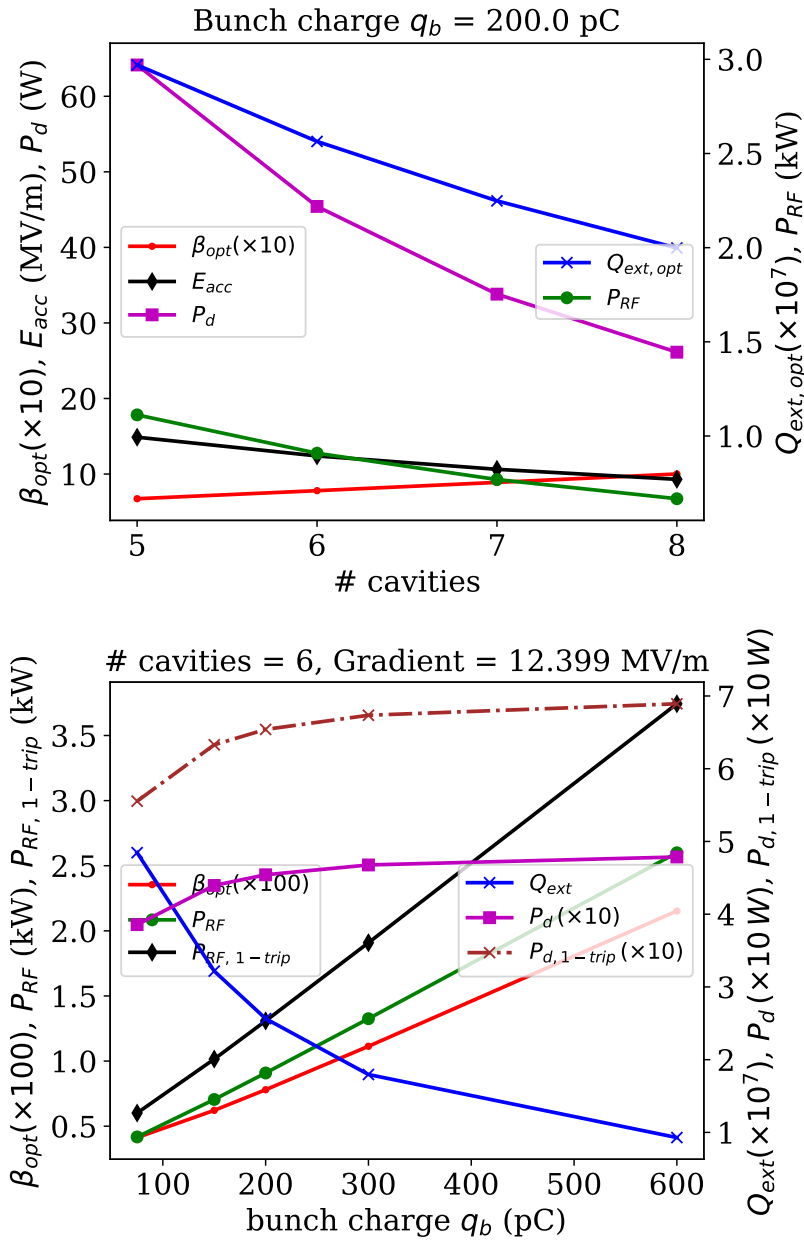
Figure 5.18: RF parameters optimised for different bunch charge and number of cavities, for bunch repetition rate of 1 MHz. Top: For 200 pC bunch, using different number of cavities. Bottom: For different bunch charge using six cavities.
