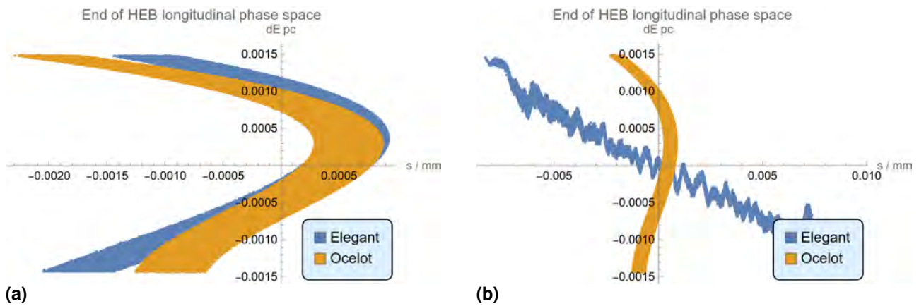
Figure 5.37: Longitudinal phase space distributions at the end of the HEB using a standard 4-bend chicane lattice as simulated using Elegant and Ocelot for a 75 pC bunch. (a) OCELOT compared to an Elegant simulation without synchrotron radiation, longitudinal space charge or wakefield effects. (b) OCELOT compared to an Elegant simulation which includes coherent synchrotron radiation in the dipoles, longitudinal space charge in the drifts and rf cavities, transverse wakefields in the rf cavities and longitudinal wakefields in the rf cavities.
