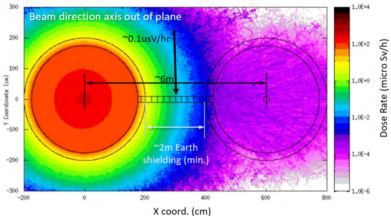
Figure 13.20: FLUKA Simulation Plot Radiation Dose Rates Concept Option FEL Tunnels
