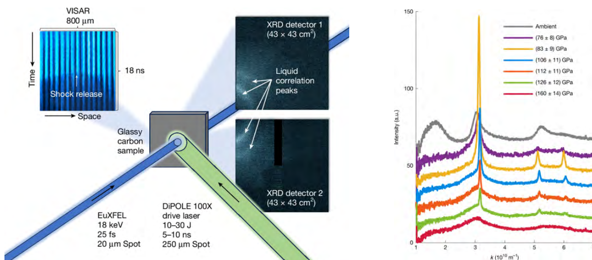
Figure 8.23: (Left) - X-ray diffraction of laser-shocked glassy carbon samples. (Right) - X-ray diffraction patterns for varying drive pressures. The transition from amorphous carbon structure to a liquid carbon state is observed as the pressure increases. Figures adapted from D. Kraus et al. Nature 642 351-355 (2025)
