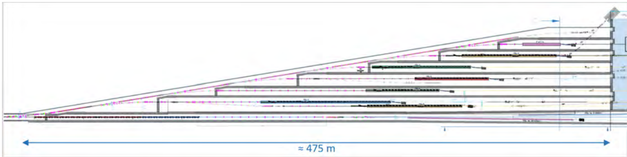
Figure 6.10: Engineering drawing of FEL switchyard
