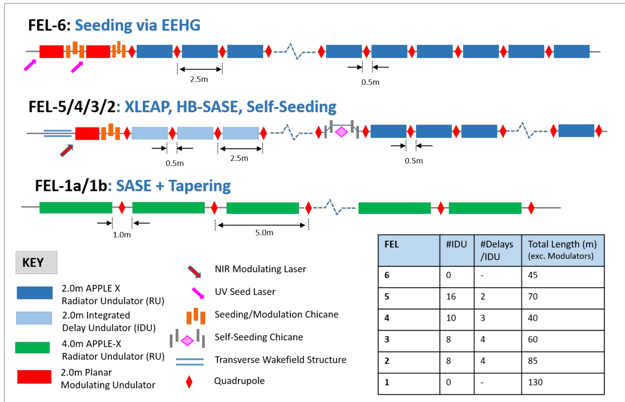
Figure 3.13: Schematic of FEL components. FEL-6 features two modulator lasers/undulators to enable EEHG seeding. FELs 2-5 feature relatively short undulator modules with integrated chicane delays to enable HB-SASE, with a chicane for self-seeding, while a modulator laser/undulator enables laser-driven ESASE/XLEAP. FEL-1a/1b have a simple undulator layout for SASE plus tapering for high-power output.
