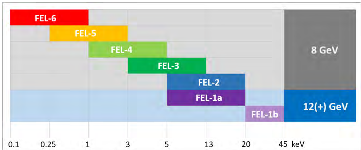
Figure 3.10: FEL tuning ranges.
