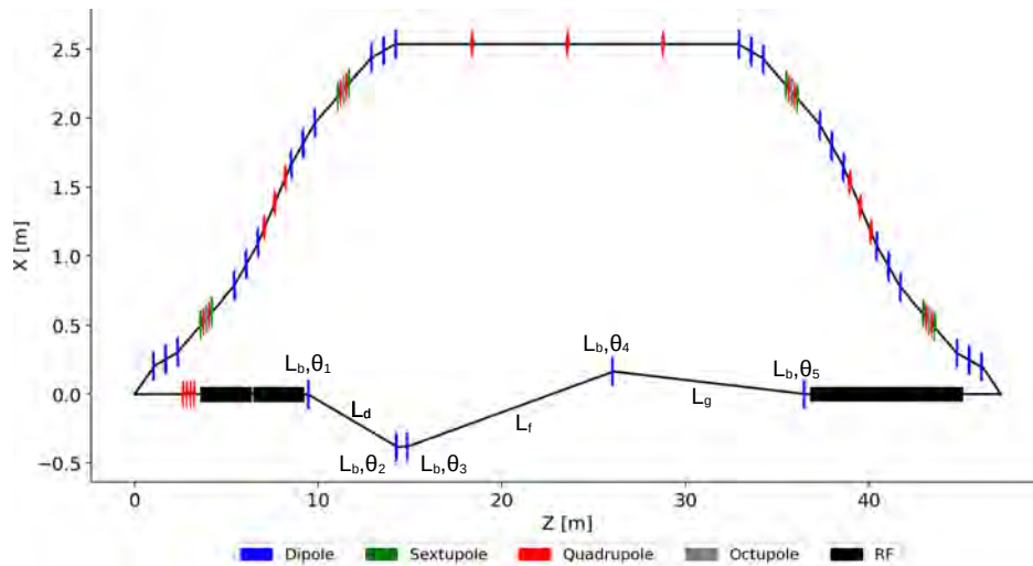
Figure 5.20: Schematic of the first bunch compressor. The beam can be directed onto either the arc (upper beam path) or the C5 chicane (lower beam path) through the use of magnetic or RF kickers.
