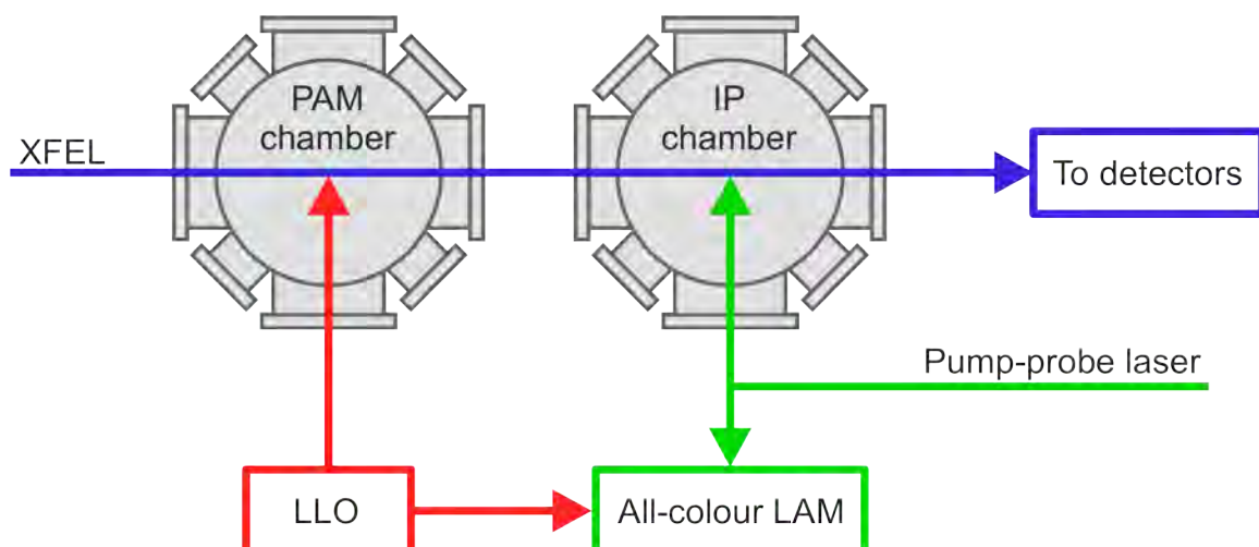
Figure 11.3: Hold: DART concept [44] , employing an all-colour LAM as close to the interaction point as possible. LLO: Local laser oscillator; LAM: Laser Arrival Monitor; PAM: Photon Arrival Monitor; IP: interaction point.
