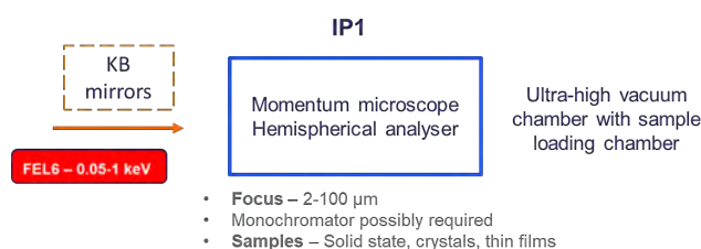
Figure 8.5: ES2 end station - FEL-6's fully tuneable operating range of 50 - 1000 eV would provide flexibility for studying different interfaces and photoelectron escape depth
