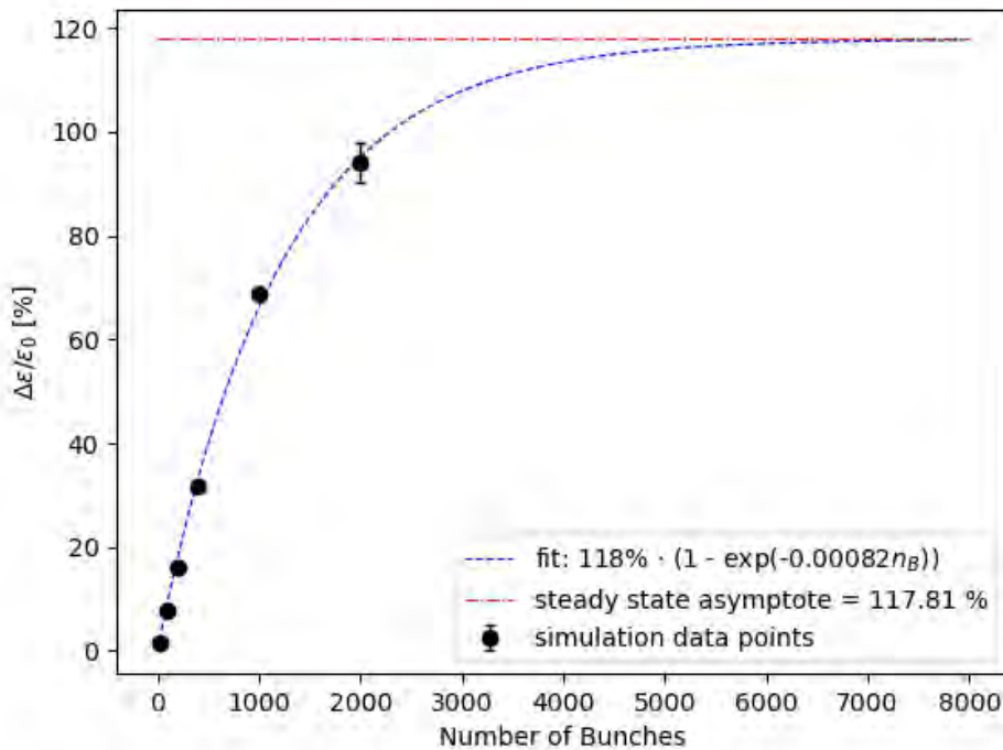
Figure 5.16: Unmitigated transverse emittance dilution due to a systematic 1\sigma transverse offset of the 75 pC beam returned by multiple PLACET simulations as a function of number of bunches.
