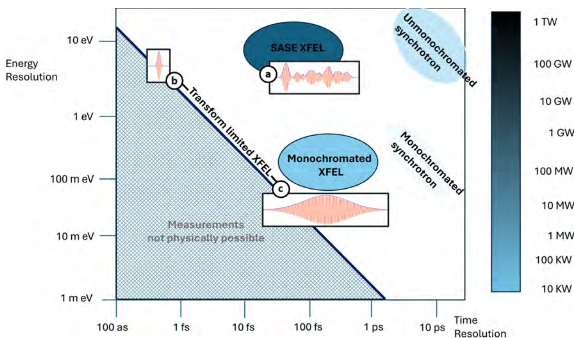
Figure 2.8: Science and Technology Case illustration of the requirement for near-transform-limited FEL operation across the X-ray range, compared to other sources. Indicative temporal profiles are superimposed for a SASE pulse (a), and transform-limited short (b) and long (c) pulses.
