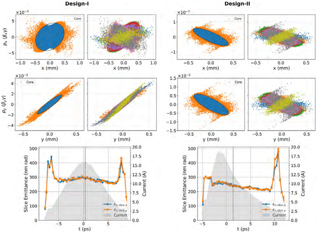
Figure 4.11: Transverse phase space comparison for Design-I and Design-II. Each row shows the full horizontal and vertical phase spaces at the injector exit, followed by 9-slice visualizations along the bunch to illustrate phase space rotation and alignment. The final row shows the horizontal and vertical slice emittance distributions along the bunch, plotted together with the one-dimensional current profile.
