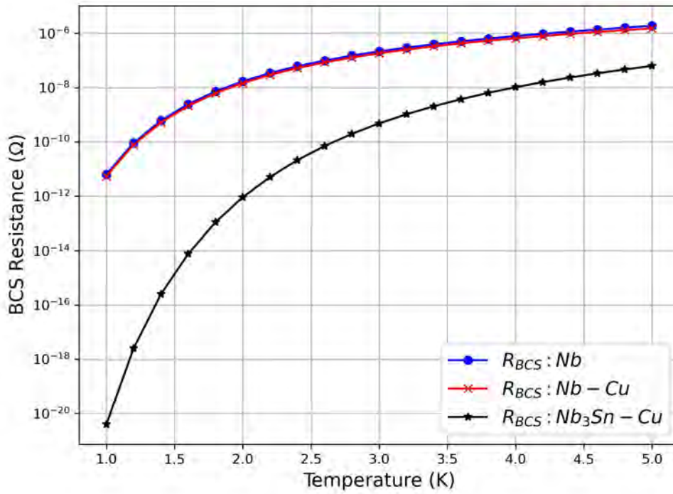
Figure 5.3: BCS resistance of Nb (blue), Nb on Cu (red), and Nb 3 Sn on Cu (black) as a function of temperature.
