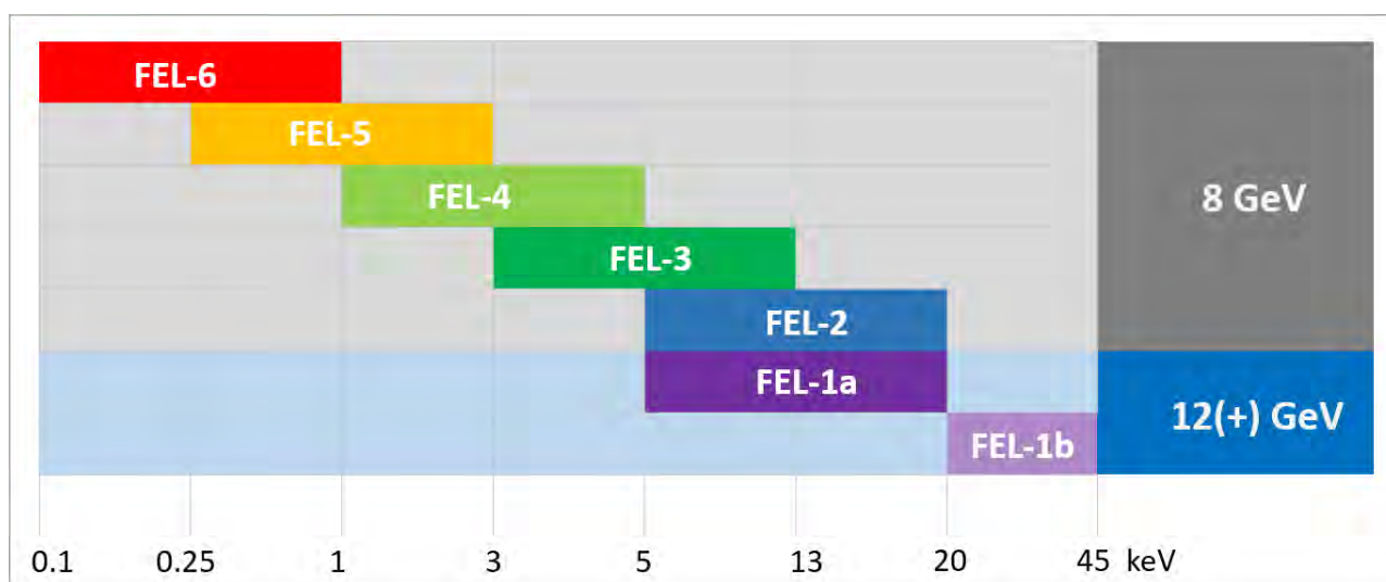
Figure 6.8: FEL Tuning Ranges
