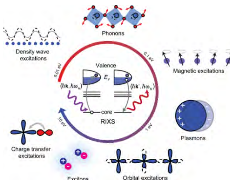
Figure 8.11: The Kramers-Heisenberg process for resonant inelastic x-ray scattering (RIXS) and the different excitations that it can probe. Image adapted from M. Mitrano et al. , Phys. Rev. X 14, 040501 (2024). Reproduced under terms of the Creative Commons Attribution License 3.0 BY
