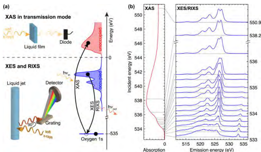
Figure 8.10: Illustration of X-ray absorption and emission methods along with RIXS, in this example for liquid methanol. (a) Schematic of transmission XAS geometry and XES/RIXS with a grating spectrometer. (b) Experimental data of XAS spectrum and RIXS spectra for excitation energies tuned through the X-ray absorption resonance. Figure adapted from S. Schreck et al. Struct. Dyn. 1 , 054901 (2014). Reproduced under terms of the Creative Commons Attribution License 3.0 BY
