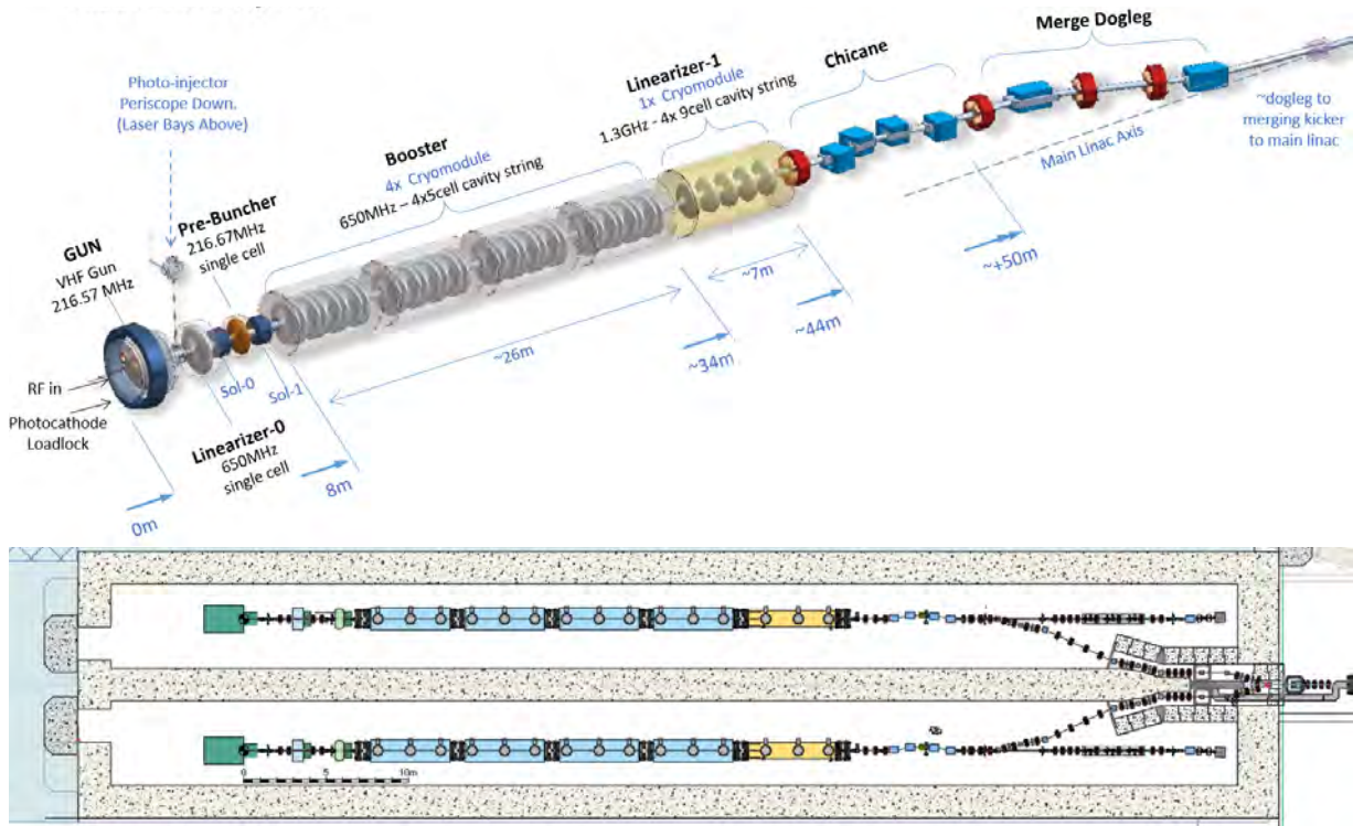
Figure 3.6: Novel injector concept for the Low Energy Beamlines, featuring RF compression (the pre-buncher) and magnetic compression (in the chicane), with a progressive increase in RF frequency for optimal beam quality. The length of the section is \sim 50 m. Two identical injectors are envisaged to run in parallel before merging into a single linac.
