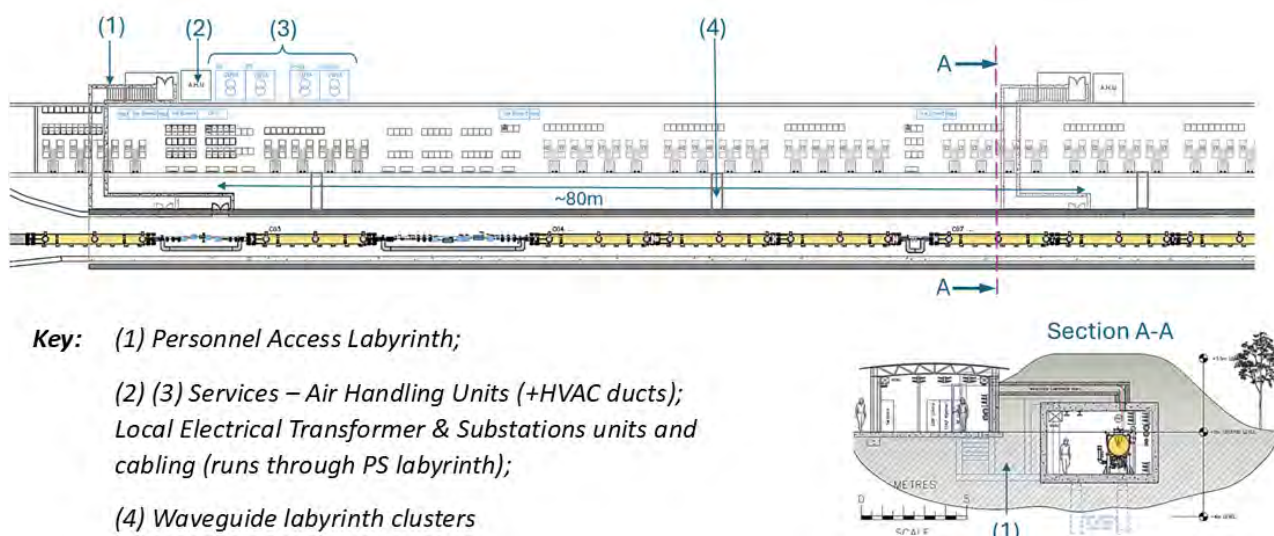
Figure 13.10: Portion of Linac Hall & RF services gallery – Plan view option A & Section.
