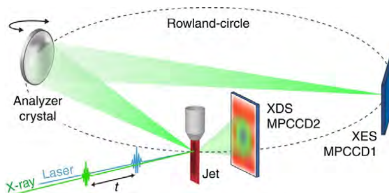
Figure 8.14: An example of a pump-probe set-up accommodating simultaneous XES and X-ray scattering from BL3 on SACLA for measurement of coupled electronic and structural dynamics following photoinduced electron transfer. Figure reproduced from S.E. Canton et al. Nat. Comms. 6 6359 (2015). Reproduced under terms of the Creative Commons Attribution License 3.0 BY
