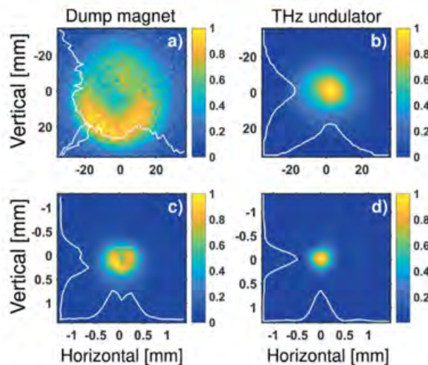
Figure 9.15: Replicated from [36]. (Top) THz transverse beam profiles at FLASH. (a) Dump magnet (the THz undulator is off), and (b) THz undulator tuned to 88 mm (3.4 THz), unfocused beam profiles measured in the THz hutch; beam position imaged 10 m from the virtual source. Note that the undulator profile is padded with zeros to fill in the same image size. (Bottom) The same beams focused. (c) Dump magnet beam (600 mm FWHM), and (d) THz undulator beam (350 mm).
