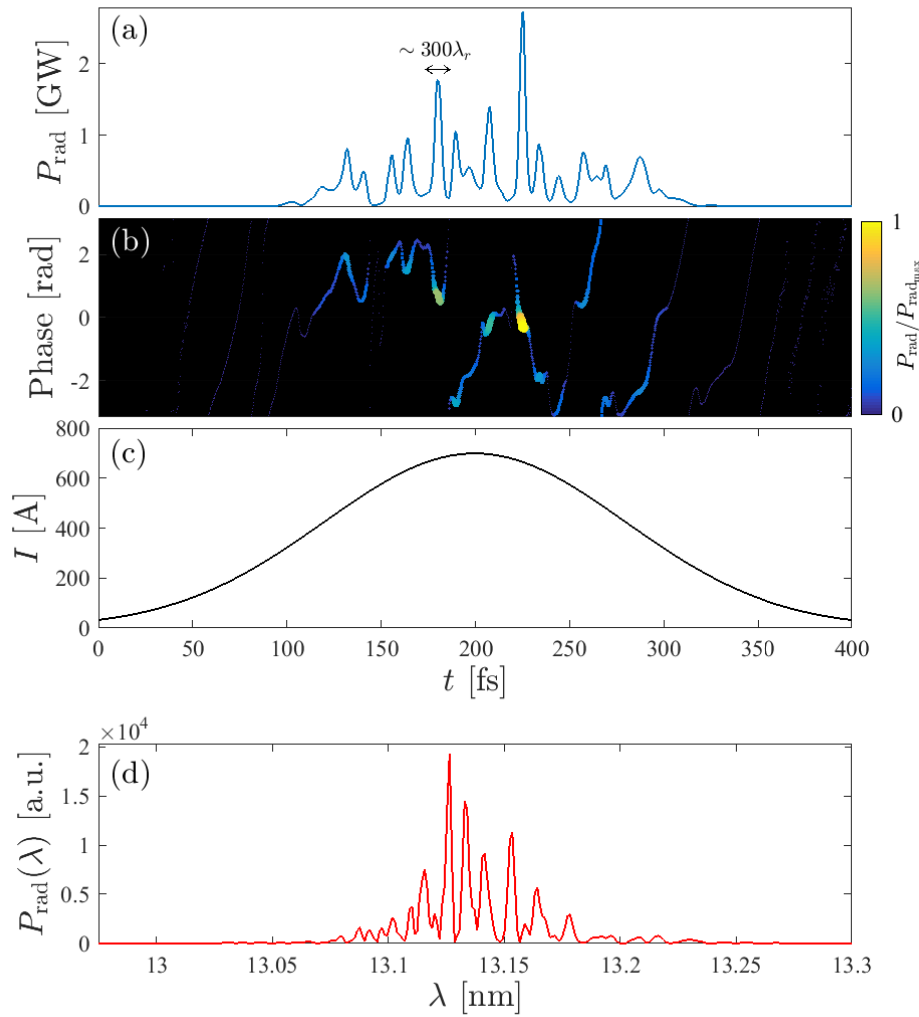
Figure 6.1: Example SASE properties. The figure shows simulation results for a high-gain SASE FEL with parameters similar to FLASH [1]. Results are shown at saturation: (a) radiation temporal profile comprising multiple spikes; (b) radiation phase showing phase correlation within but not between spikes; (c) the idealised Gaussian current profile used in the simulation and (d) the radiation spectrum, also comprising multiple spikes.
