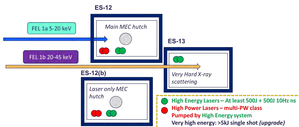
Figure 8.22: End station layout for FEL-1 featuring ES12 for a broad range of MEC experiments (including a separate hutch for laser-only experiments), and ES13 for very hard X-ray scattering measurements for materials under high static and dynamic load as well as time-resolved PDF (tr-PDF).
