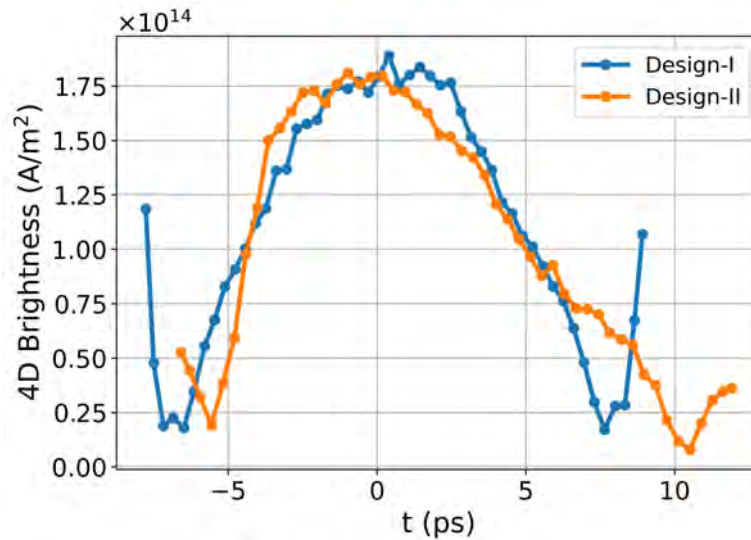
Figure 4.13: 4D beam brightness for Design-I and Design-II at the end of each injector beamline.
