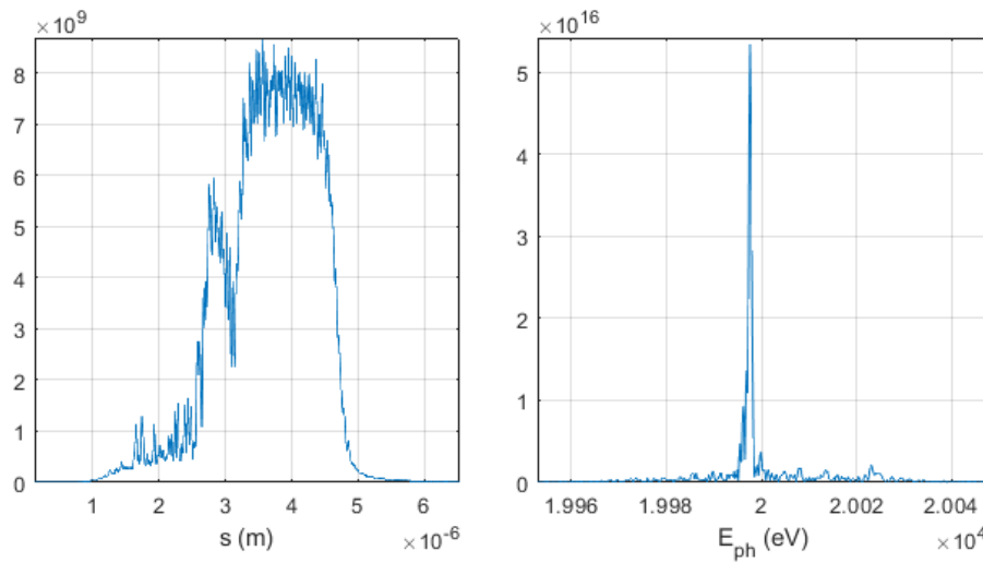
Figure 6.25: HB-SASE output from FEL-2 at 20 keV. Left: pulse profile at position of maximum brightness. Right: the pulse spectrum. The FWHM pulse duration is 6.5 fs and the FWHM relative bandwidth is 3.4 \times 10^{-5} , giving a time-bandwidth product \Delta\nu\Delta t = 1.0 .
