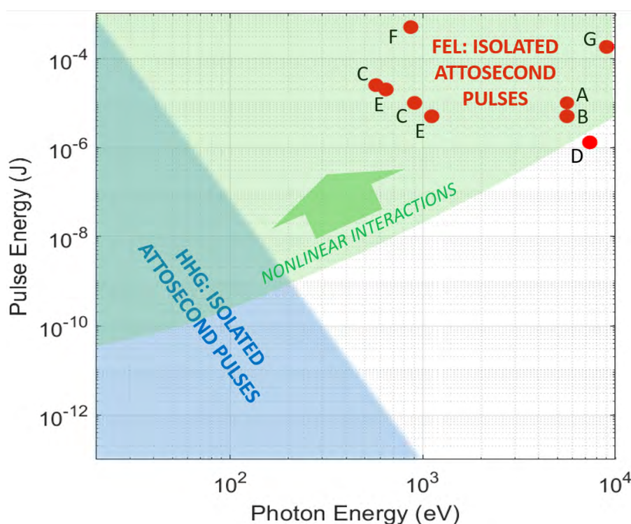
Figure 2.4: Experimentally demonstrated schemes for generating isolated attosecond pulses from XFELs, showing orders of magnitude enhancements in photon energy and pulse energy compared to HHG sources, thus extending access to the study of non-linear interactions for users. Schemes shown are as follows: A [18], B [19], C [20], D [21], E [22], F [23], G [24] Figure adapted from [25].
