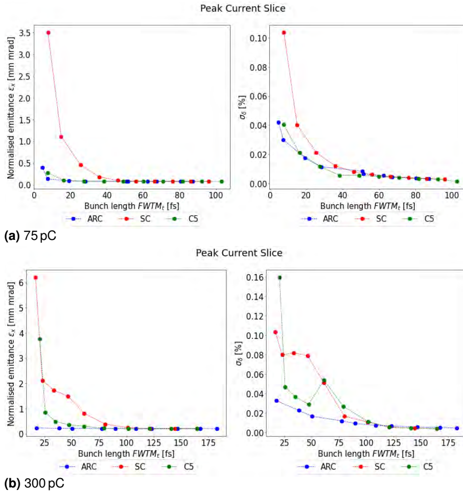
Figure 5.22: Bunch properties in the peak current slice at the end of the linac as a function of bunch length for the three compression schemes considered at two different bunch charges (above: 75 pC; below: 300 pC). The plots on the left show the normalised slice emittance in the bending plane, and those on the right show the slice energy spread.
