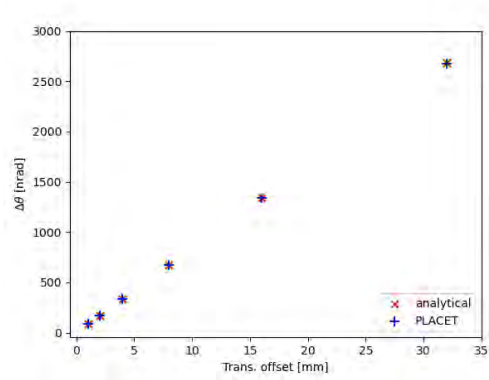
Figure 5.15: Comparison of LR wakes in PLACET to the analytical model outlined in Figure 5.14 and Equation 5.18.
