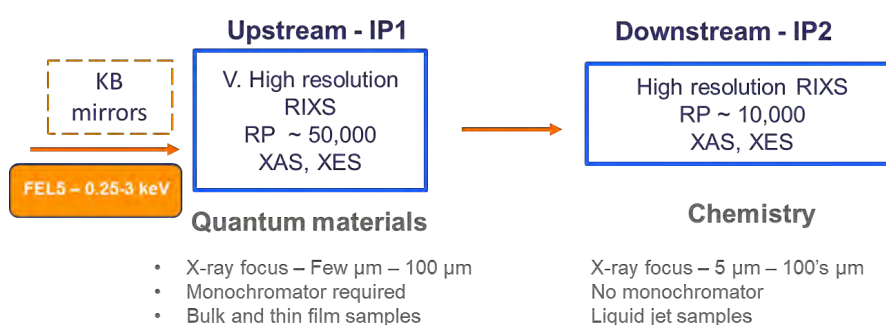
Figure 8.12: ES4 for RIXS and other photon spectroscopy methods on FEL-5. Note - these two interaction points may require splitting into two hutches due to the differing requirements for monochromation
