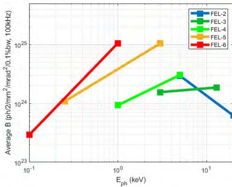
Figure 6.31: Predicted average brightness in long pulse transform-limited mode at a repetition rate of 100 kHz.
