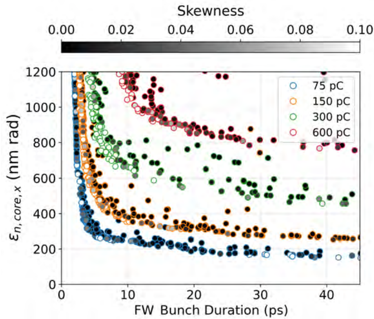
Figure 4.6: Pareto fronts for core emittance and bunch duration obtained for all bunch charges after initial acceleration up to the end of the first booster cryomodule in the Design-I beamline shown in Figure 4.5. The skewness of the longitudinal charge distribution is represented by a colormap ranging from dark to light, explaining the spread in the Pareto front compared to a typical one-dimensional trade-off curve.
