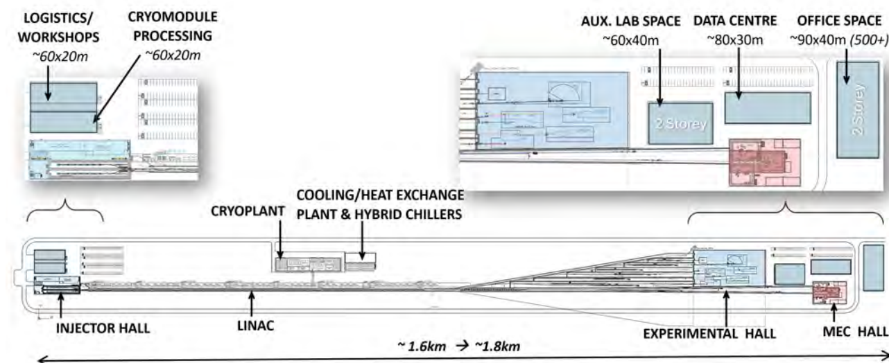
Figure 3.21: Layout of the next-generation XFEL design to scale, including ancillary and auxiliary buildings.
