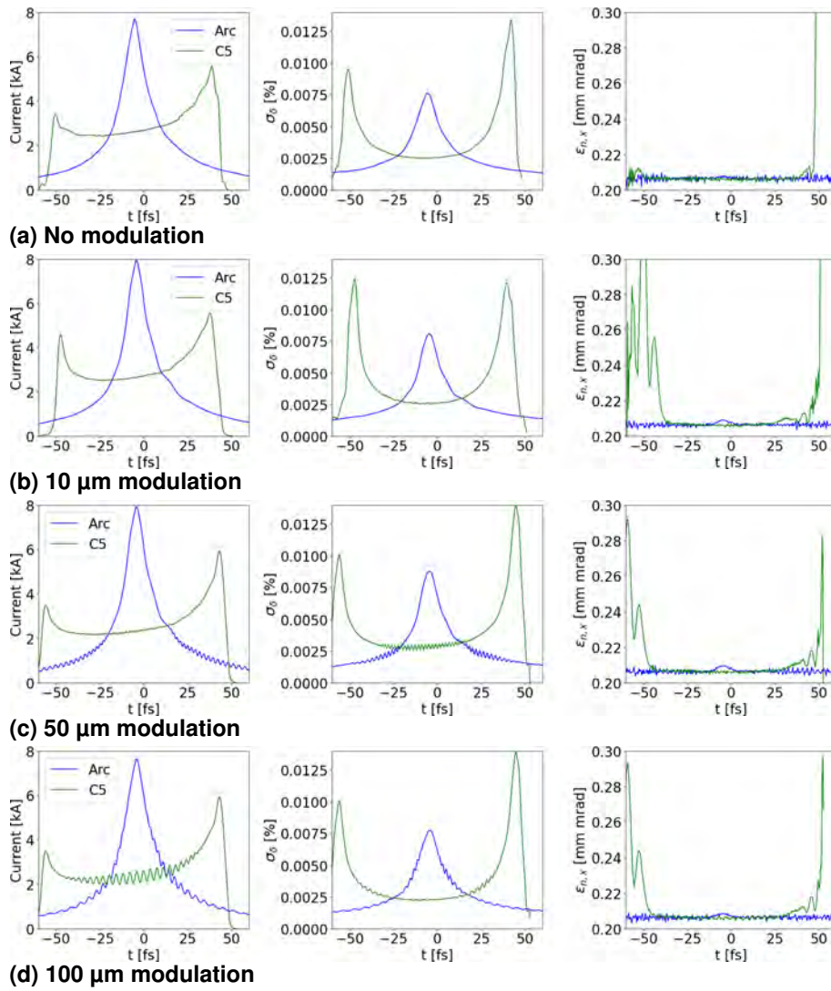
Figure 5.26: Slice current (left), energy spread (middle) and normalised horizontal emittance of the 300 pC electron bunch at the entrance of the FEL from the arc (blue) and five dipole chicane (green) compression schemes. The initial electron bunches had no initial density modulation (top/first), 10 \mu\text{m} initial density modulation (second), 50 \mu\text{m} initial density modulation (third), and 100 \mu\text{m} initial density modulation (fourth/bottom).
