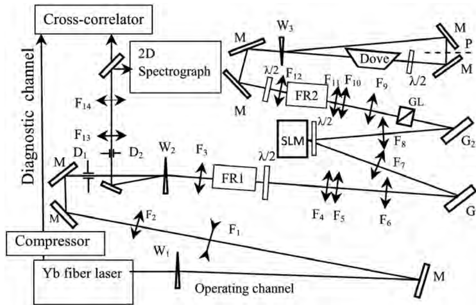
Figure 4.1: Reproduced from [76]. Schematic diagram of experimental setup: M, mirror; G1;2, diffraction gratings; FR1, FR245°, Faraday rotators; SLM, spatial light modulator; GL, Glan prism; W1,2,3, calcite wedges; D1,2, diaphragms; P, plane of image transfer from grating; G2, Fi (i = 1... 14) lenses (F1 = -140 mm, F2 = 350 mm, F3 = 400 mm, F4 = 169 mm, F5 = 259 mm, F6 = 369 mm are spherical; F7 = F8 = 405 mm are cylindrical; and F9 = 368 mm, F10 = 174 mm, F11 = 394 mm, F12 = 414 mm, F13 = 160 mm, F14 = 260 mm are spherical).
