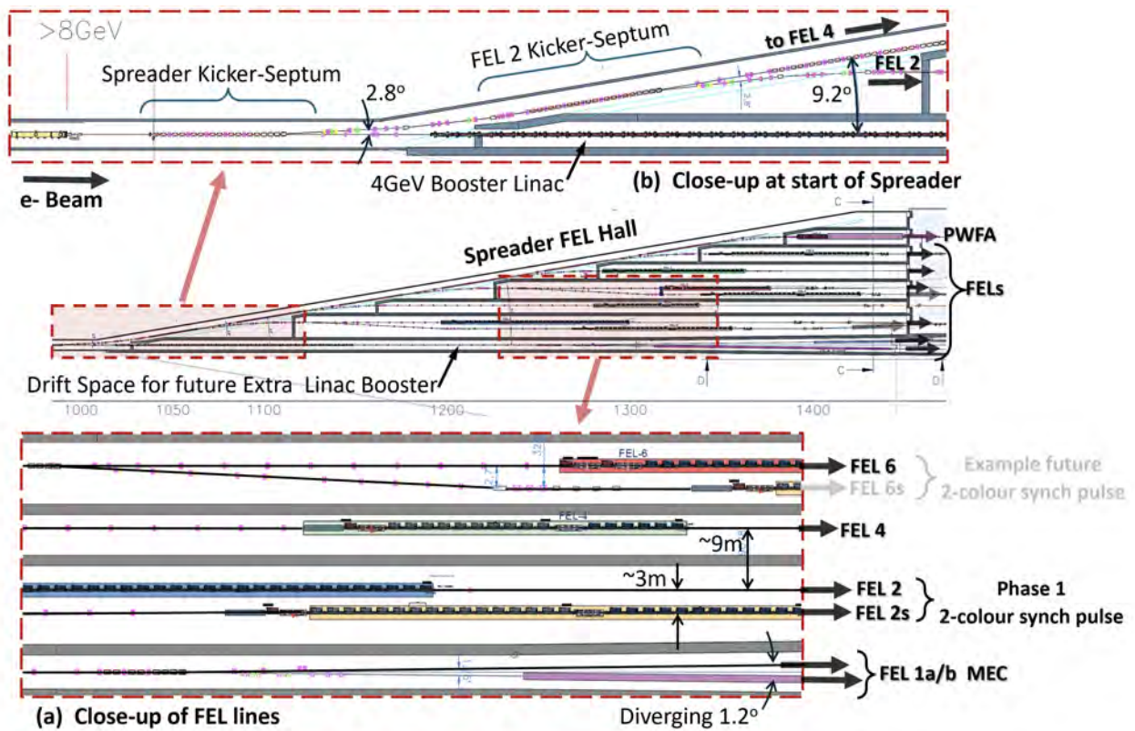
Figure 13.11: 2D Plan View of the Spreader and FEL Hall
