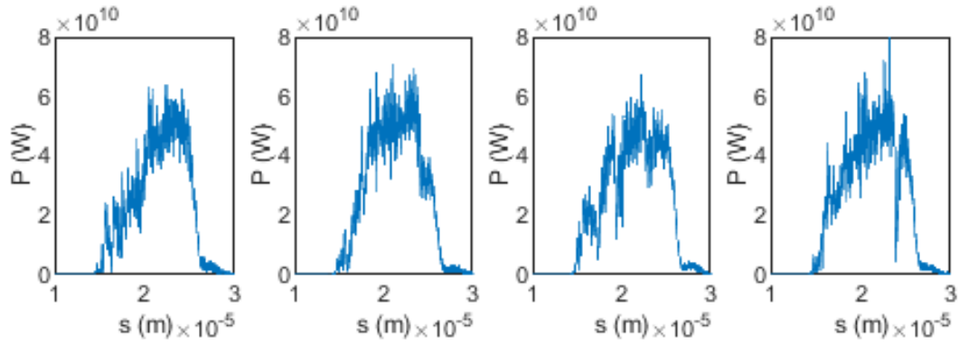
Figure 6.22: HB-SASE pulses at median position of maximum 6D brightness.
