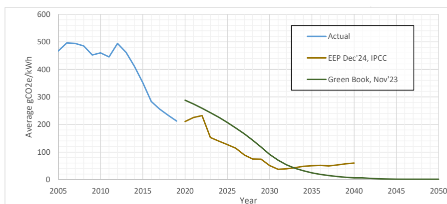
Figure 14.1: Carbon intensity of electricity generation, in gCO 2 e/kWh, for the period 2005-2050. The blue line shows the actual intensity up to 2019; the green and brown lines are projections from the UK government's Green Book and EEP documents respectively.
