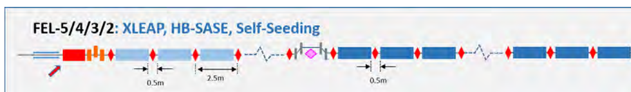
Figure 6.15: Schematic Layout of FELs 2/3/4/5
