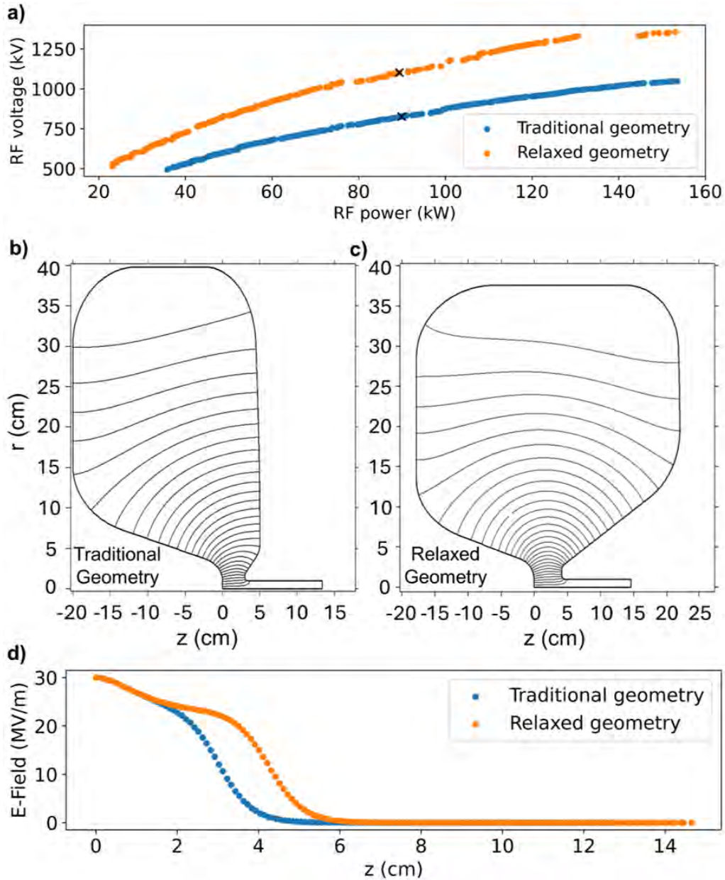
Figure 4.3: (a) Pareto fronts for each gun design. The selected design is marked with a black cross. (b) Optimised traditional gun geometry. (c) Optimised relaxed gun geometry. (d) Peak electric field on axis for each gun design.
