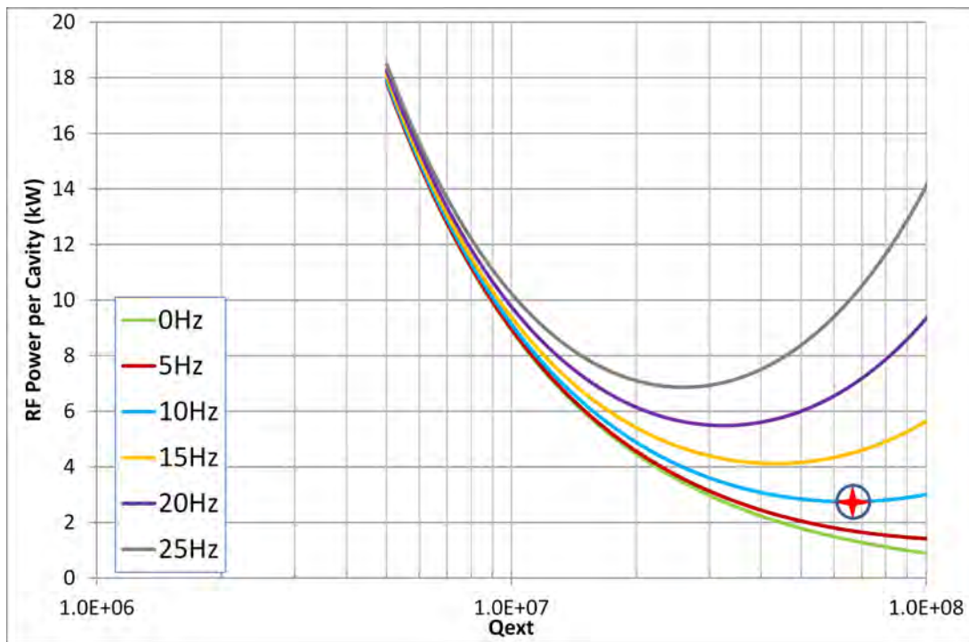
Figure 5.2: Microphonic assessment of 1.3 GHz cavities at gradient 19 MV/m.
