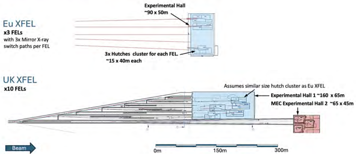
Figure 13.15: Comparison of Main Experimental Halls: European XFEL and UK XFEL
