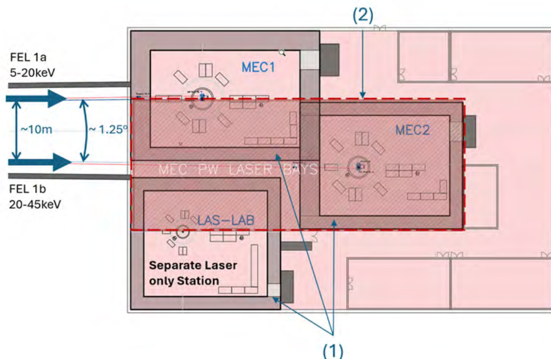
Figure 13.16: MEC Experimental Hall , showing (1) Concrete shielded 2x MEC interaction experimental areas with 1 ancillary laser only and (2) Petawatt high power lasers to be mounted above on stable concrete hatch roof with a short run periscope down to the experimental areas.
