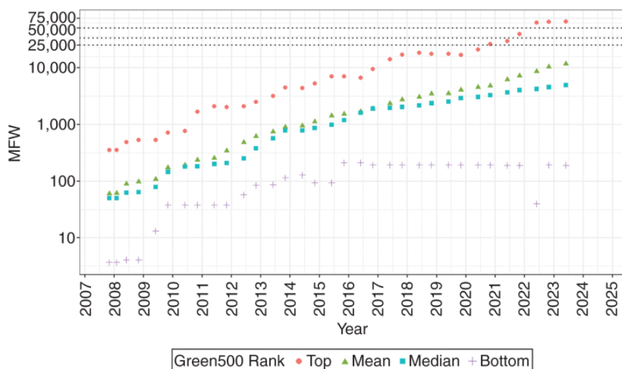
Figure 14.2: Progression of the energy efficiency of supercomputers on the Green500 list between 2007-23, measured in MFLOPs/W [6].
