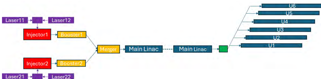
Figure 4.19: Example scheme of the UK XFEL with two injectors and 6 FELs.
