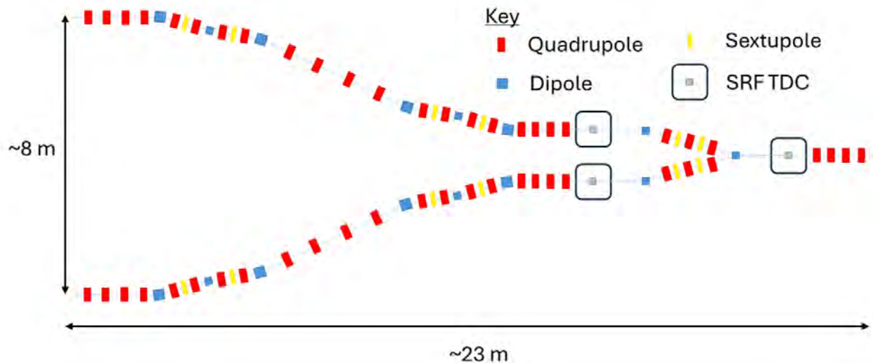
Figure 4.22: A sketch of a potential scheme for combining bunches from two separate injectors into a common main linac. This beamline uses TDCs to do the final combining and should be 2nd order achromatic and isochronous.
