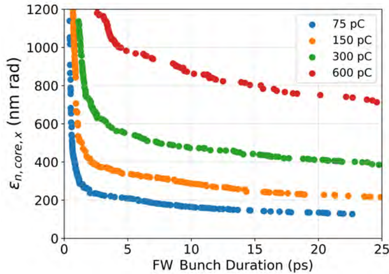
Figure 4.8: Pareto fronts for core emittance and bunch duration obtained for all bunch charges after initial acceleration up to the end of the first booster cryomodule in Design-II beamline shown in Figure 4.7 .
