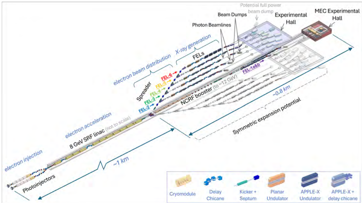
Figure 13.5: Illustrative 3D Schematic CAD Layout
