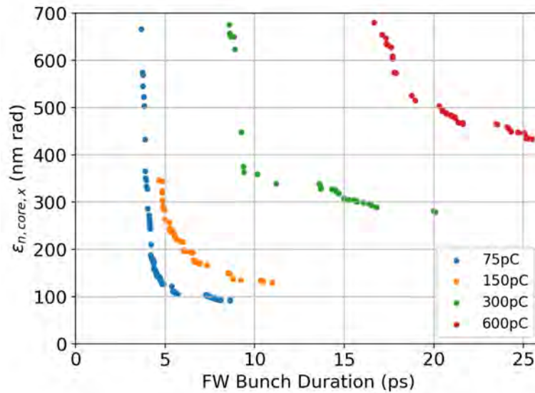
Figure 4.16: Pareto fronts for core emittance and bunch duration obtained for all bunch charges after initial acceleration up to the end of the booster cryomodule for the L-band injector.
