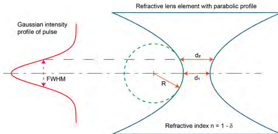
Figure 7.5: Simple model for calculating the thickness of a CRL that contributes to propagation time difference. R is the central radius of curvature of the lens
