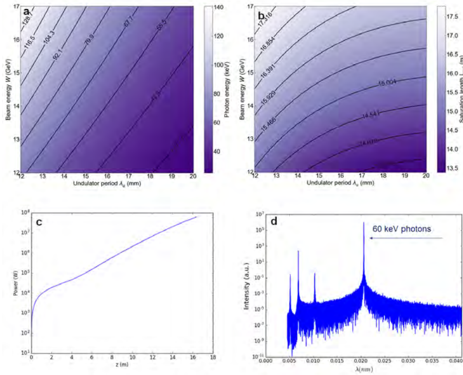
Figure 5.35: Estimation of plasma-XFEL performance and preliminary Puffin XFEL simulation of the brightness-boosted witness beam. (a-b) Estimation of XFEL performances as a function of beam energy and undulator period. (c-d) Preliminary simulation of the plasma-XFEL at E_{ph} = 60 keV.
