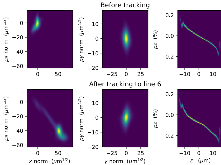
Figure 5.31: The horizontal (left), vertical (centre) and longitudinal (right) phase space of the bunch before (upper) and after (lower) tracking to the end of the spreader line to FEL-6. Horizontal and vertical phase space coordinates have been normalised using the Courant-Snyder parameters to make them invariant through linear beam transport.
