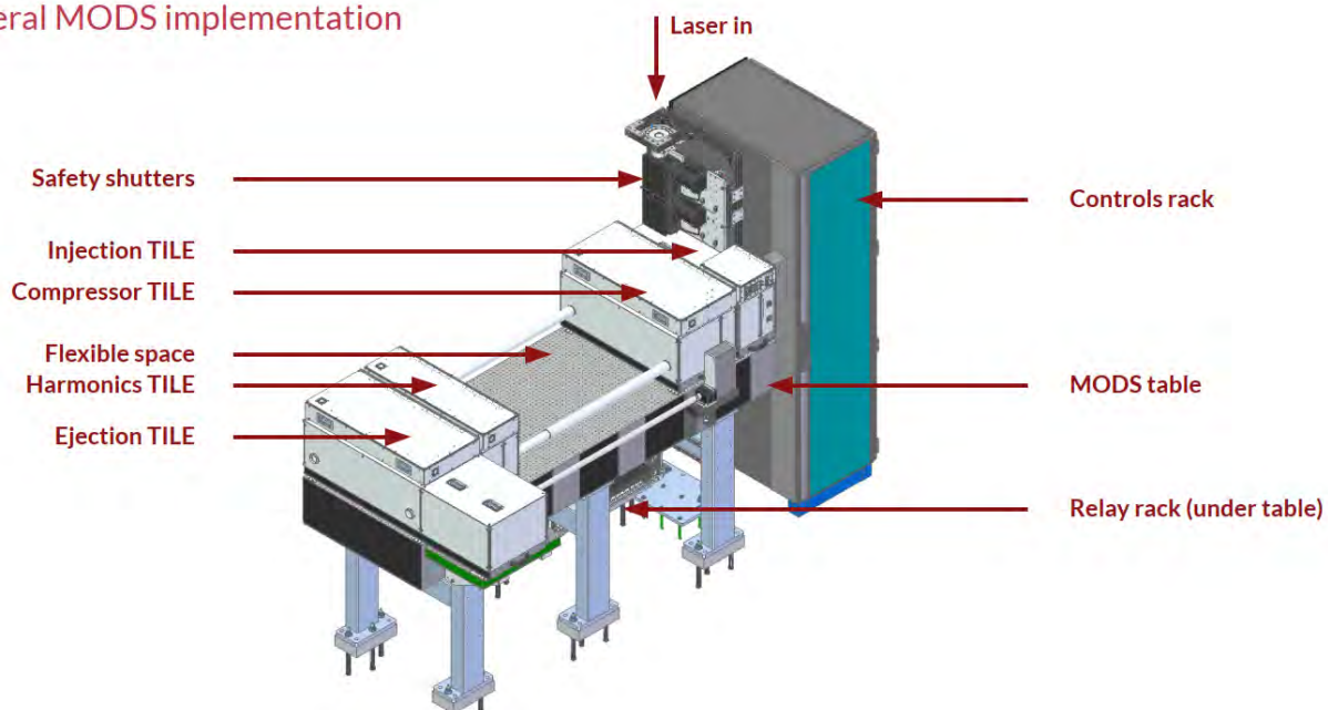
Figure 9.8: MODS system at LCLS showing an example implementation of the reconfigurable TILE layout.
