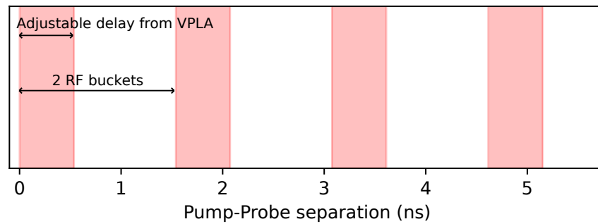
Figure 5.30: The highlighted red regions show the range of possible pump-probe separations that can be provided by the double FEL line using a combination of RF bucket selection and the variable path length adjustment chicane (VPLA).
