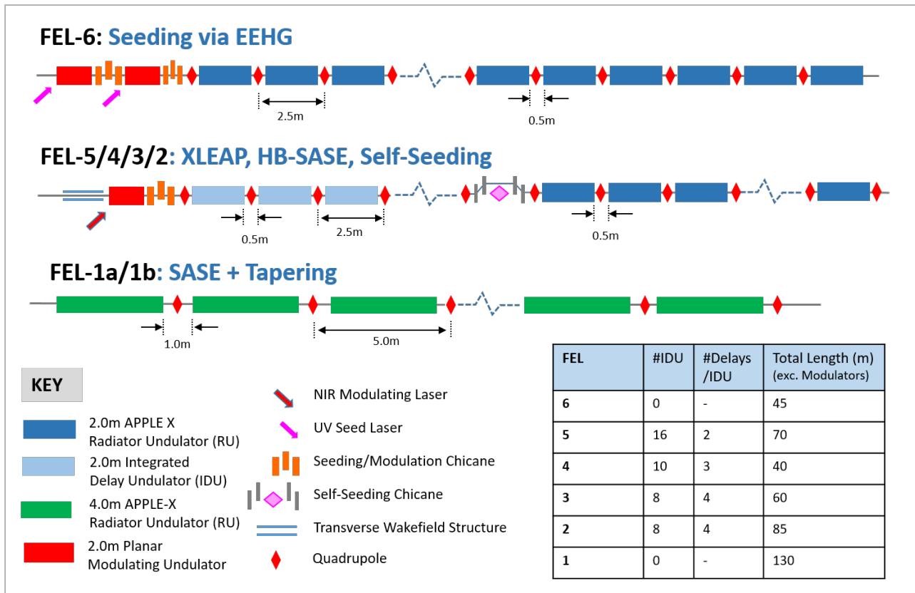
Figure 6.9: Schematic of FEL components.
