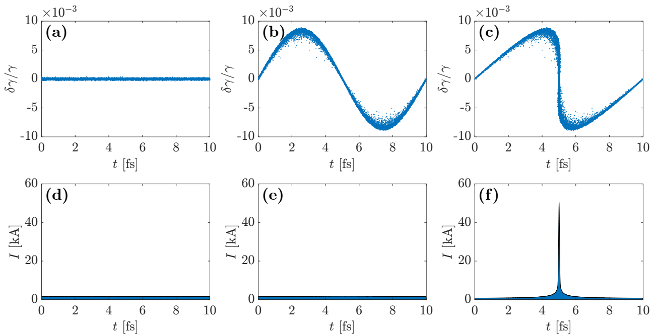
Figure 6.27: Simulation of electron bunch modulation in the ESASE scheme for the selected UK XFEL case. The upper row shows the longitudinal phase space (a) before and (b) after the first undulator section as well as (c) after the magnetic chicane. The lower row shows the corresponding current profiles (d) before and (e) after the first undulator section as well as (f) after the magnetic chicane.
