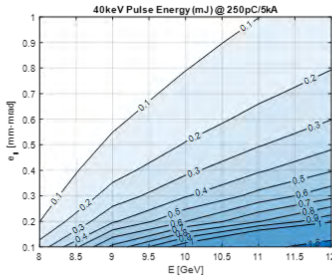
Figure 4.23: Lines of equivalent FEL pulse energy for different beam emittances and energies, for a photon energy of 40 keV.
