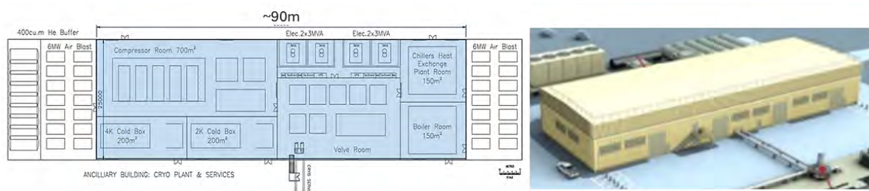
Figure 13.18: 90 \times 25 m Cryoplant Plan (left) vs Recent LCLS-II-HE install 75 \times 25 m (right)
