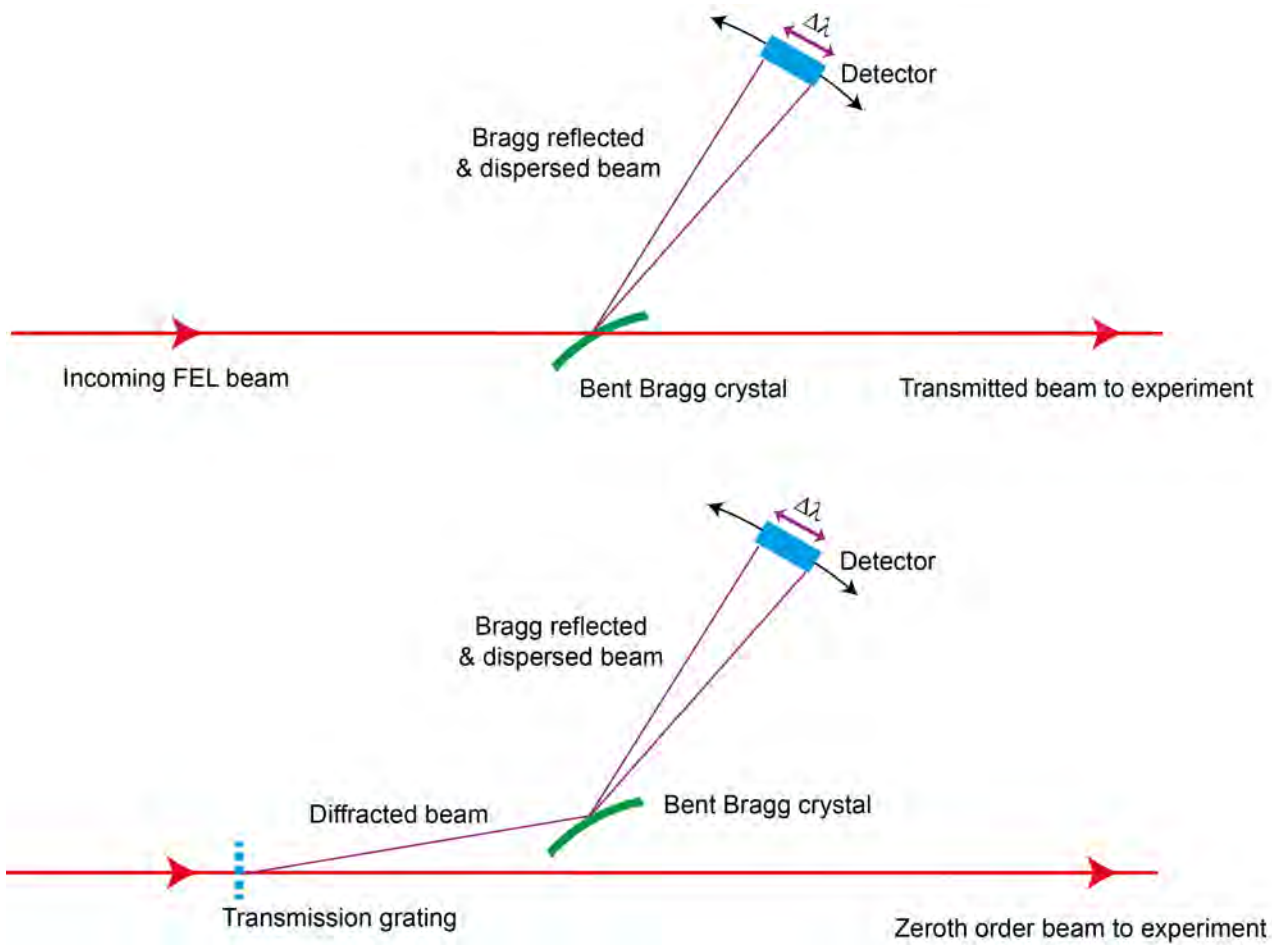
Figure 7.15: Schema showing the operating concepts of the two types of Bragg crystal spectrometers. Top: the crystal is the beam splitter. Bottom: a transmission grating is the beam splitter
