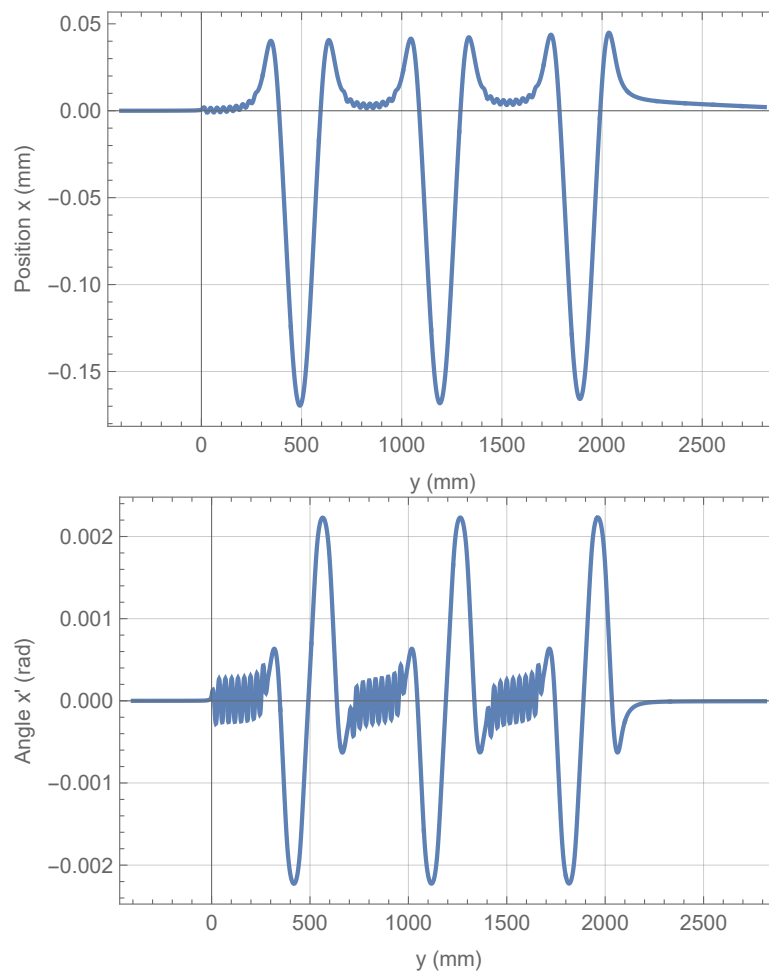
Figure 6.38: Trajectory of an 8 GeV electron: x (mm) (top) and x' (rad) (bottom).
