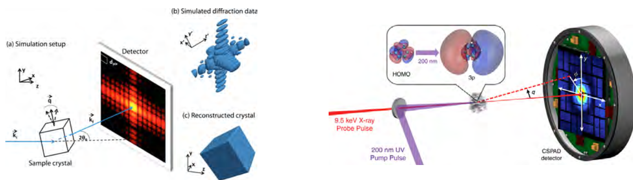
Figure 8.16: The two main experimental geometries for ES9. Left - Schematic of a Bragg CDI geometry. Adapted from H Ozturk et al. New J. Phys. 19 103001 (2017). Right - Schematic of ultrafast, time-resolved X-ray scattering with a gas sample of 1,3-cyclohexadiene (CHD). Adapted from H Yong et al. Nat Comms. 11 , 2157 (2020). Reproduced under terms of the Creative Commons Attribution License 3.0 BY
