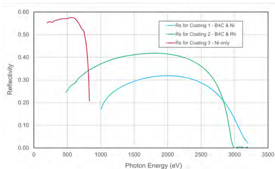
Figure 7.13: Calculated S-reflectivity of the complete soft x-ray beamline from 200 to 3200 eV for different mirror coating combinations
