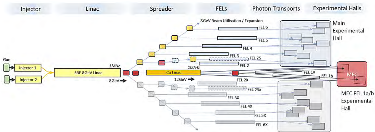
Figure 13.3: Schematic illustration of UK XFEL key elements
