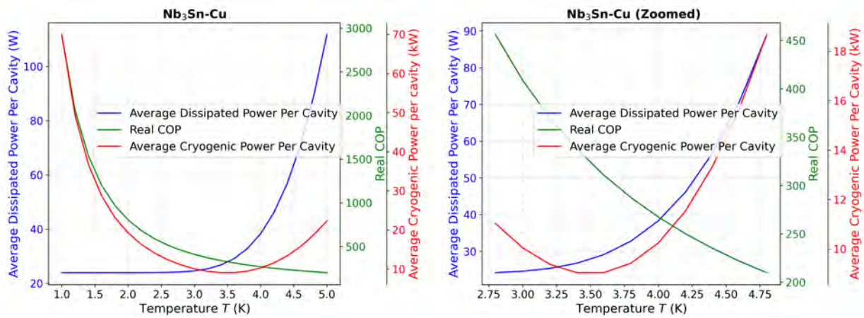
Figure 5.7: Normal-scale (left) and magnified (right) plots as functions of temperature, showing the average dissipated power per cavity (blue), the real coefficient of performance (COP) (green), and the average cryogenic power per cavity (red), for the Nb 3 Sn on Cu cavities.
