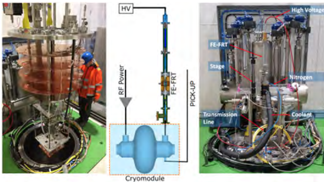
Figure 5.9: Ferroelectric fast reactive tuner under test with 400 MHz HL-LHC prototype crab cavity [30].
