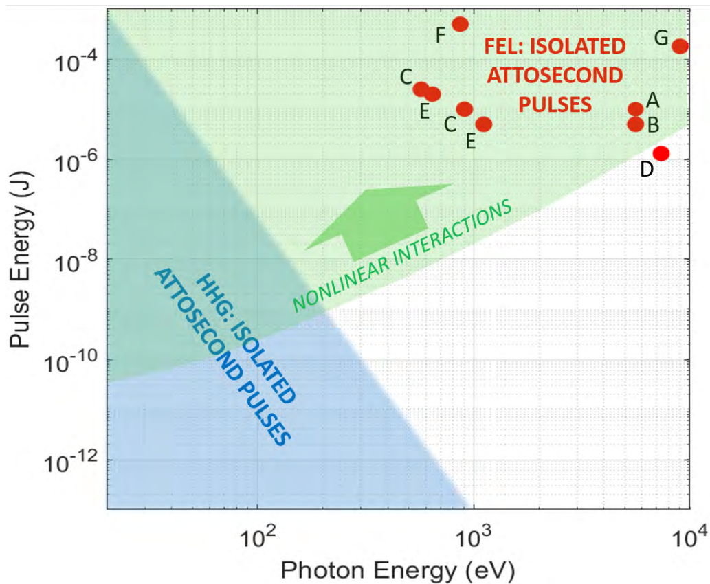
Figure 6.7: Experimentally demonstrated schemes for generating isolated attosecond pulses from FELs, showing orders of magnitude enhancements in photon energy and pulse energy compared to HHG sources, thus enabling access to the study of nonlinear interactions. Schemes shown are as follows: A [39], B [35], C [46], D [40], E [41], F [45], G [42]. Figure adapted from [47] during discussions with the Author.
