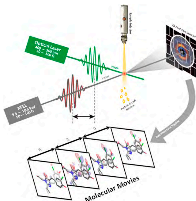
Figure 8.18: Schematic of a time-resolved Serial Femtosecond Crystallography (tr-SFX) experiment, enabling the production of ultrafast molecular movies. Reproduced from S. Perrett et al. J. Chem. Phys. 160, 100901 (2024). Reproduced under terms of the Creative Commons Attribution License 3.0 BY.
