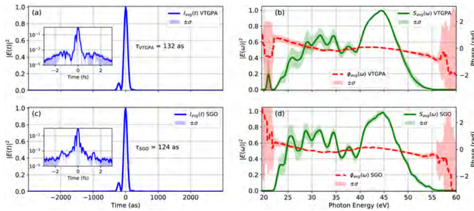
Figure 9.10: Example of an HHG attosecond pulse replicated from [21]. Retrieval of the XUV isolated attosecond pulses. (a) Retrieved XUV pulse intensity envelope normalized to its maximum value. The blue line corresponds to the average over all Volkov-transform generalized projection algorithm retrievals, and the shaded area corresponds to one standard deviation around the mean (not visible on the linear scale). The inset shows the intensity envelope on a logarithmic scale. (b) Retrieved average spectrum (green) and spectral phase (red dashed line) corresponding to the pulse in (a). The shaded areas correspond to one standard deviation around the means. (c) and (d) show the corresponding results found with the streaking global optimisation retrievals.
