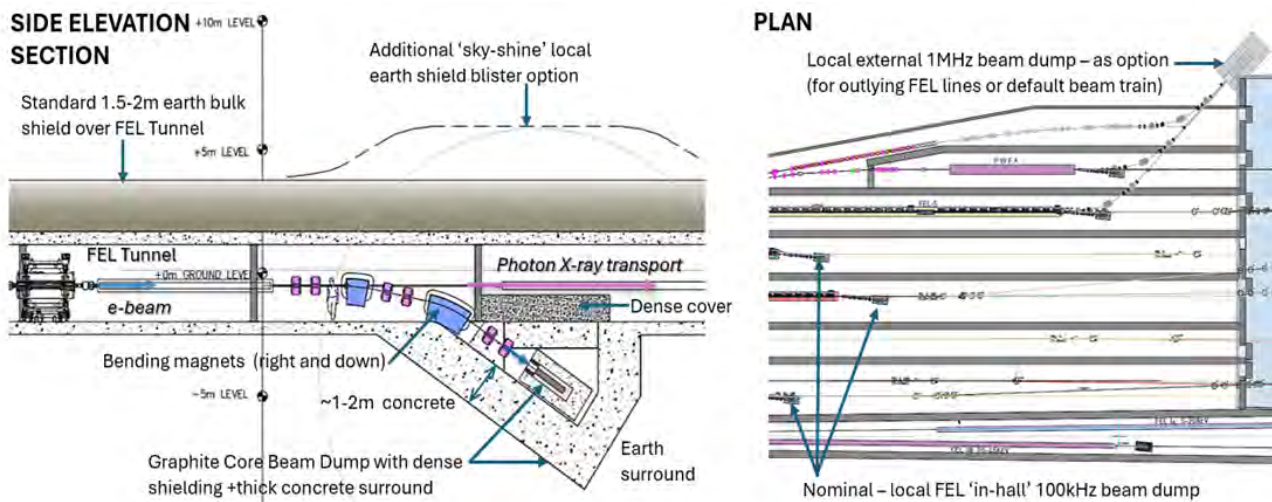
Figure 13.22: Beam dump concepts - Left: illustrates a side elevation of a local <250 kW beam dump within the FEL hall. Right: shows a conceptual layout for a shared high-power (~1 MHz, >2 MW) beam dump located outside the FEL hall, with associated beam transport lines.
