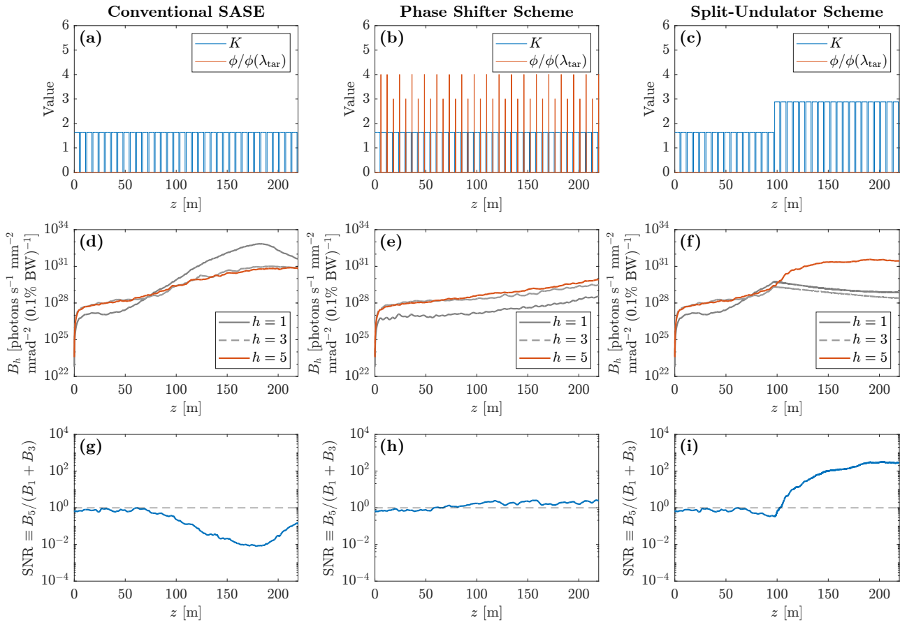
Figure 6.29: Simulation results. The three columns represent the three FEL schemes: conventional SASE (left), the phase shifter scheme (centre) and the split-undulator scheme (right). The top row illustrates the undulator and phase shifter configurations along the FEL line. The middle row displays the brightness B_h as a function of the distance z along the FEL line for harmonic numbers h = 1, 3, 5 of the wavelength \lambda_{\text{res}} . The bottom row shows the SNR as a function of z , defined in this context as B_5/(B_1 + B_3) .
