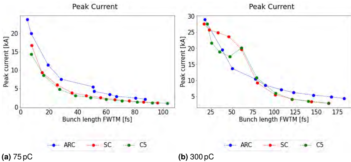
Figure 5.23: Peak current slice at the end of the linac as a function of bunch length for the three compression schemes considered at two different bunch charges (left: 75 pC; right: 300 pC).
