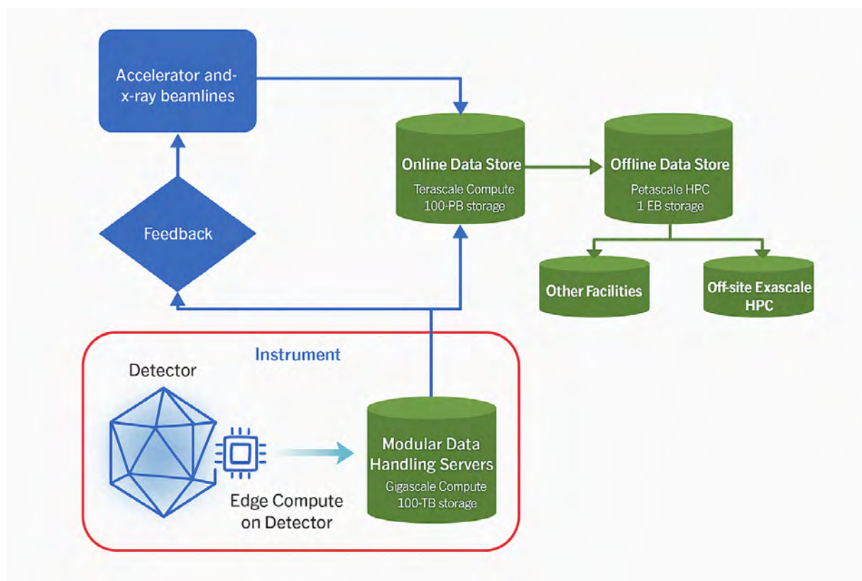
Figure 12.2: Proposed high-level data pipeline for the next-generation XFEL.
