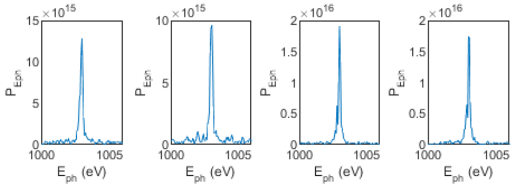
Figure 6.17: Self-Seeding Spectra at median position of maximum 6D brightness.
