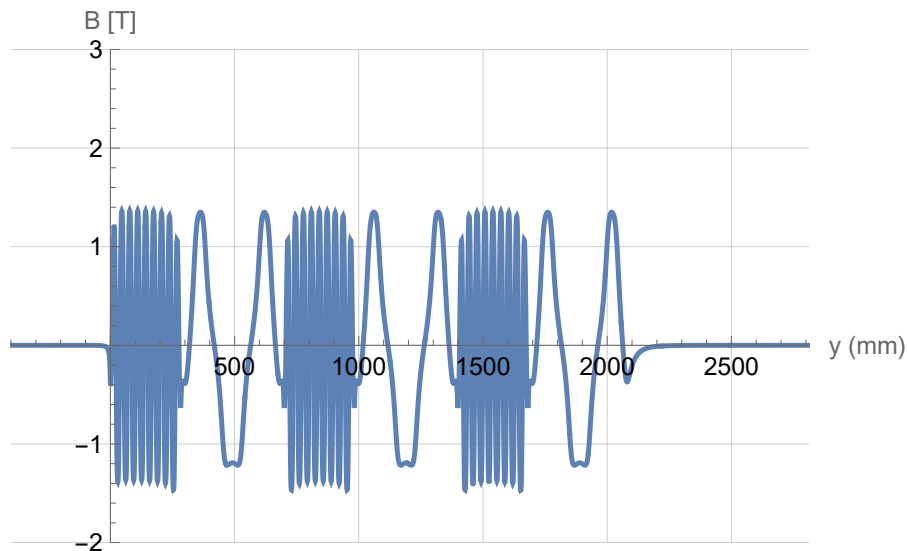
Figure 6.37: Modelled magnetic field of the Integrated Delay Undulator
