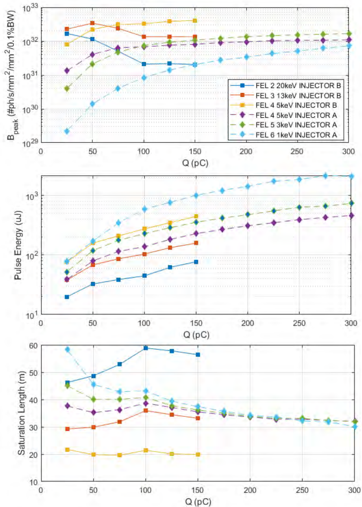
Figure 6.13: Optimisation of Bunch Charge
