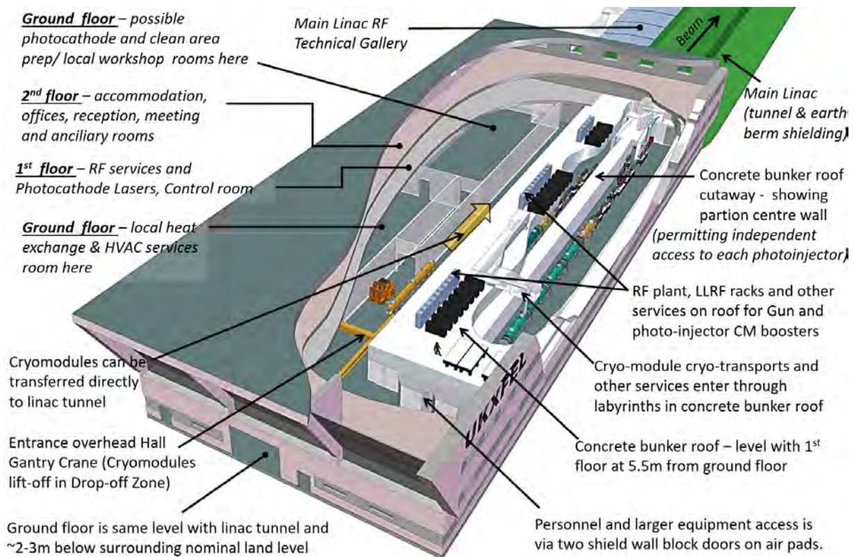
Figure 13.7: Injector Hall Building - 3D cutaway view with floors and shielding bunker cut to show dual Photoinjectors
