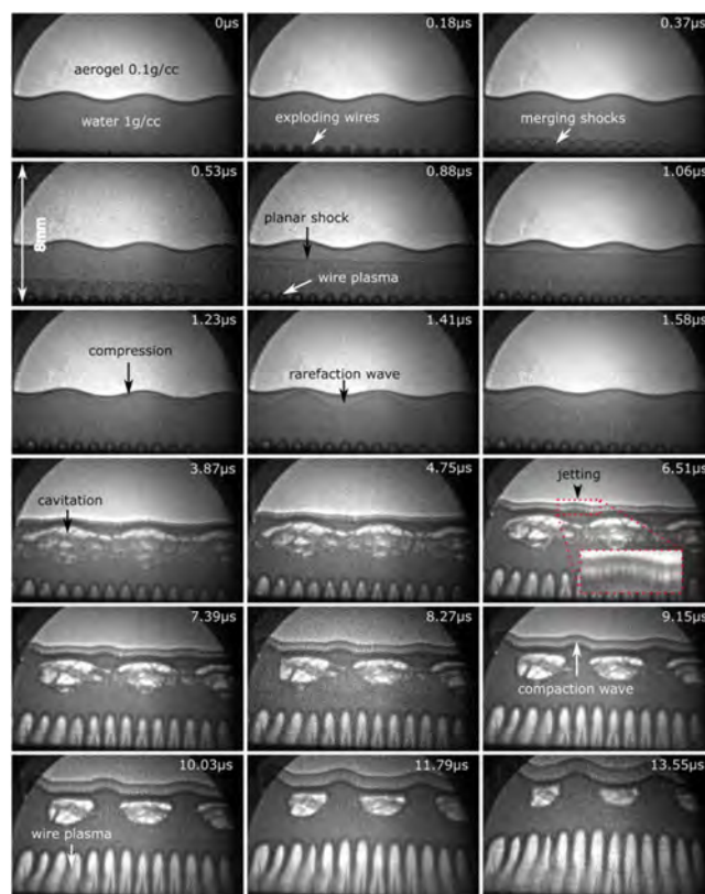
Figure 8.24: Multi-frame hard X-ray ( \bar{E} \sim 30 keV) radiography showing a Richtmyer-Meshkov instability driven by exploding wire arrays, conducted on ID19 at the ESRF. Figure adapted from J. Strucka et al. Physics of Fluids 35 044108 (2023). Reproduced under terms of the Creative Commons Attribution License 3.0 BY.
