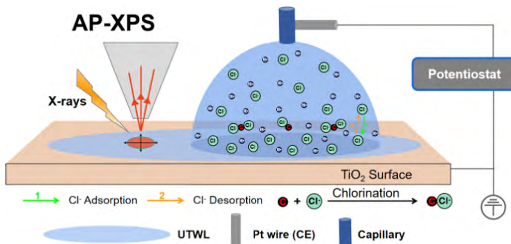
Figure 8.8: Experimental set-up for ambient pressure X-ray PES to investigate the effect of applied potential on the interface of \text{TiO}_2(110) with 0.1 M HCl, as performed on the VerSoX end-station at B07 on the Diamond Light Source. Ambient pressure operation (13 mbar) with in-operando electrochemical characterisation, enabled real-time monitoring and analysis of electrochemical processes. Figure reproduced from J. Yu et al. J. Phys. Chem. C 128 , 49, 20933-20939 (2024). Reproduced under terms of the Creative Commons Attribution License 3.0 BY
