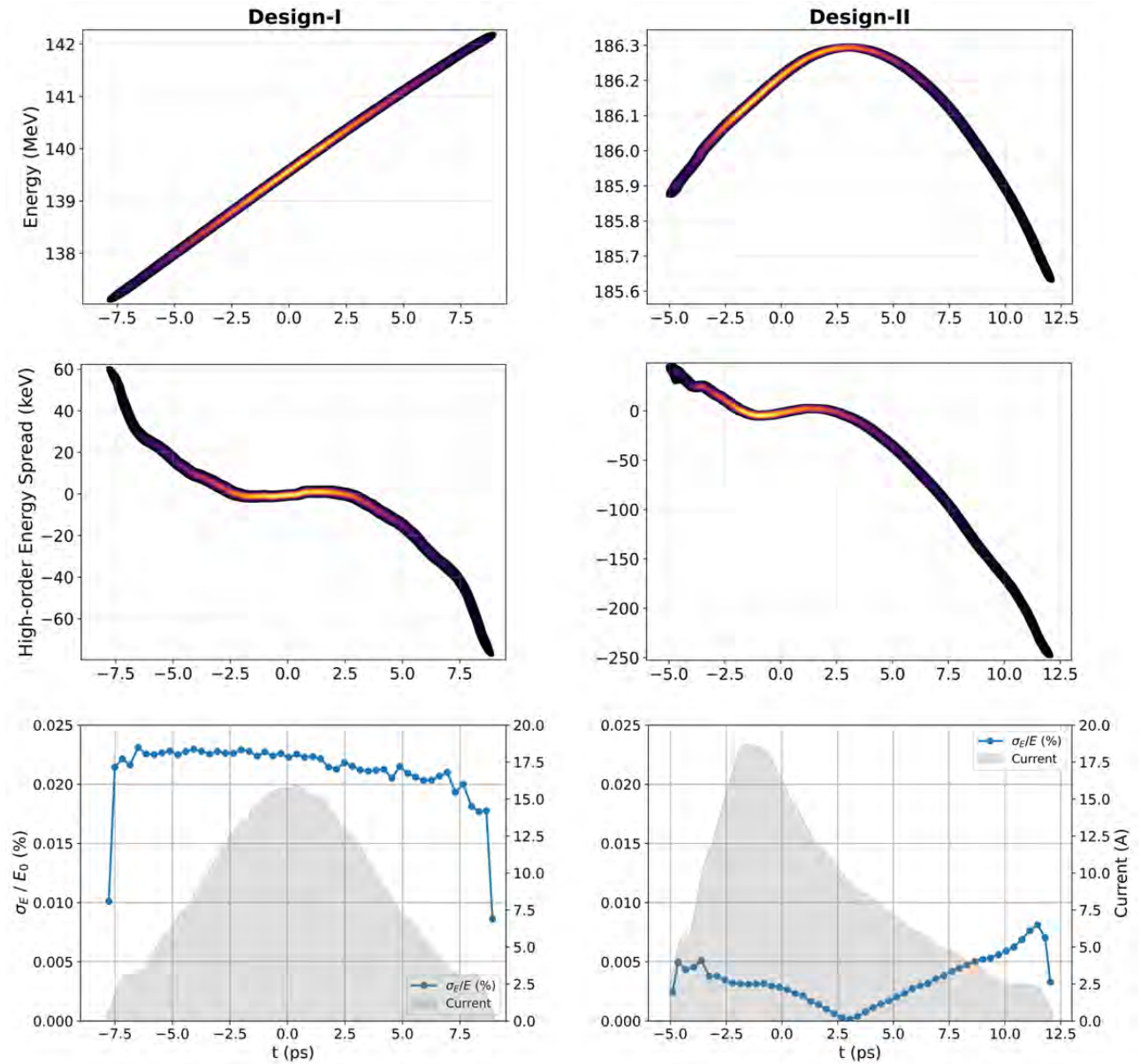
Figure 4.10: Comparison of longitudinal beam dynamics for Design-I and Design-II in terms of bunch energy, high-order energy spread, slice energy spread and current profile.
