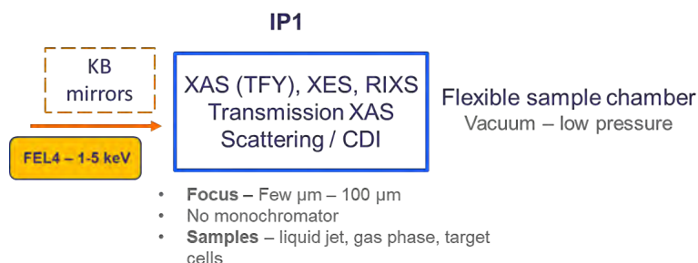
Figure 8.13: Configuration for ES6 featuring soft-tender X-ray photon spectroscopy methods.
