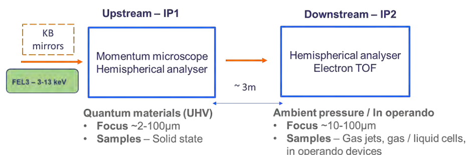
Figure 8.9: The ES8 (HAXPES) end station configuration on FEL-3 with two interaction points for differing sample environments.
