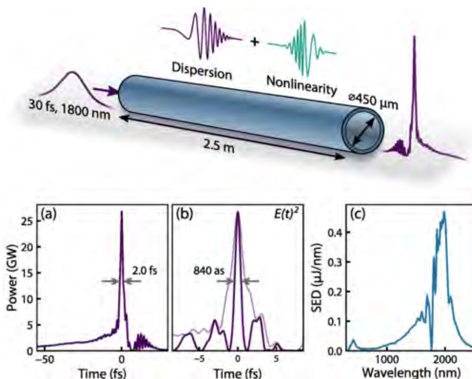
Figure 9.9: Example RDW pulse replicated from [18]. Self-compression to infrared attosecond pulses. Laser pulses at 1800 nm central wavelength with a duration of 30 fs at FWHM are coupled into a 2.5 m long gas-filled HCF with an inner diameter of 450 \mu\text{m} . In the HCF, the combination of anomalous dispersion arising from the waveguide and positive nonlinearity provided by the gas leads to self-compression of the pulses. With an argon pressure of 470 mbar and an initial pulse energy of 289 \mu\text{J} , the pulse at the HCF exit has an envelope duration of 2 fs at FWHM (a), which corresponds to an 840 as field transient (b). The spectrum of this pulse extends from the ultraviolet (400 nm) to the mid-infrared (2550 nm) (c).
