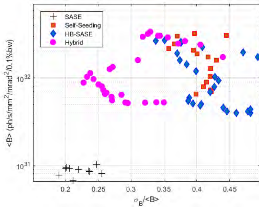
Figure 6.24: Mean Peak Brightness vs rms Brightness variation for the four schemes. Each plot point represents a different distance along the undulator, showing how the balance between brightness and stability changes during the FEL interaction process from start up through exponential growth to post-saturation.
