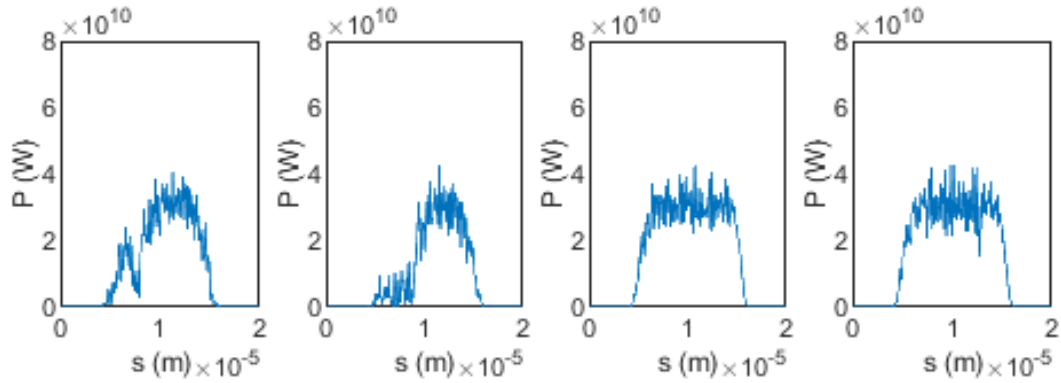
Figure 6.21: Self-Seeding pulses at median position of maximum 6D brightness.
