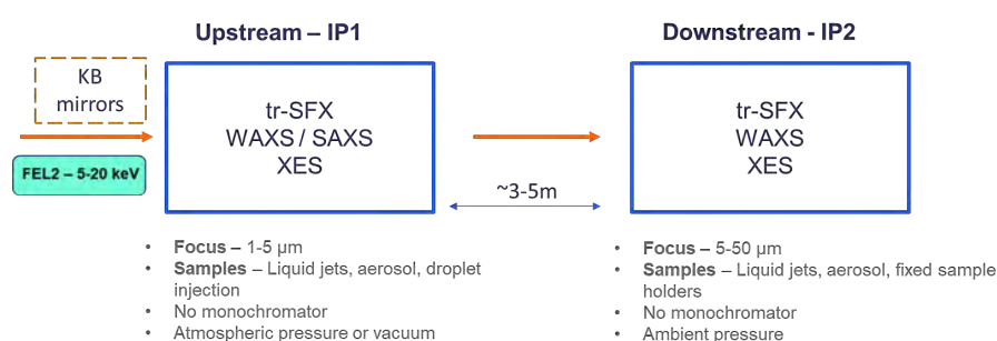
Figure 8.19: ES10 end station for application of tr-SFX techniques
