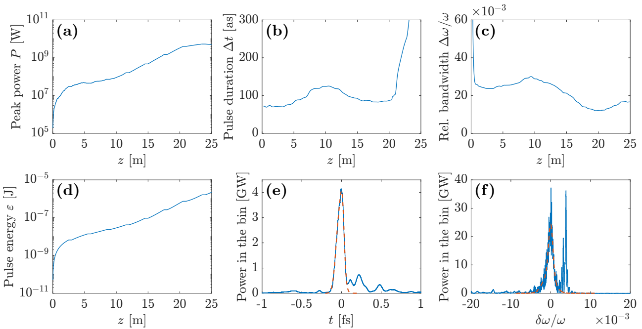
Figure 6.28: Simulation of photon pulse production in the ESASE scheme for the selected UK XFEL case. The (a) peak power, (b) pulse duration, (c) relative bandwidth and (d) pulse energy are shown as functions of the distance z along the second undulator section. Saturation occurs at z = 20 m, for which the (e) temporal and (f) spectral profiles are shown with an additional red dashed curve indicating a Gaussian fit to the principal spike.
