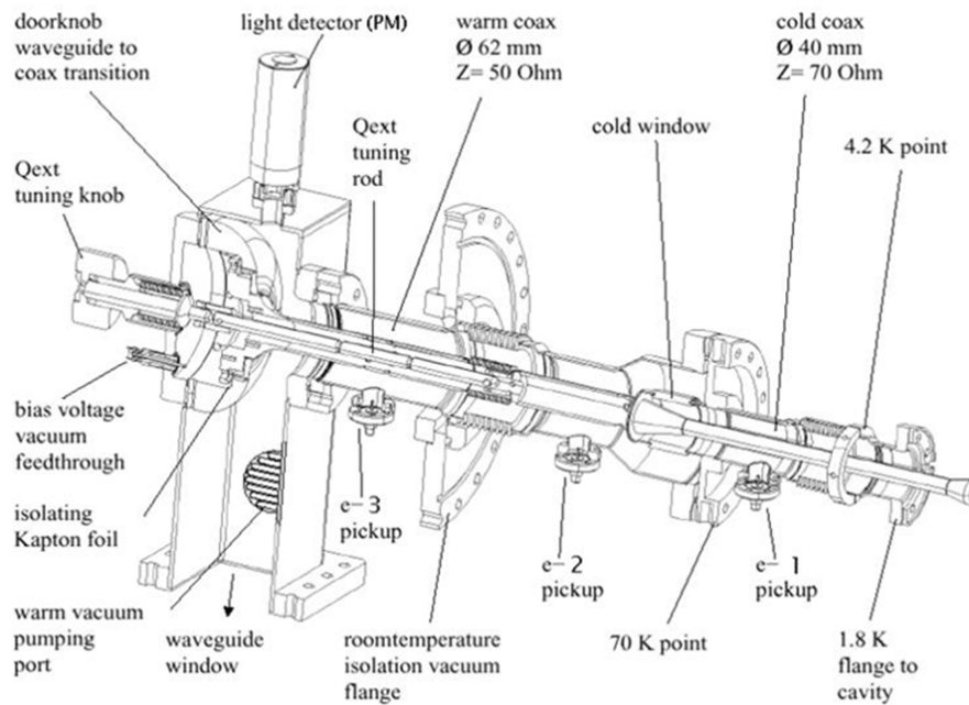
Figure 5.8: TTF-III coupler
