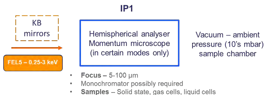
Figure 8.7: Configuration for ES5 end station for time-resolved APPES on FEL-5
