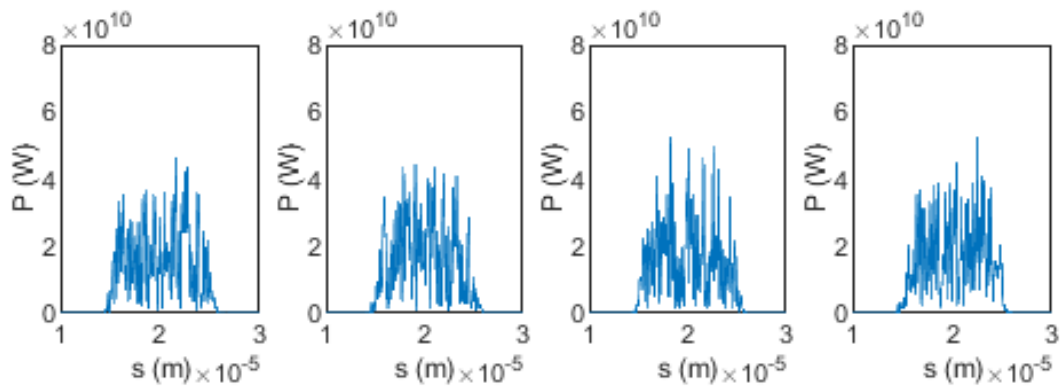
Figure 6.20: SASE pulses at median position of maximum 6D brightness.
