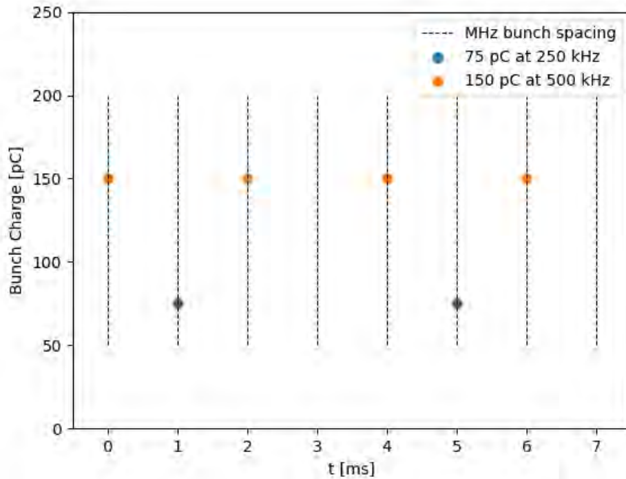
Figure 5.12: The proposed fill pattern of the 150 & 75 pC composite beam with a repeat pattern at 1 MHz of "150 - 75 - 150 - gap".
