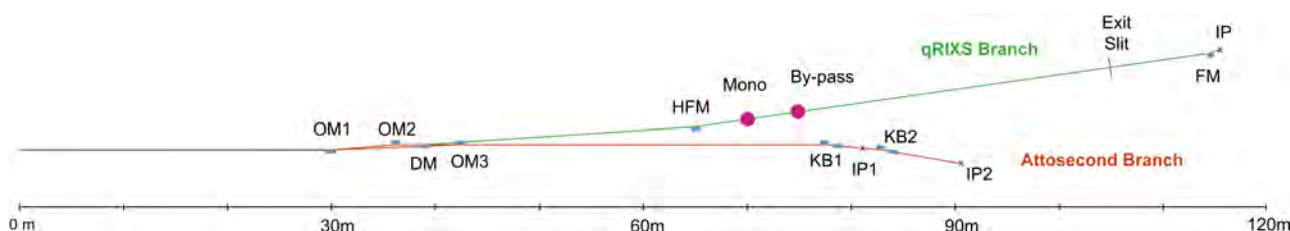
Figure 7.6: Overall optical layout of FEL-5 beamline with separate attosecond and qRIXS branches. OM = Offset mirror; DM = distribution mirror; HFM = horizontally focusing mirror; KB = Kirkpatrick-Baez mirror; FM = Focussing mirror; IP = interaction point
