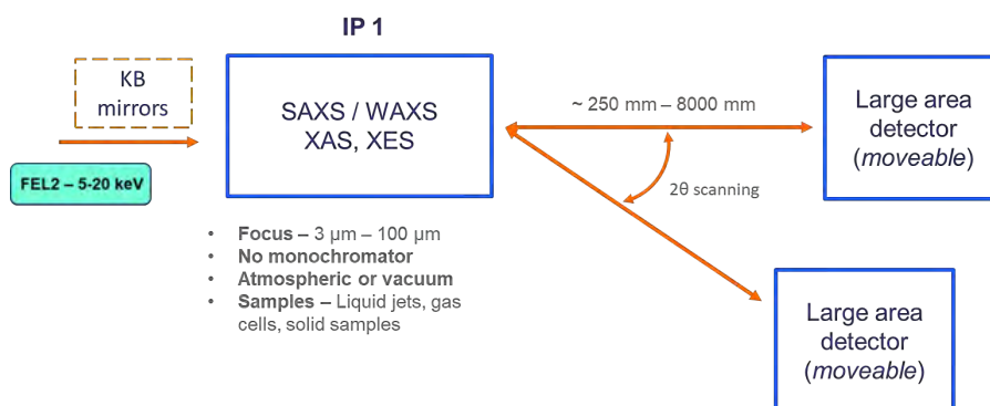
Figure 8.17: ES9 end station for coherent scattering techniques
