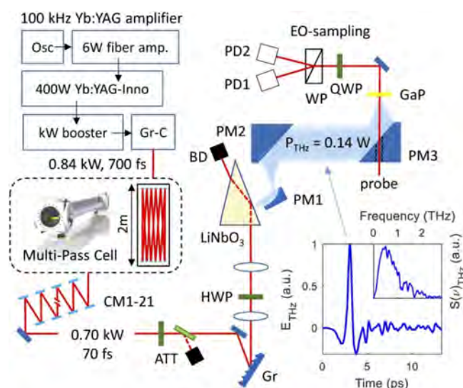
Figure 9.11: THz generation using lithium niobate at high repetition rate, as demonstrated (and reproduced from) [24].
