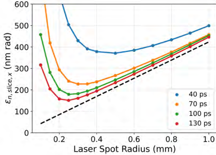
Figure 4.4: Average slice emittance of the three central slices of the 150 pC bunch generated with Cs 2 Te photocathode at the emittance compensation point after the gun, shown as a function of laser spot size and pulse duration for the relaxed gun geometry. Dashed line shows theoretical value of the emittance
