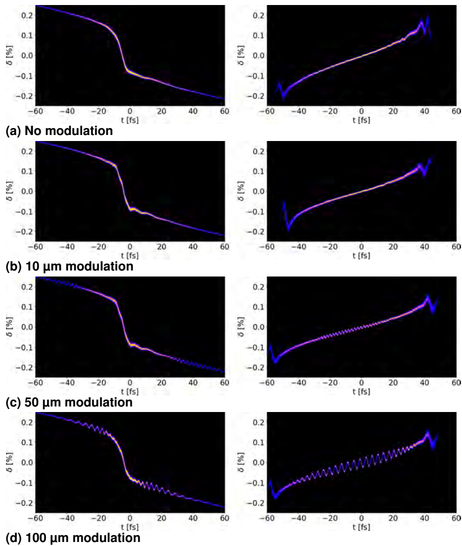
Figure 5.25: Longitudinal phase space of 300 pC electron bunch at the entrance of the FEL compressed by: arc (left) and five dipole chicane (right). The initial electron bunches had no initial density modulation (top/first), 10 \mu\text{m} initial density modulation (second), 50 \mu\text{m} initial density modulation (third), and 100 \mu\text{m} initial density modulation (fourth/bottom).
