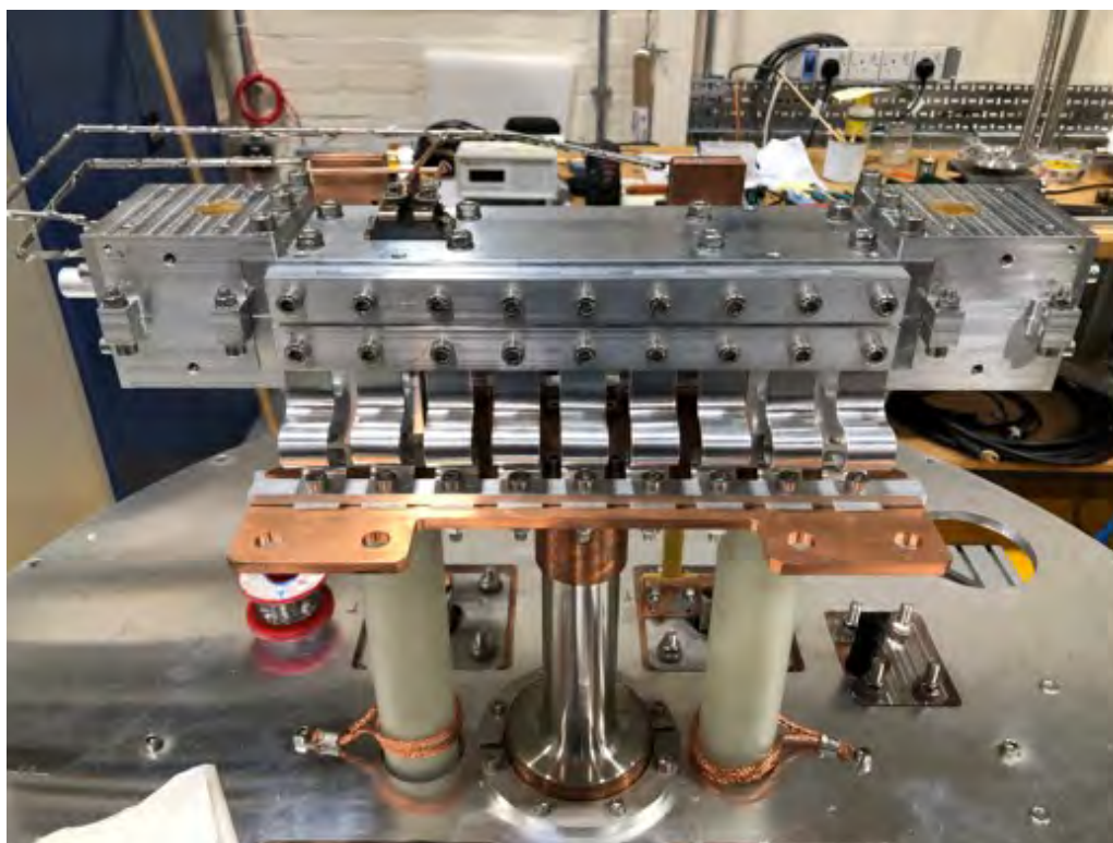
Figure 6.34: Test cryostat for the 325 mm prototype of the STFC helical SCU.
