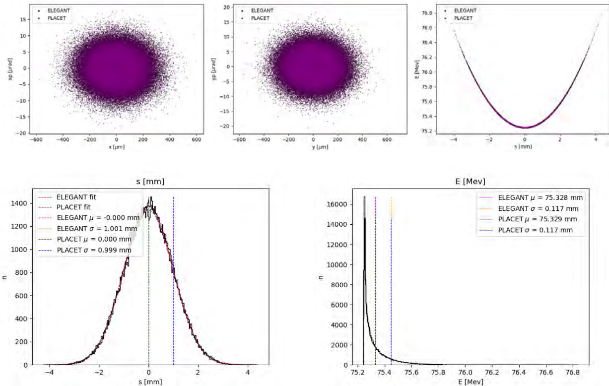
Figure 5.43: The diagnostic plots to verify parity between the ELEGANT and PLACET code bases, with ELEGANT shown in black and PLACET in purple for the 3 rd harmonic 3.9 GHz cavity with the bunch coinciding with the trough of the RF phase. Top left: Horizontal phase space. Top middle: Vertical phase space. Top right: Longitudinal phase space. Bottom left: Histogram of the longitudinal distribution of the bunch. Bottom right: Histogram of the energy distribution of the bunch.
