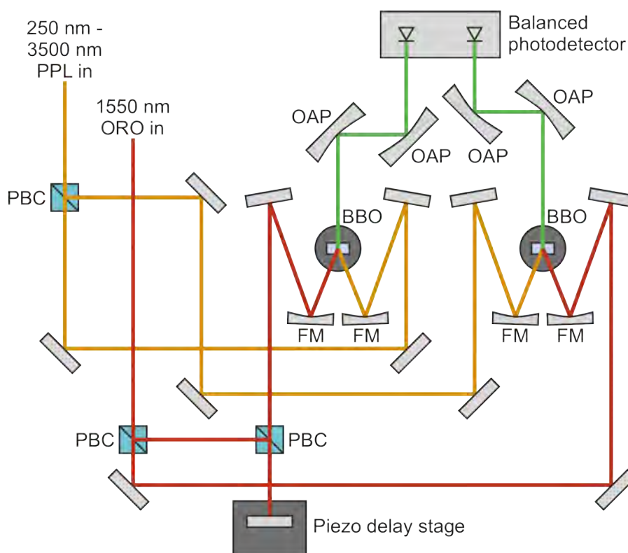
Figure 11.2: Layout of the non-collinear, two-crystal BOXC being developed at DESY for use as an all-colour LAM. PPL: Pump-probe laser; ORO: Optical reference oscillator; PBC: Polarising beamsplitter cube; FM: Focusing mirror; BBO: Barium borate non-linear crystal; OAP: Off-axis parabolic mirror. Figure printed with DESY permission.
