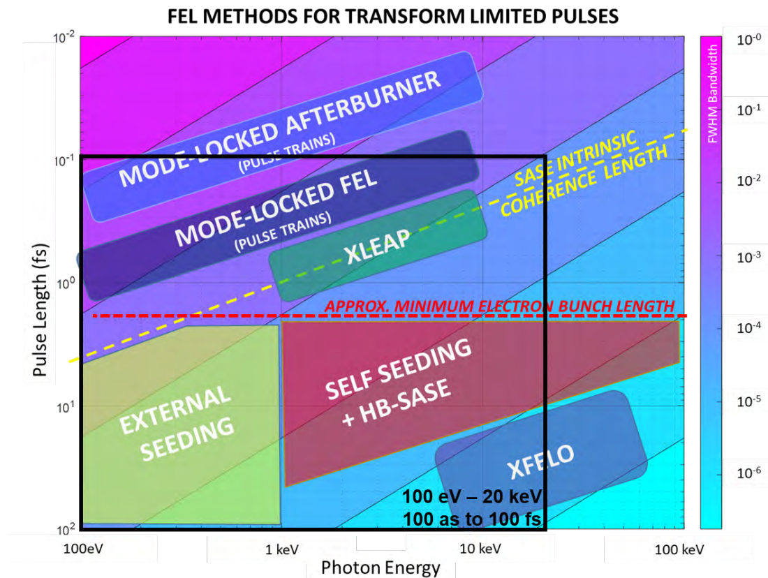
Figure 6.2: The estimated coverage of some relevant FEL techniques for the generation of near-transform-limited pulses. The project's aim for near-transform-limited pulses from 0.1 to 20 keV and 100 as to 100 fs is shown by the black box in the photon energy-pulse length parameter space.
