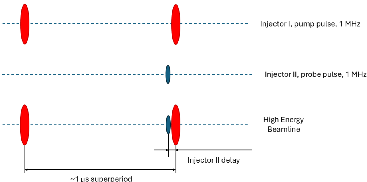
Figure 4.21: Operation of the two injector LEB in two colour mode.
