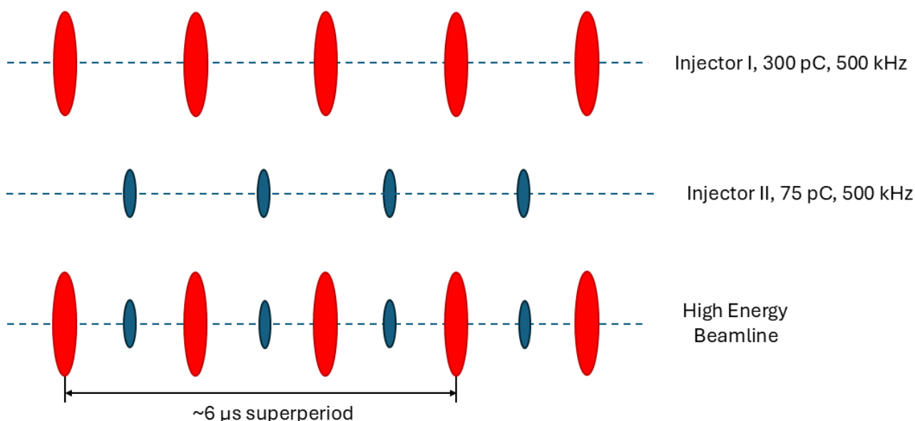
Figure 4.20: Example of two injector LEB operation in 6 FEL mode.
