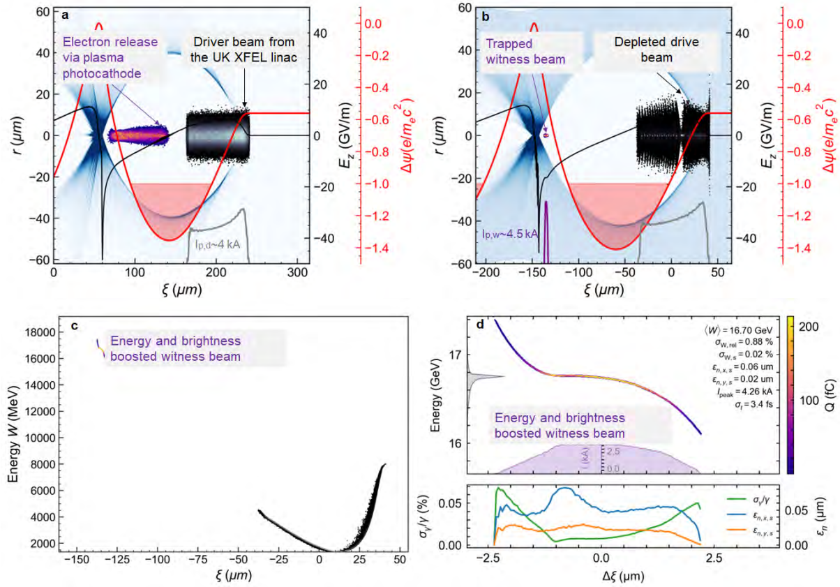
Figure 5.34: Plasma photocathode injection PWFA configuration at UK XFEL. An electron driver beam (grey) from the linac propagates through a one-meter-long PWFA stage filled with helium plasma (blue), generating a plasma wakefield (solid black line). (a) A trailing sub-mJ-class plasma photocathode injector laser pulse releases electrons directly inside the plasma blowout via tunnelling ionisation of helium ions. (b) These released cold electrons form a well-defined witness beam with nm-rad emittance and multi-kA peak current at the back of the wakefield. (c) The witness beam experiences phase-stable acceleration along the PWFA stage and overtakes the driver, reaching multi-GeV beam energy. (d) At the end of the plasma stage, an energy- and brightness-boosted witness beam with exceptional projected and slice beam properties is released into the vacuum.
