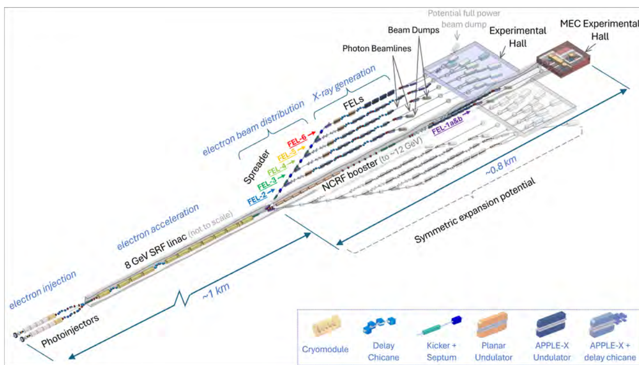
Figure 3.1: An outline of the conceptual design for a next-generation XFEL to meet the requirements of the Science and Technology Case. A repeating section of the SRF linac is omitted for clarity.
