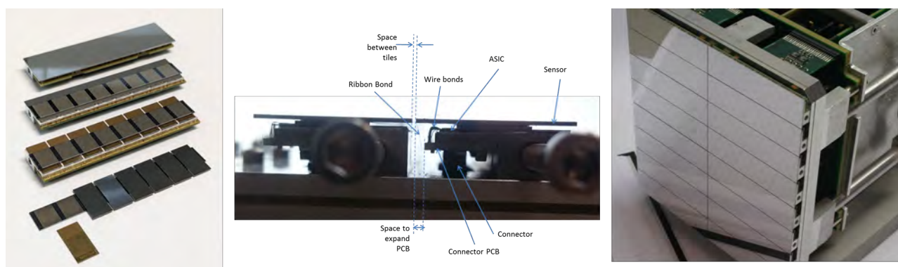
Figure 10.12: The LPD tile with interposer parts (left), side view of the tiled modules (middle) and a tiled array (right). Credit: Matthew, reproduced under terms of the Creative Commons Attribution License 2.0
