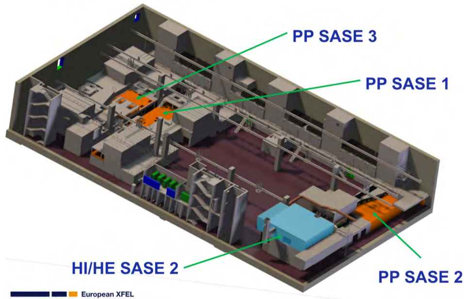
Figure 9.4: Location of the pump-probe laser systems at European XFEL [8]
