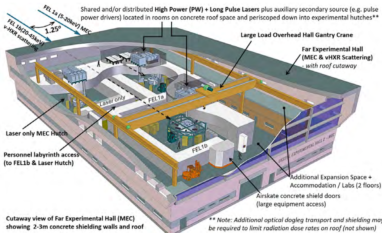
Figure 13.17: 3D Isometric Elevation and Cutaway of MEC Far Experimental Hall
