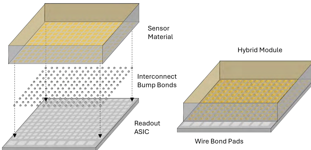
Figure 10.2: Illustration of a hybrid detector module.
