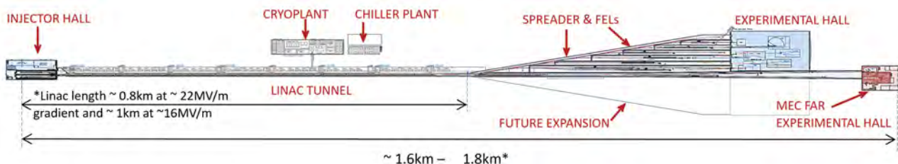
Figure 13.1: Scaled Plan View Full Layout of UK XFEL concept
