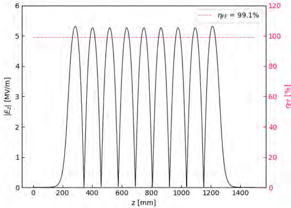
Figure 5.40: The on-axis z component of the electric field of the main accelerating TM_{010} \pi mode of the TESLA 9-cell cavity, with \eta_{ff} = 99.1\% .
