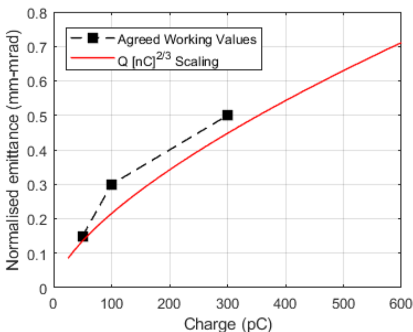
Figure 6.12: Emittance vs Charge scaling.
