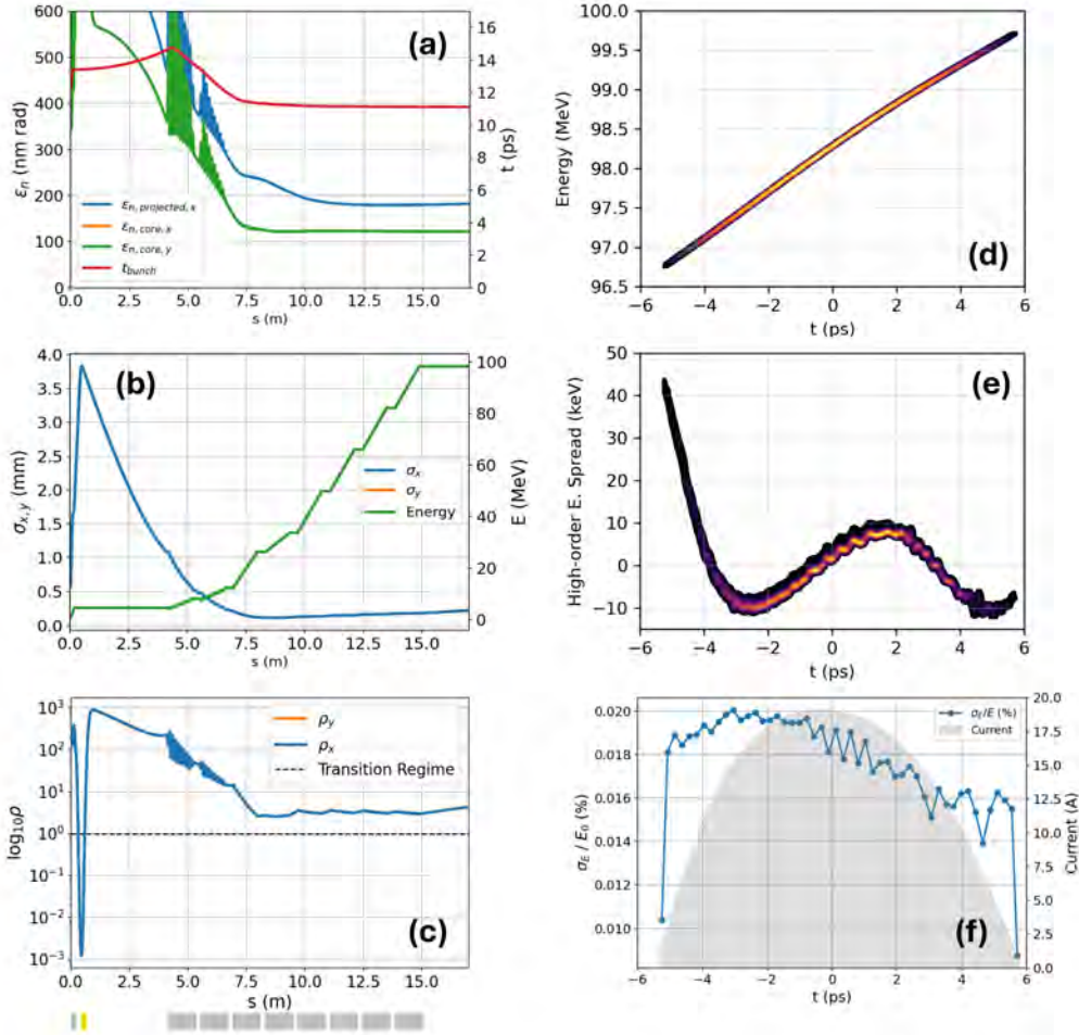
Figure 4.17: Left column: Evolution of beam parameters along the injector beamline for the L-band injector design at 150 pC bunch charge, (a) normalized projected and core emittances (horizontal and vertical) and bunch duration, (b) RMS transverse beam size and mean kinetic energy, (c) laminarity parameter. Right column: Longitudinal beam properties, (d) energy, (e) high-order energy spread, (f) slice energy spread and current profile.
