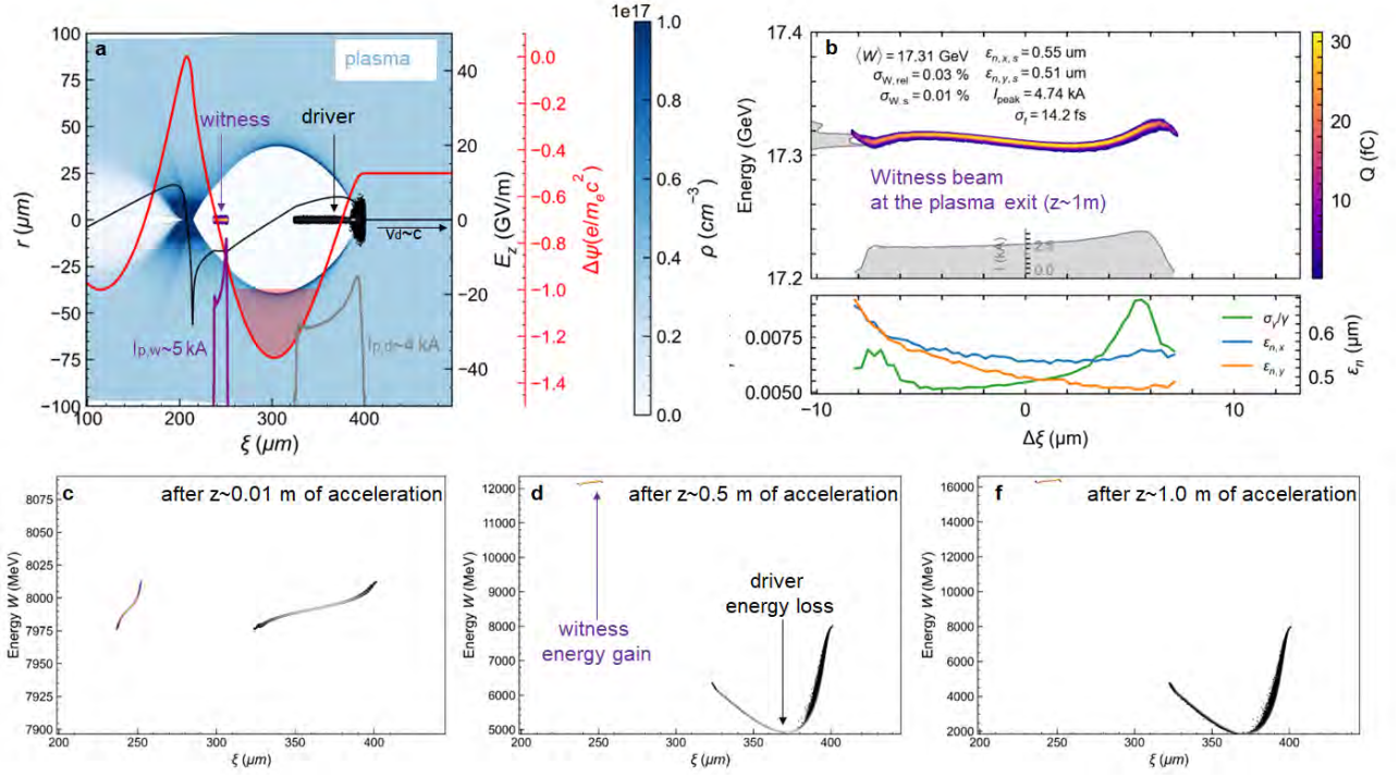
Figure 5.33: Double-bunch PWFA configuration at UK XFEL. (a) An electron driver beam (grey) from the linac propagates through a 1 m long PWFA stage filled with helium plasma (blue), generating a plasma wakefield (solid black line). A trailing witness beam (purple), positioned at the accelerating phase of the wakefield, experiences energy gain. Evolution of the longitudinal phase spaces of both driver and witness beams along the plasma stage length is depicted in the bottom plots (c-f), illustrating the driver beam deceleration and the witness beam acceleration to 17 GeV energy. The resulting witness beam longitudinal phase space and corresponding slice properties at the exit of the plasma stage are shown in panel (b).
