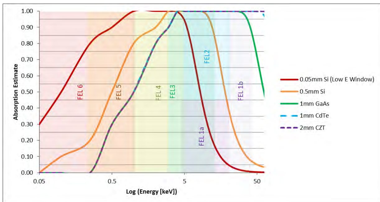
Figure 3.18: Sensor material X-ray stopping power with energy relating to the FEL energies.
