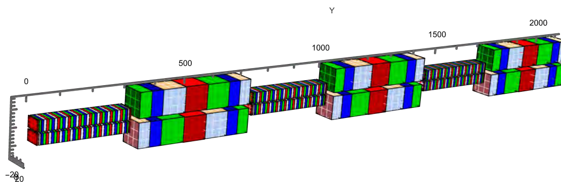
Figure 6.36: RADIA Model of a 2 m long Integrated Delay Undulator
