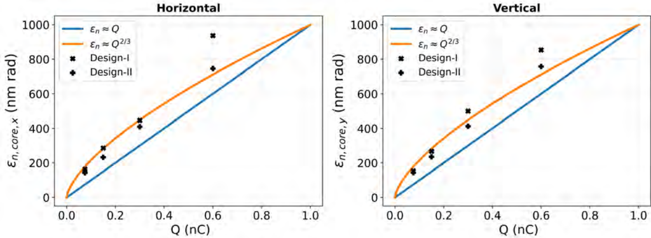
Figure 3.7: Final horizontal and vertical core emittances for the VHF-gun-based injectors Design-I (baseline choice) and Design-II across all simulated bunch charges. Emittance values generally show good agreement with the theoretical scaling law assumed in FEL modelling (orange lines).
