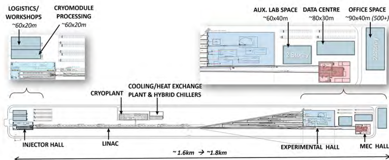
Figure 13.19: Showing Entire ~2 Km site with ancillary buildings highlighted
