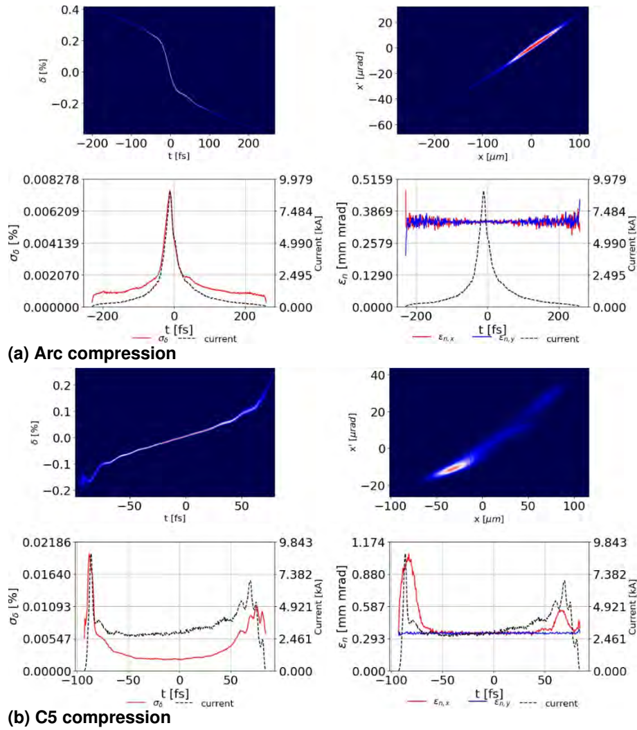
Figure 5.24: Final bunch properties at the exit of the linac for arc (top) and C5 (bottom) 300 pC compressed bunches. Each subfigure contains: Longitudinal phase space; Horizontal phase space; Slice energy spread and peak current; transverse emittances and peak current.
