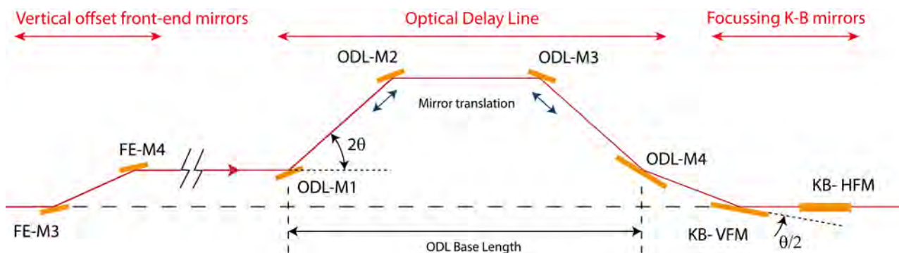
Figure 7.12: Schema showing a 4-mirror optical delay line integrated into the overall scheme for FEL-5 beamline
