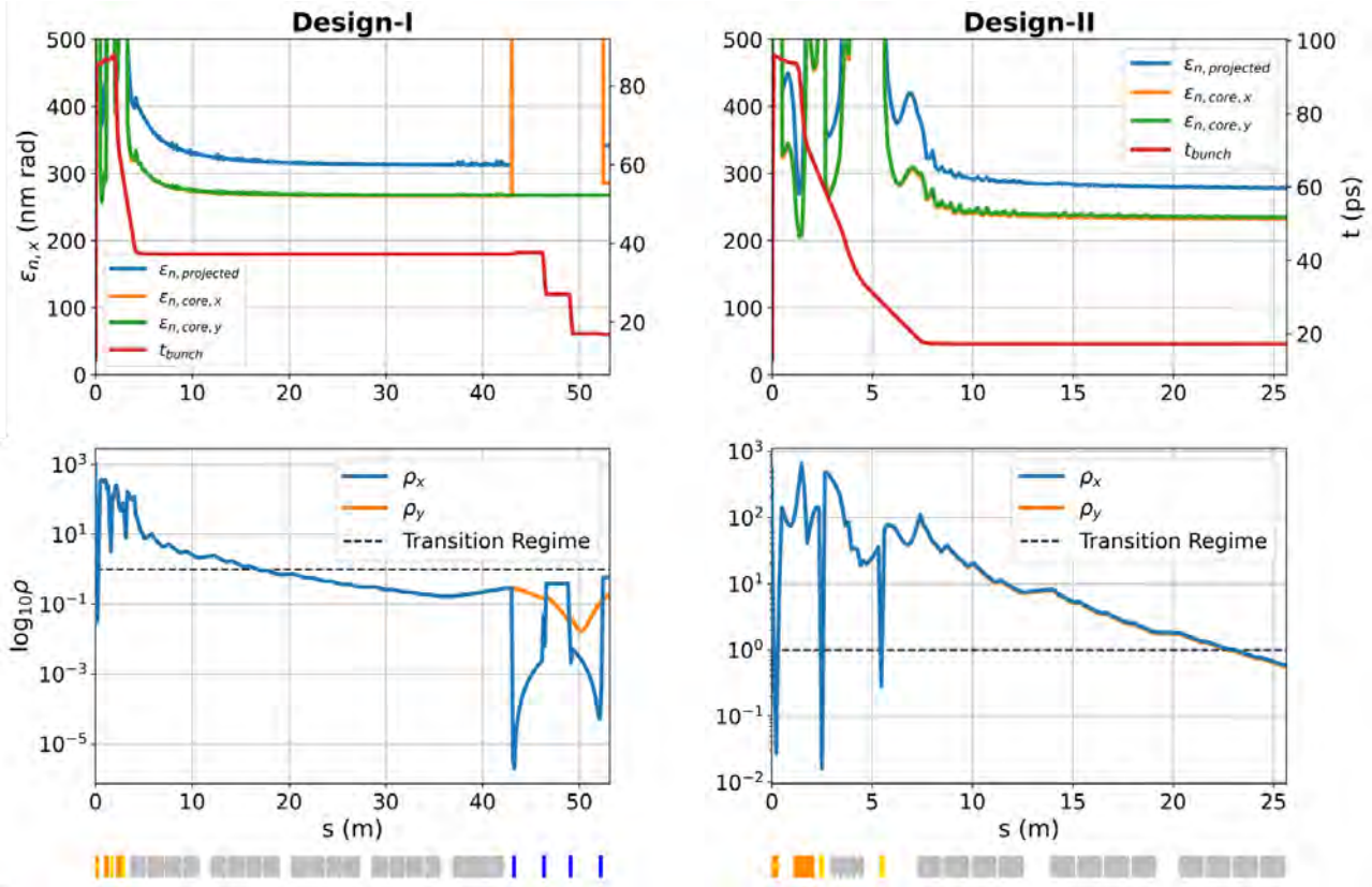
Figure 4.9: Evolution of normalized projected and core emittances (horizontal and vertical), bunch duration, and laminarity parameter along the injector beamline for Design-I and Design-II at 150 pC bunch charge. The plots illustrate compression stages, emittance compensation, and the transition from space charge-dominated to emittance-dominated regimes. The laminarity parameter confirms that both configurations achieve emittance-dominated transport by the injector exit, suitable for main linac injection.
