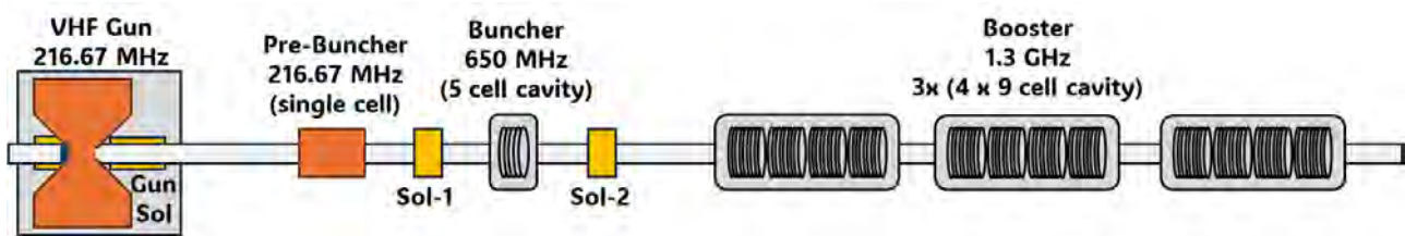
Figure 4.7: Low Energy Beamline layout for Design-II.
