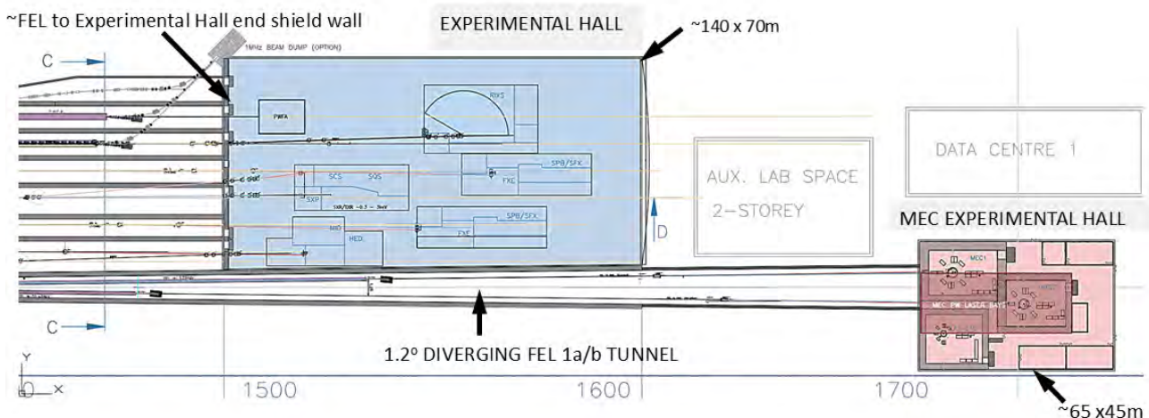
Figure 3.16: Experimental halls layout (spanning from \sim 1.4 km to 1.8 km). Three end station hutches can be accommodated per FEL line, with these clusters of end stations staggered relative to each other to minimise the transverse deflection required in the spreader
