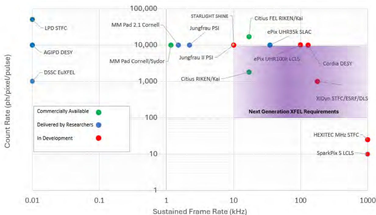
Figure 10.9: Summary of the integrating X-ray detector readout ASICs with commercially available (green), fully developed detector systems (blue) and new ASIC in development (red). *Any ASIC developments not included here is not an indication of their merit or importance, but this variety was most easily accessible to the authors.
