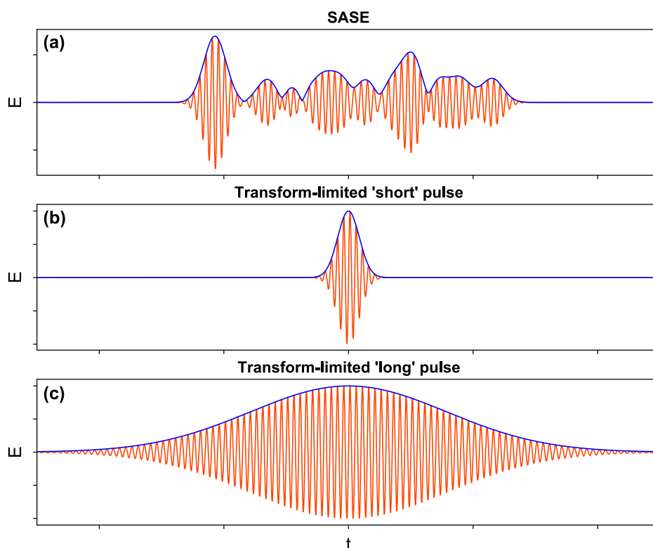
Figure 2.7: Indicative comparison between the temporal profile of (a) a SASE pulse (top) and two pulses that are transform-limited: (b) a 'short' pulse with duration similar to a single SASE spike, and (c) a 'long' pulse with duration similar to the full SASE pulse.
