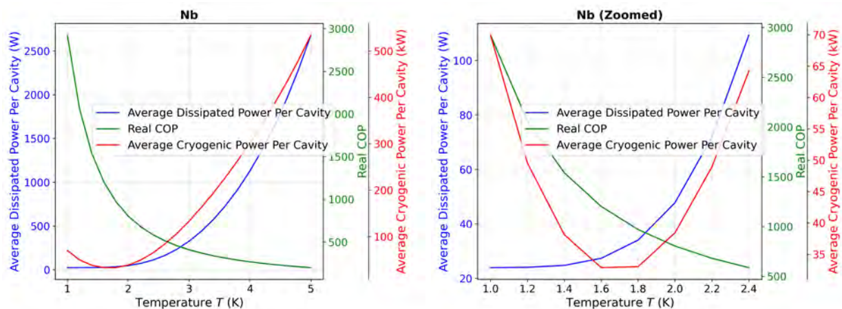
Figure 5.5: Normal-scale (left) and magnified (right) plots as functions of temperature, showing the average dissipated power per cavity (blue), the real coefficient of performance (COP) (green), and the average cryogenic power per cavity (red), for bulk Nb cavities.
