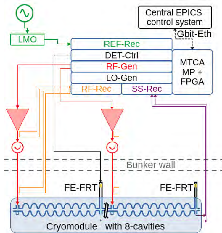
Figure 5.19: Block diagram of proposed unit LLRF system.
