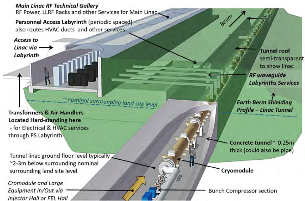
Figure 13.9: Linac Tunnel & RF services gallery – 3D cutaway visualisation of option A
