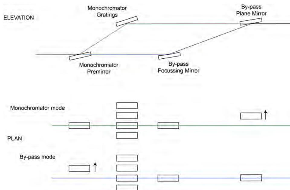
Figure 7.10: Schema showing how a by-pass might be implemented in the qRIXS monochromator. In monochromator mode, the second by-pass mirror is moved out of the beam path. In by-pass mode, the monochromator is moved sideways to allow the beam to pass the premirror.
