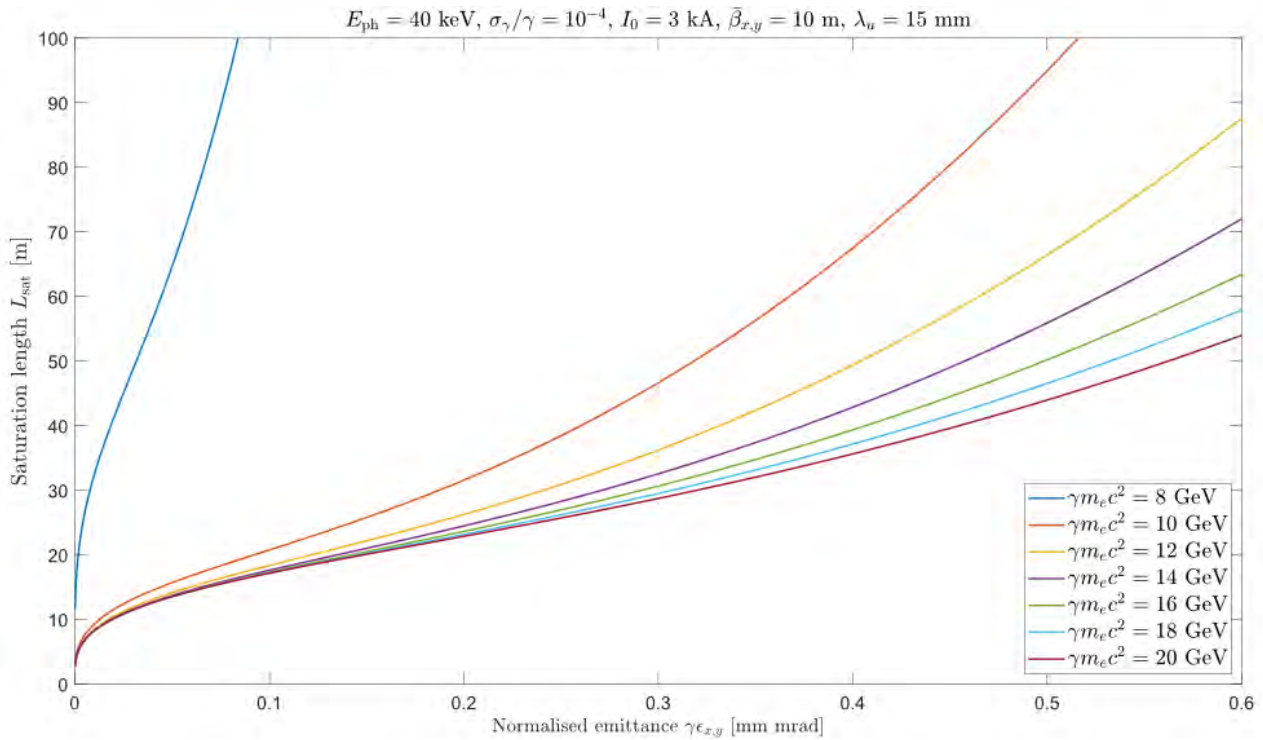
Figure 4.24: Plot of saturation length as a function of beam energy and emittance, for a photon energy of 40 keV.
