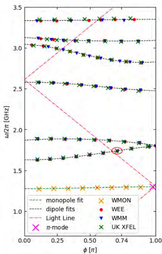
Figure 5.42: The Brillouin diagram showing the dispersion curves of the first six dipole passbands and the equivalent modes from the Wanzenberg DESY study [31]. Here, "WEE" and "WMM" refer to the Wanzenberg study with electric-electric and magnetic-magnetic boundaries in the beampipes, respectively. Also included are the first nine monopole modes (WMON) with the main accelerating \pi -mode highlights in magenta. The red circle highlights dipole mode 7, the off-axis E_z profile of which is shown in Figure 5.41
