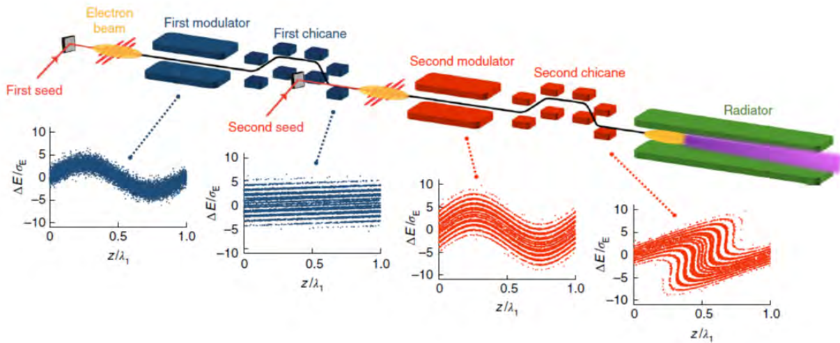
Figure 6.3: Schematic of Echo-Enabled Harmonic Generation (EEHG) scheme. There are two modulator undulators, in which lasers modulate the energy-time phase space of the electron bunch, as shown, to generate microbunching at a high harmonic of the laser. The bunches propagate into a radiator undulator which is tuned to be resonant at this higher harmonic. Figure reproduced from [6].
