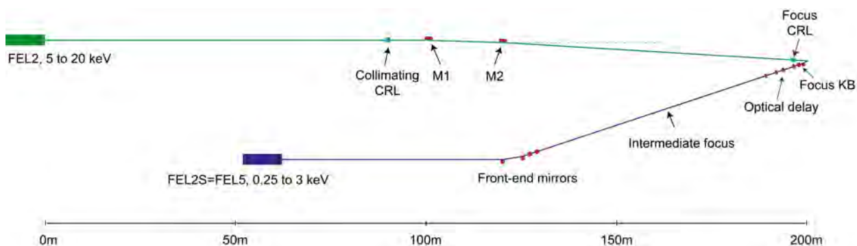
Figure 7.11: Layout of beamlines combining output of FEL-2 and its associated soft x-ray FEL (equivalent to FEL-5) to a common interaction point.
