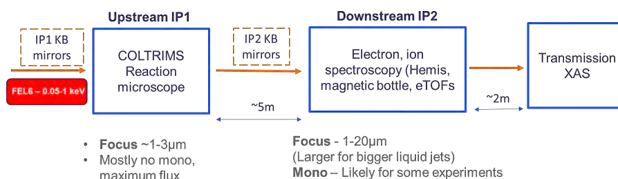
Figure 8.2: Planned configuration for ES1 for AMO experiments on FEL-6 using soft X-ray energies (0.05 - 1 keV)
