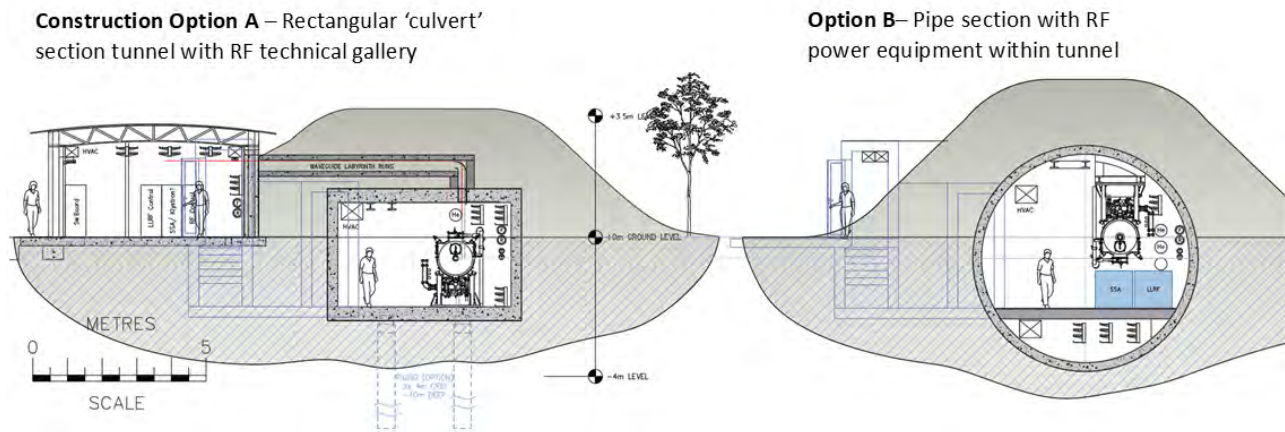
Figure 13.8: Cross section for cut and cover construction options for Linac Hall
