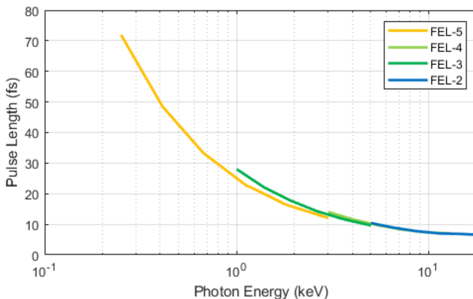
Figure 6.11: Required Electron Bunch Lengths for HB-SASE Transform Limited Operation
