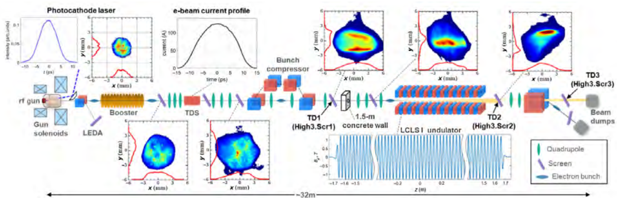
Figure 9.16: Replicated from [38]: PITZ machine layout (not to scale). The beam travels from the rf gun through the booster, electron beam transport beamline, bunch compressor, the LCLS-I undulator, and THz diagnostic sections. The photocathode laser, electron beam transverse distributions, and temporal profiles measured along the beamline are shown as insets close to locations of measurement. The measured magnetic field of the LCLS-I undulator is shown as well.
