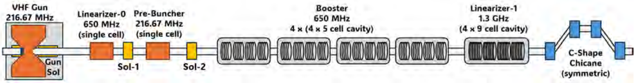
Figure 4.5: Low Energy Beamline layout for Design-I.
