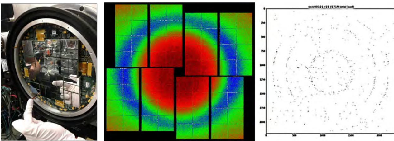
Figure 10.6: An ePix10k2M detector array (left), a typical diffraction pattern with water ring features (middle), and a map of bad pixels on a Jungfrau 4M detector due to radiation damage with the pattern corresponding to the water ring pattern. Credit: Conny Hansson
