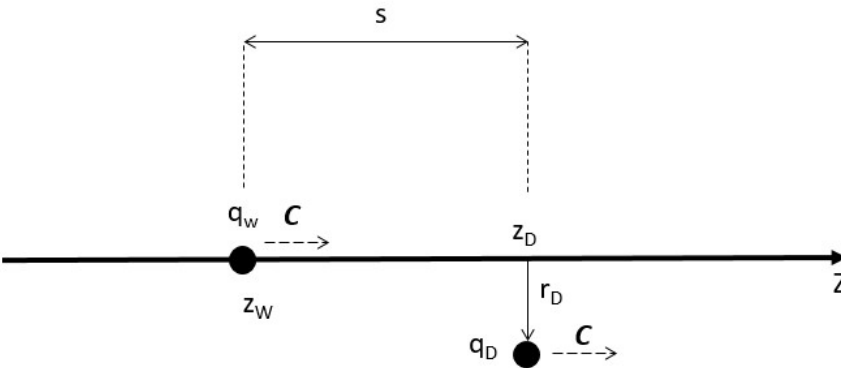
Figure 5.14: An illustration of the situation used to benchmark PLACET's handling of LR transverse wakes to the analytical solution outlined in Equation 5.18.
