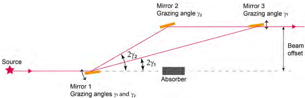
Figure 7.7: Three-mirror system for offset mirrors allowing two grazing angles and a fixed exit beam axis. Mirror 3 moves out of the beam when Mirror 2 is in use.
