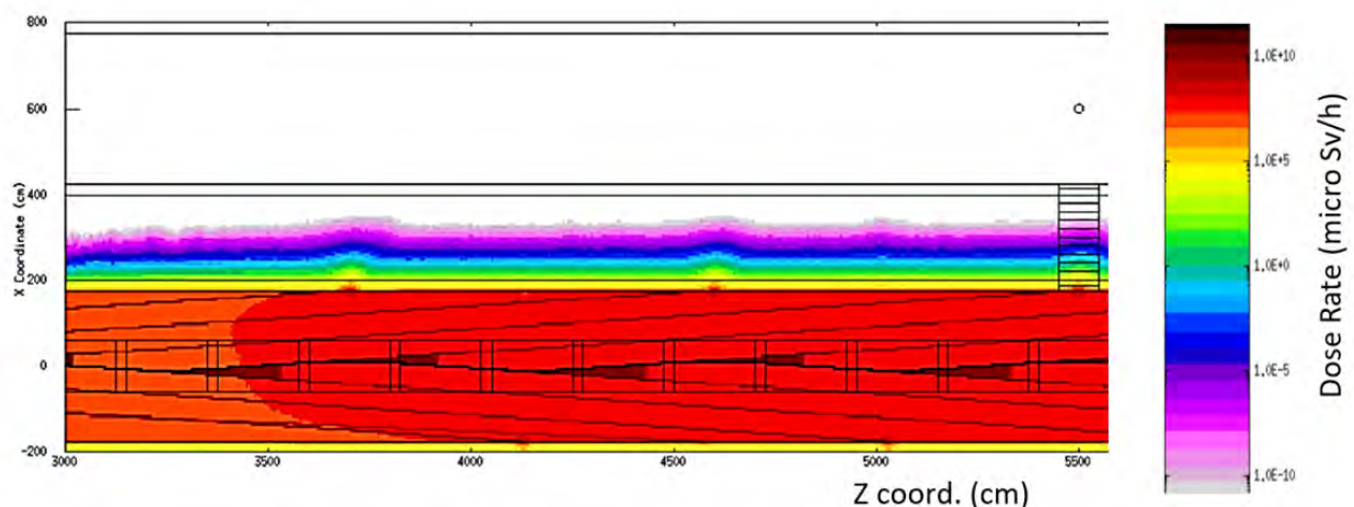
Figure 13.21: Plan view dose rates contour plot during normal operation from Synchrotron Radiation.
