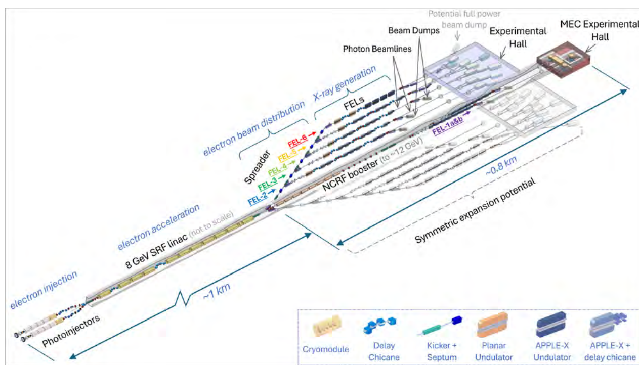
Figure 1.2: An outline of the conceptual design for a next-generation XFEL providing a unique combination of capabilities to meet the requirements of the Science and Technology Case.
