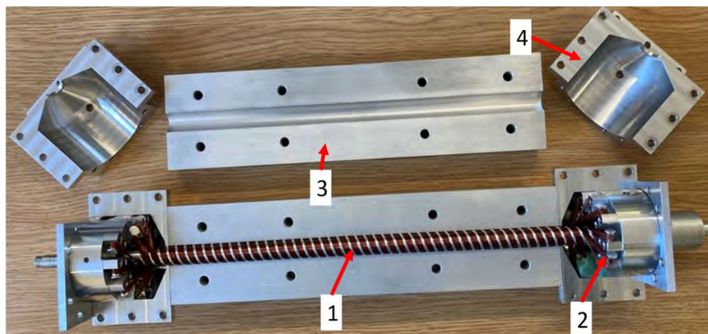
Wound 325 mm HSCU in strong back; 1- Wound HSCU former, 2- Turnaround pins, 3-Potting jig strong back, 4- Potting jig turnaround section.
