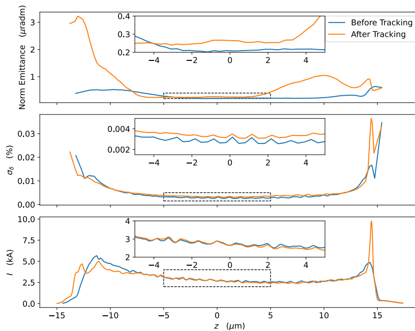
Figure 5.32: The slice normalised horizontal emittance (top), slice energy spread (centre) and current profile (bottom) of the bunch before (blue) and after (orange) tracking to the end of the spreader line to FEL-6. Each plot shows a zoomed-in region to make it easier to read the values at the core of the bunch.
