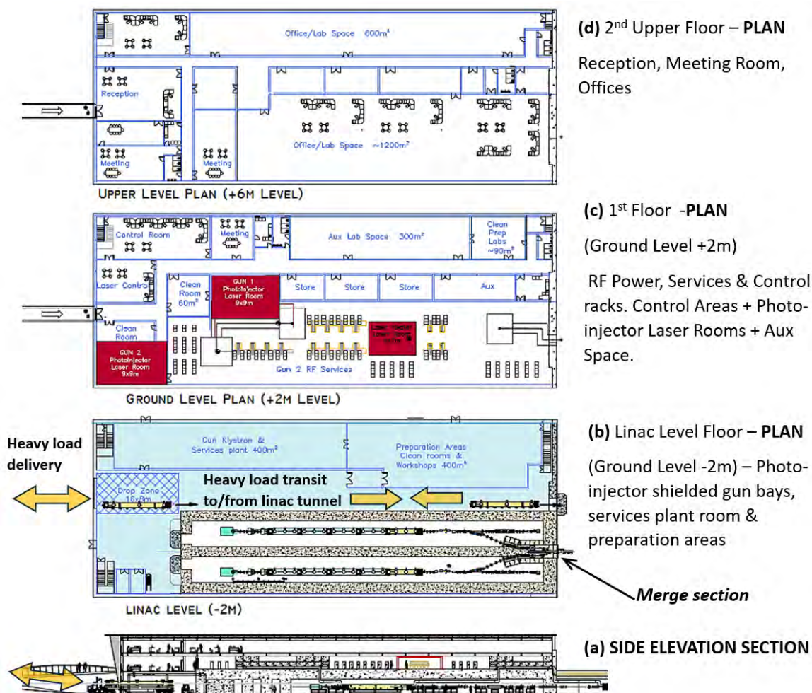
Figure 13.6: Photoinjector Hall showing 90 × 35 m plan of 3 levels plus side elevation view
