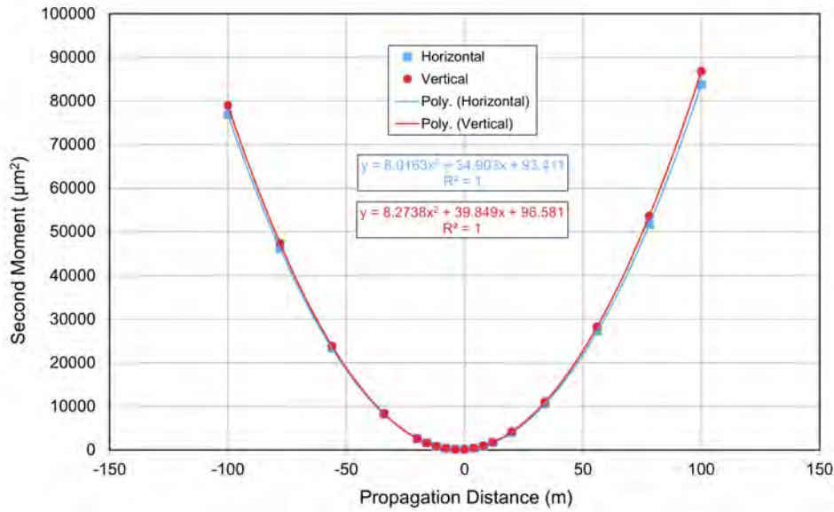
Figure 7.1: M^2 analysis for simulated output of FEL-2 at 5 keV. The abscissa is the propagation distance in metres from the Genesis output file. The ordinate is the second moment of the horizontal and vertical beam profile. Perfect quadratic fits are achieved, confirming the validity of the M^2 theory. The beam is actually close to Gaussian in this case with an average M^2 of 1.04.
