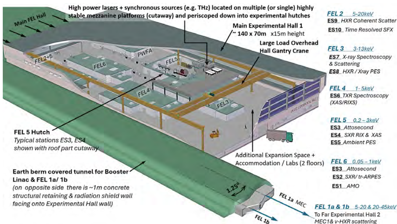
Figure 13.14: 3D Isometric Elevation & Cutaway of Main Experimental Hall
