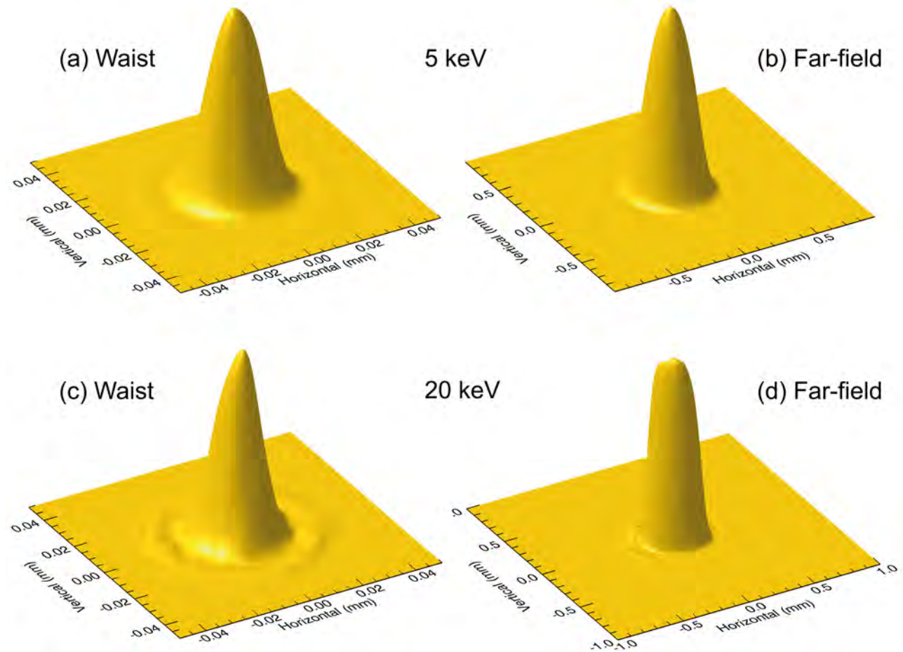
Figure 7.2: Results of the FOCUS wavefront propagations for FEL-2 Genesis simulations at 5 and 20 keV. The 3D plots show the spatial distribution of beam intensity on a linear scale. In (a) and (c) the propagation is back to the average longitudinal position of the horizontal and vertical waists, as determined from the M^2 analysis. We interpret this as the photon source for beamline modelling. In (b) and (d) the propagation is 100 m forward from the location of the Genesis file, representing the far-field beam profile. At 5 keV M^2 = 1.04 and the beam is close to Gaussian. At 20 keV, M^2 = 1.47 and the deviation from Gaussian is obvious.
