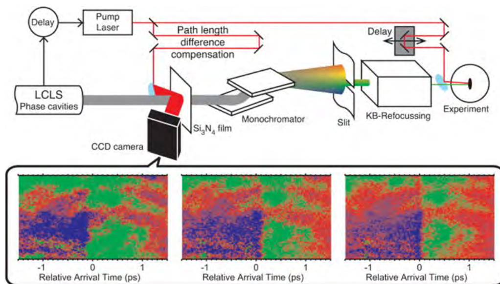
Figure 11.5: Experimental setup of spatial encoding at LCLS, as presented in [52]. The LCLS beam (grey) impinges on a thin \text{Si}_3\text{N}_4 film prior to travelling through the monochromator. An optical reference was derived using a pick-off of the laser pulse directed to the experiment IP, with suitable path length matching. Typical camera images of the optical laser reflected from the film after background subtraction are shown at the bottom. The relative arrival time jitter is mapped onto a spatial coordinate on the camera (here already converted to time).
