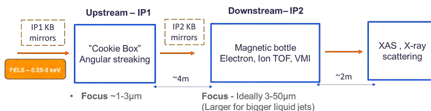
Figure 8.4: Planned configuration for ES3 for experiments on FEL-5 for ultra-short pulse (attosecond) soft x-ray experiments
