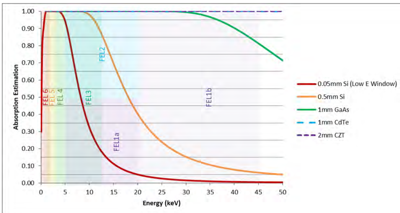
Figure 10.3: Sensor material X-ray stopping power with energy relating to the FEL energies.
