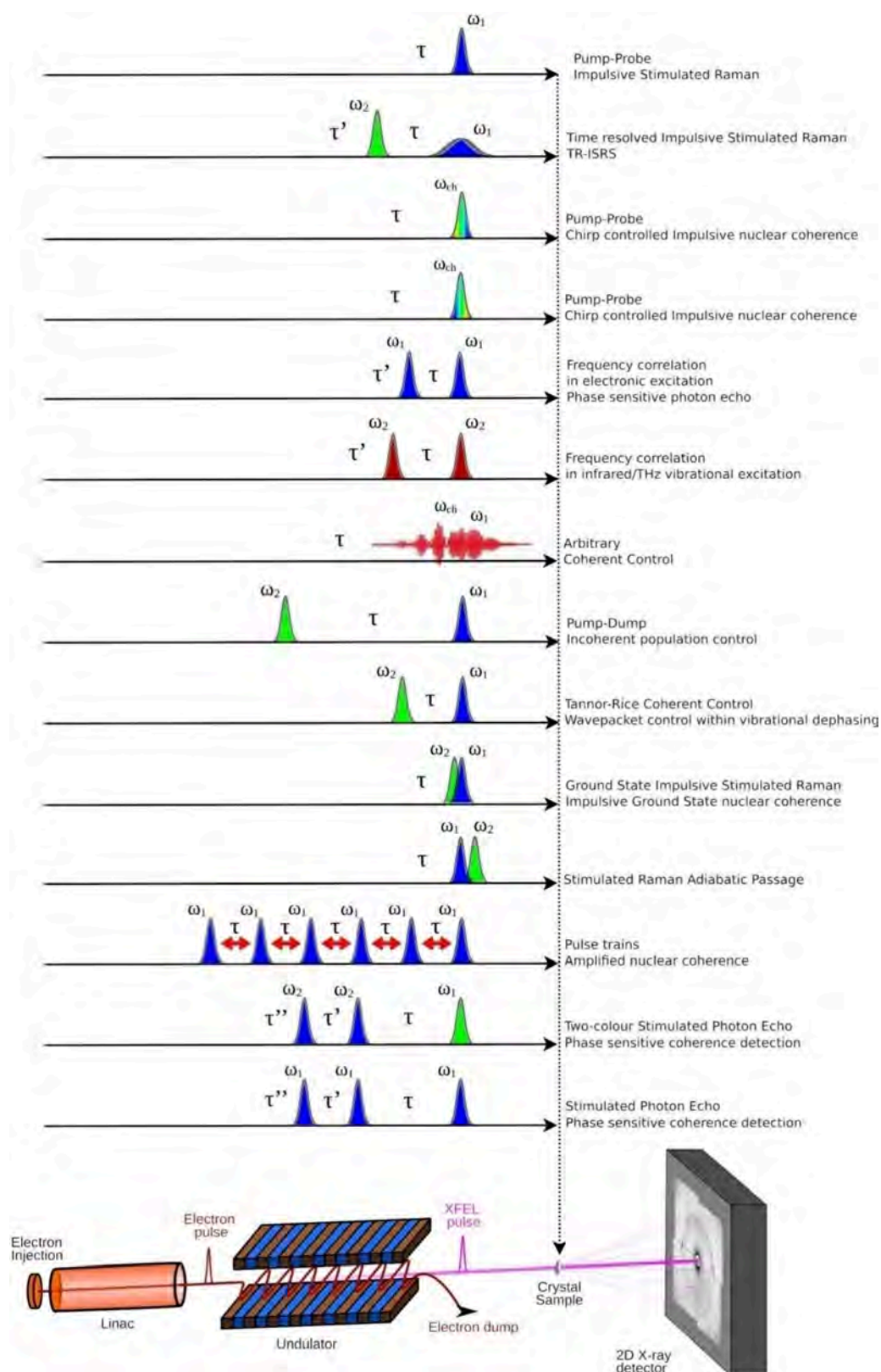
Figure 9.2: Overview of proposed pulse schemes for ultrafast hard X-ray diffraction. Reproduced from [1] under terms of the Creative Commons Attribution License 3.0 BY.
