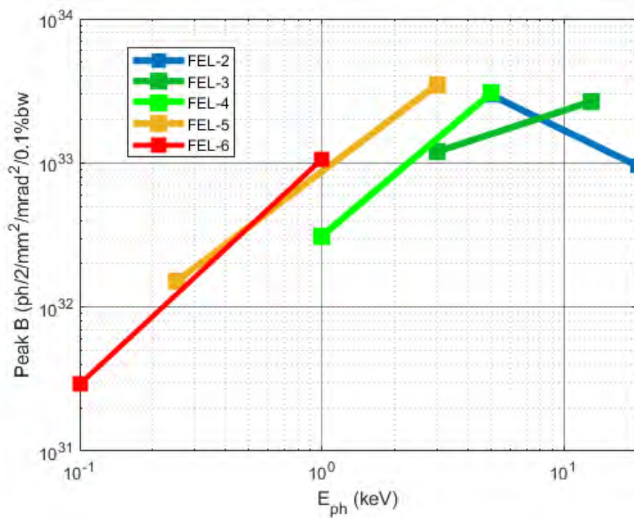
Figure 6.30: Predicted peak brightness in long pulse transform-limited mode.
