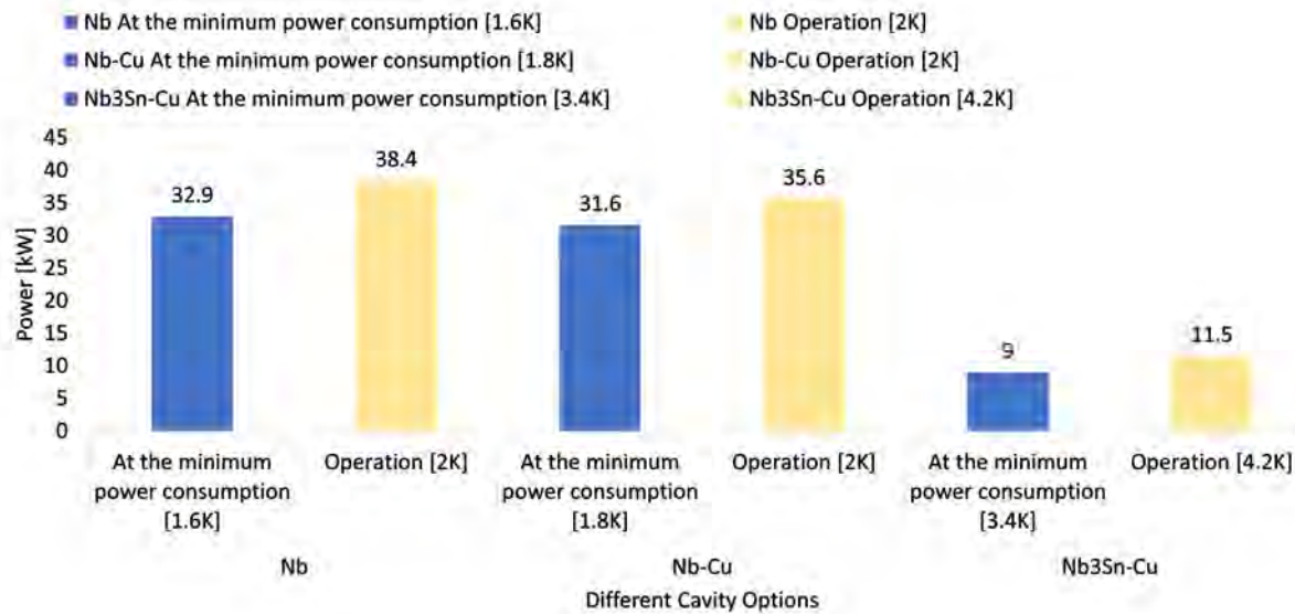
Figure 5.4: Graphical comparison of cryogenic power demand per cavity [kW] for different cavity types, evaluated at the temperature [K] corresponding to the minimum cryogenic load (blue) and at an operationally feasible temperature (yellow).
