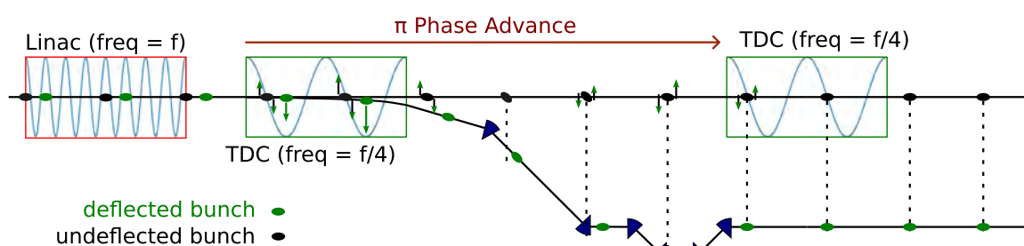
Figure 5.29: The “double bunch” at various point during its passage through the spreader to FELs 2 and 2b. Shown are: the phases that the bunches must enter the linac and the TDC cavities, how a bunch entering the TDC at the zero crossing affects the head tail tilt and how the the transverse offset of the dogleg and VPLA chicane is used to synchronise the two bunches.
