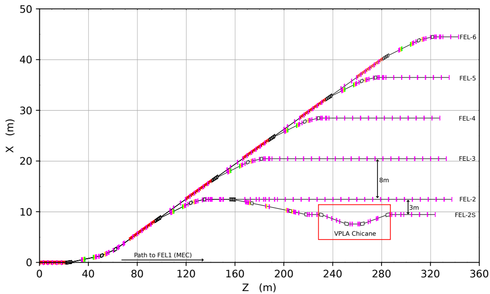
Figure 5.27: Diagonal wedge spreader layout.
