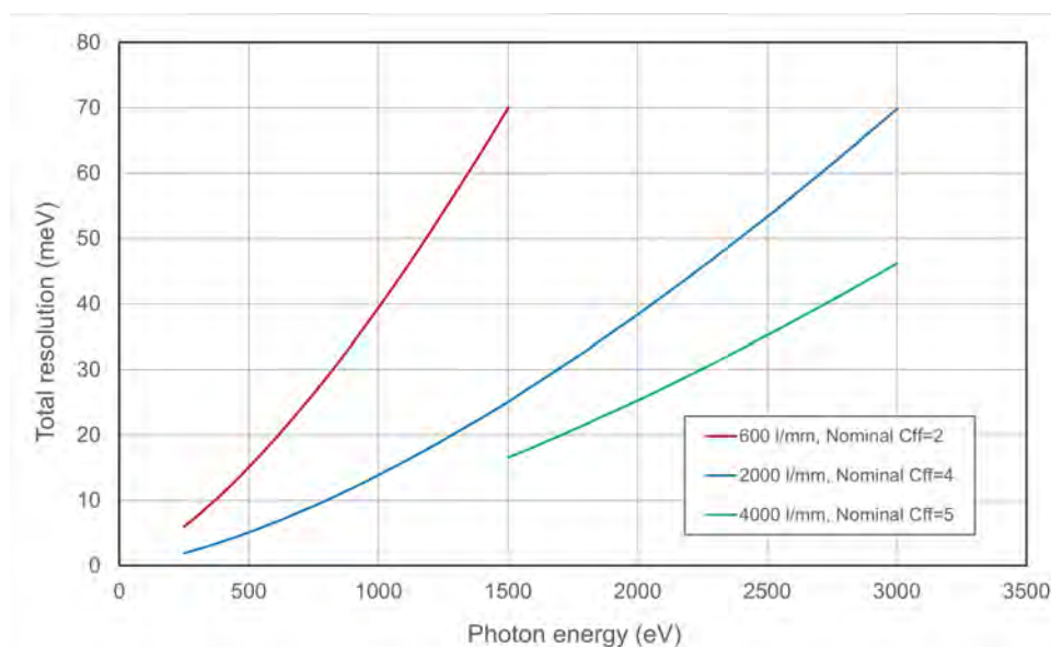
Figure 7.8: Calculated total monochromator resolution for three gratings (600, 2000 and 4000 l/mm) covering the FEL tuning range. The nominal C_{ff} values for each grating are 2, 4 and 5 (note actual C_{ff} changes slightly to keep the monochromator in focus). Grating and premirror slope errors are 100 nrad and 150 nrad RMS respectively. Exit slit is 10 \mu m. Entrance arm is 70 m and exit arm is 35 m. Resolution is the vector sum of source size, exit slit, and grating and premirror slope error contributions. Defocus, coma and spherical aberration are assumed nulled by the appropriate VLS terms. Any other contribution is ignored.
