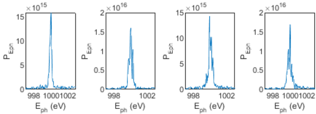
Figure 6.18: HB-SASE Spectra at median position of maximum 6D brightness.
