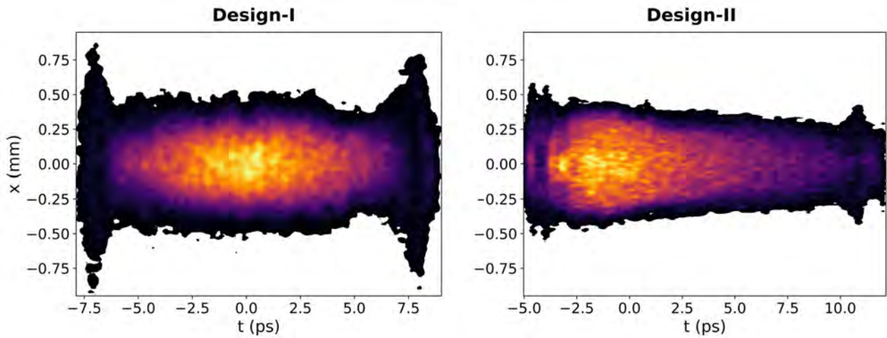
Figure 4.12: Current density projection of the electron bunch in the horizontal-longitudinal plane for Design-I and Design-II.
