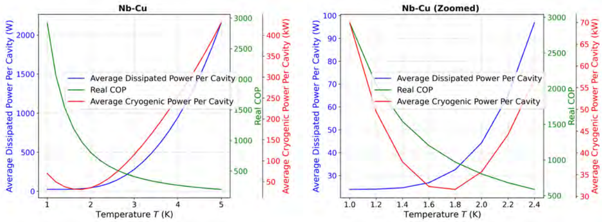
Figure 5.6: Normal-scale (left) and magnified (right) plots as functions of temperature, showing the average dissipated power per cavity (blue), the real coefficient of performance (COP) (green), and the average cryogenic power per cavity (red), for Nb on Cu cavities.
