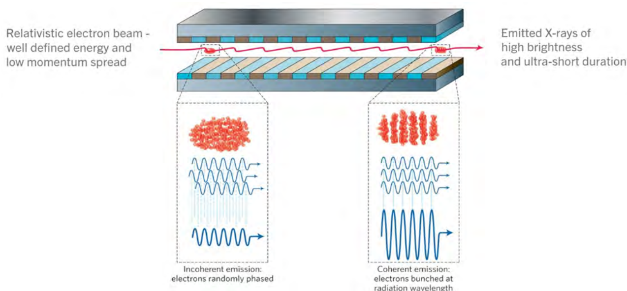
Figure 2.1: Schematic of the FEL mechanism. Bunches of randomly phased relativistic electrons propagate through a long array of alternating polarity dipole magnets (an undulator), which causes them to oscillate transversely and emit radiation. The transverse electric field of the co-propagating radiation couples to the electron transverse velocity allowing an energy exchange. This enables a positive feedback process in which the electrons start to micro-bunch, coherently enhancing their emission, which acts back on the electrons further enhancing the micro-bunching, and so on, giving an exponential growth of the radiation intensity. Figure reproduced from [3].
