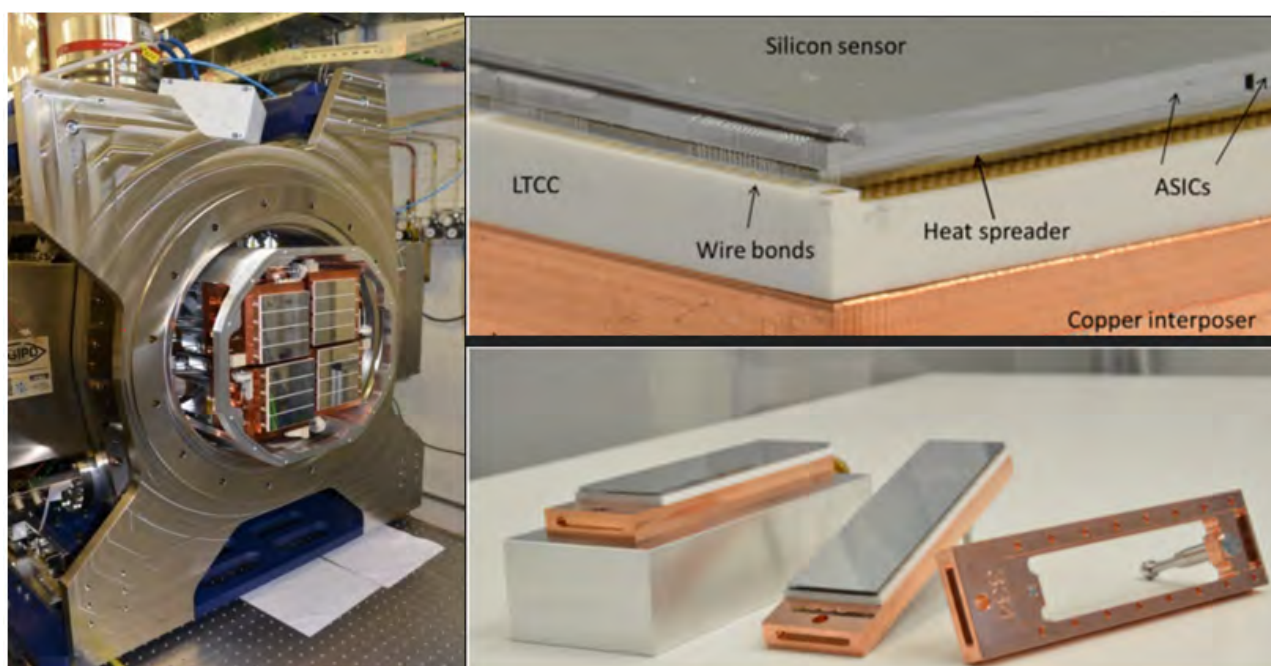
Figure 10.11: Example of the AGIPD detector module and array at the European XFEL. Credit: Heinz Graasfma, [51]
