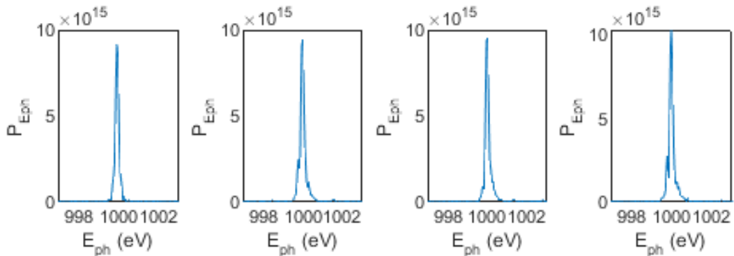
Figure 6.19: Hybrid Self-Seeding/HB-SASE Spectra at median position of maximum 6D brightness.
