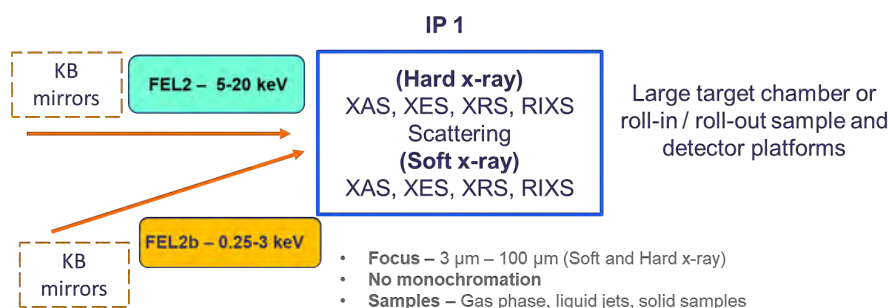
Figure 8.20: The ES11 end station for multi-colour X-ray experiments. Note - Since this needs to be a very flexible end station many detection techniques beyond those few listed here will need to be catered for at some stage.
