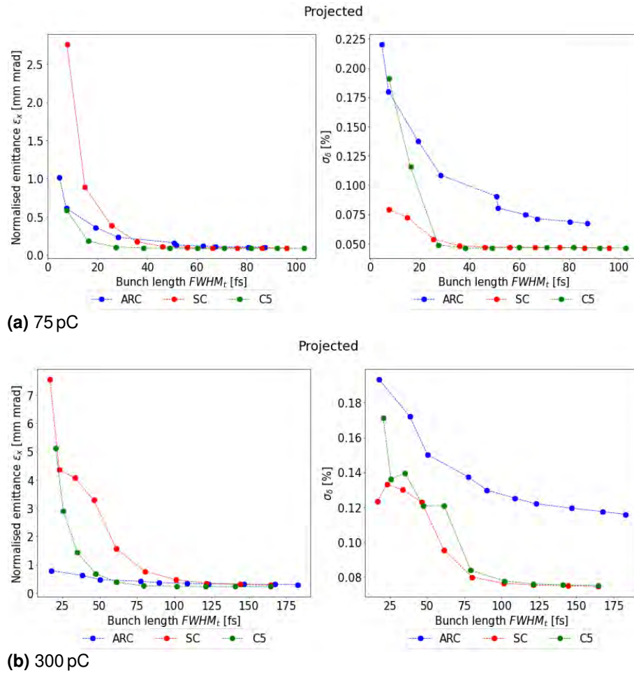
Figure 5.21: Projected bunch properties at the end of the linac as a function of bunch length for the three compression schemes considered at two different bunch charges (above: 75 pC; below: 300 pC). The plots on the left show the projected normalised emittance, and those on the right show the energy spread.
