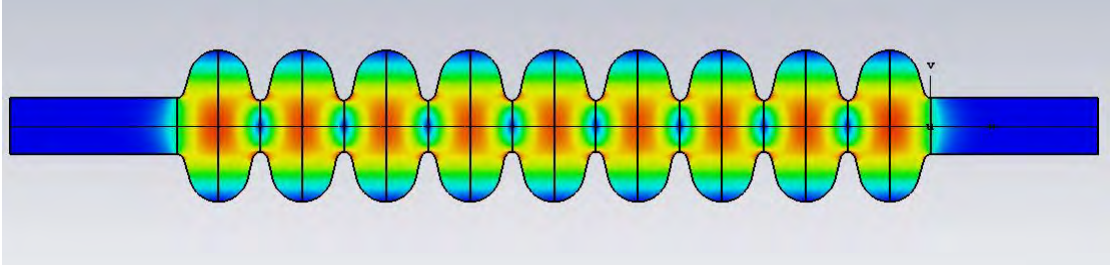
Figure 5.39: The main accelerating TM_{010} \pi mode of the TESLA 9-cell cavity rendered in CST.
