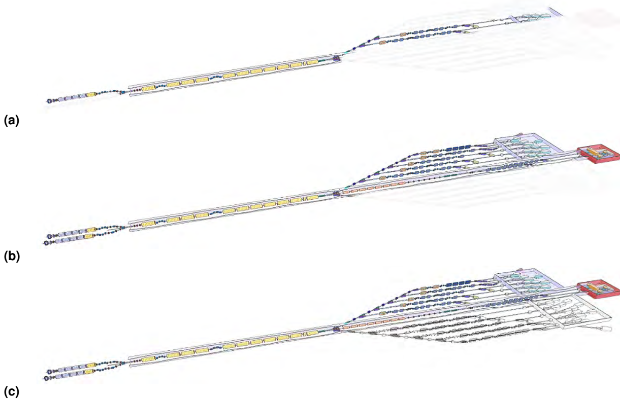
Figure 3.2: Scalable layout of the next-generation XFEL conceptual design, with different versions showing potential for a phased delivery (a) with 2 FELs (‘minimal’), (b) with 7 FELs (the ‘nominal’ case), (c) the ‘full’ realisation with 12 FELs. A repeating section of the SRF linac is omitted for clarity.
