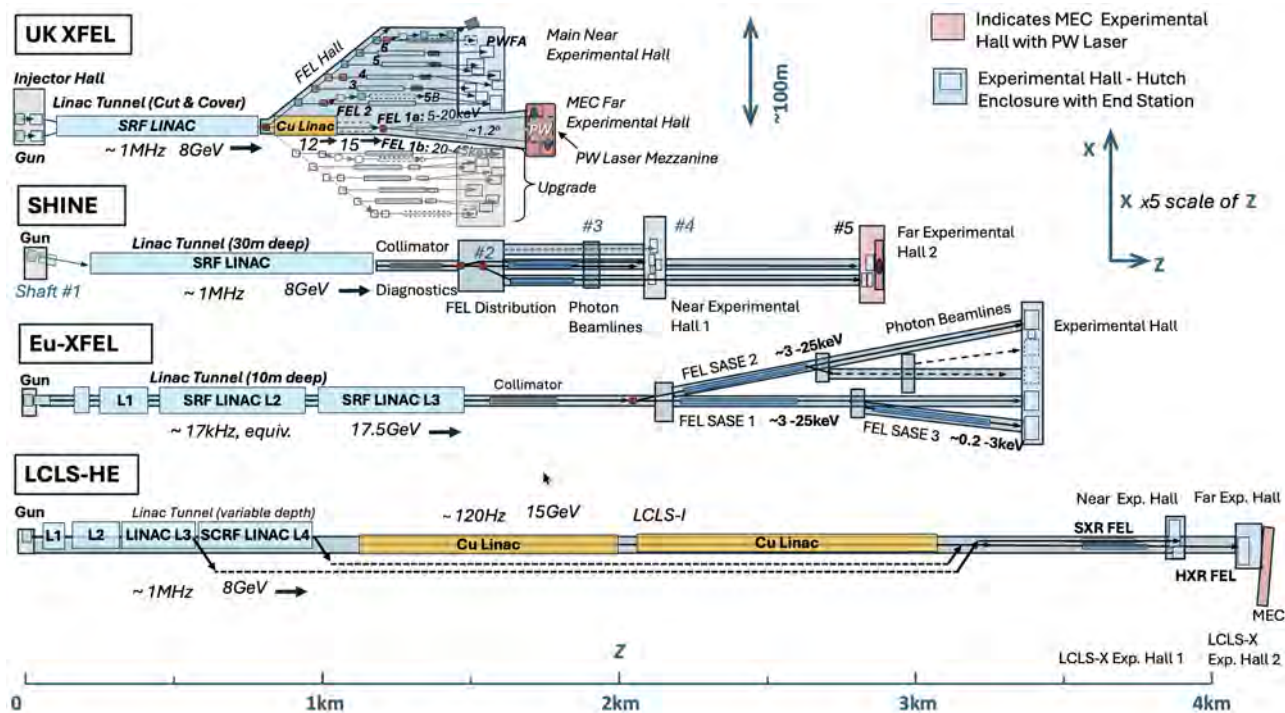
Figure 13.4: Approximately proportionally scaled schematic of UK XFEL in context of other Reference Facilities (with exaggerated \times 5 scaling in X to highlight features)
