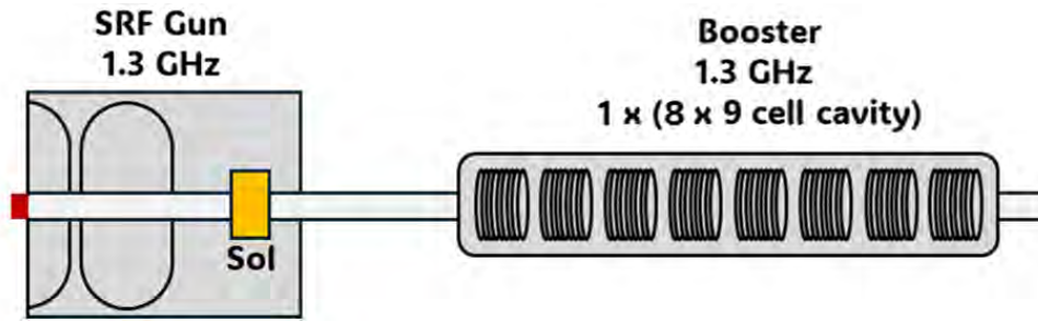
Figure 4.15: Outline schematic of the SRF L-band gun injector beamline.
