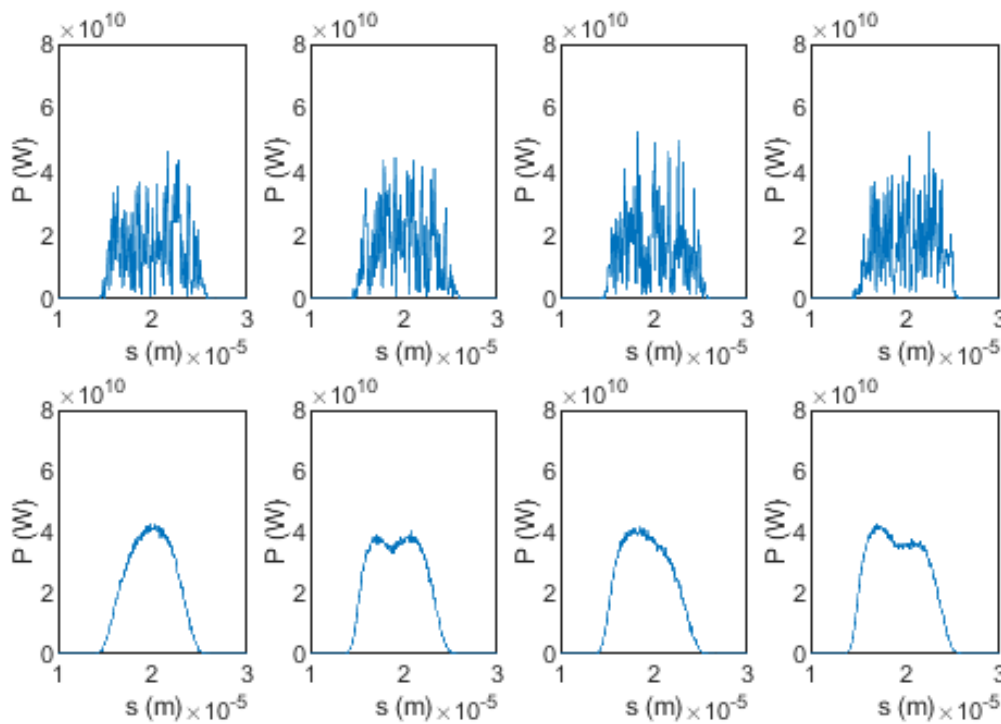
Figure 3.12: Example of the improvement in pulse quality, showing the temporal profile ( 10^{-5} m \equiv 33.3 fs), between SASE (top row) and advanced (self-seeded + HB-SASE) FEL techniques (bottom row) in the next-generation XFEL design.
