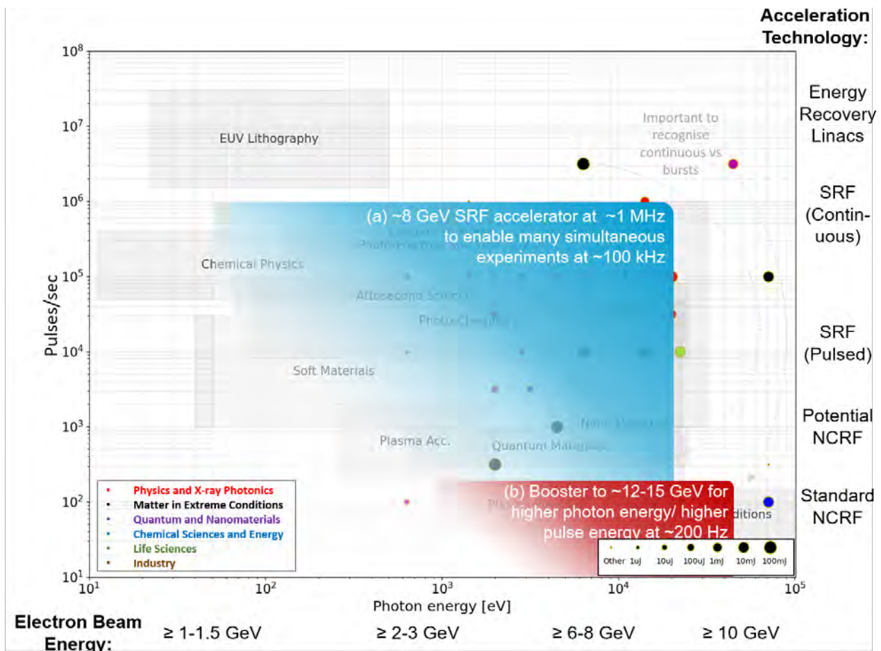
Figure 3.4: User requirements translated to high-level facility design choices for the next-generation XFEL conceptual design: (a) an \sim 8 GeV SRF linac operating at \sim 1 MHz to enable many simultaneous experiments at \sim 100 kHz, and a NCRF booster to 12-15 GeV at \leq 200 Hz. An unannotated version of this figure with clearer visibility of the user requirements is given in Figure 2.10
