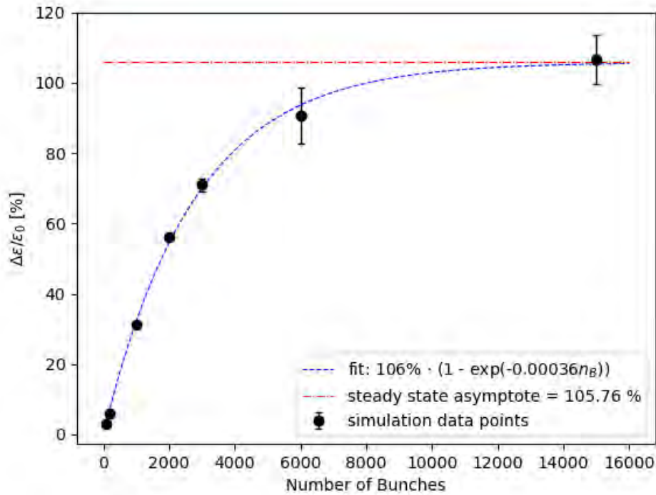
Figure 5.17: Unmitigated transverse emittance dilution due to a systematic 1\sigma transverse offset of the 150 pC beam returned by multiple PLACET simulations as a function of number of bunches included.
