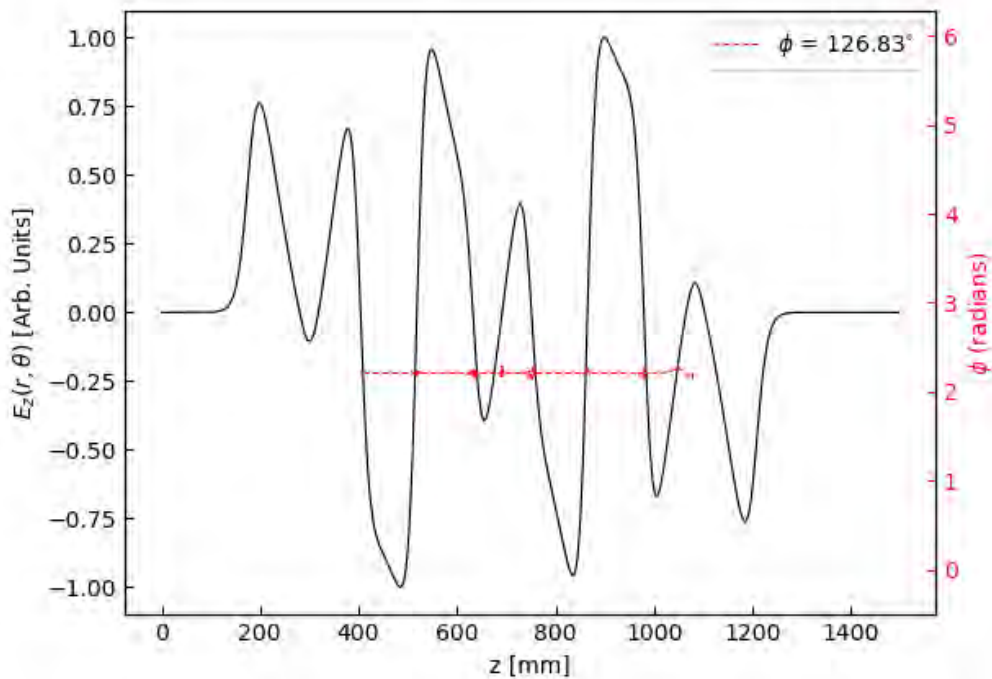
Figure 5.41: The normalised z component of the electric field of the 7 th TM_{110} dipole mode of the TESLA 9-cell cavity at a radial offset of 8 mm (black), with the phase advance ( \phi = 126.8^\circ ) calculated using Equation 5.24 plotted in red.
