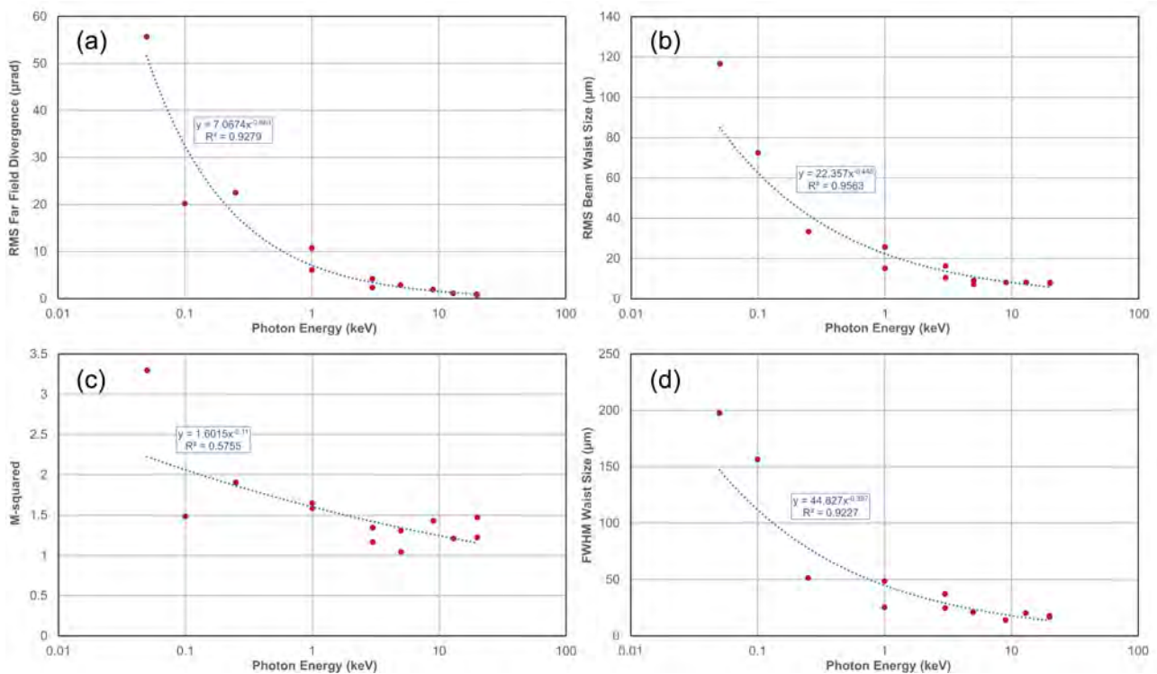
Figure 7.3: The average far-field divergence (a), RMS and FWHM waist sizes (b and d) and the beam quality factor (c), as derived from the M^2 analysis of all the FEL simulations, and the power law fits. When the model was developed it was planned for FEL-6 to operate down to 50 eV. Operation to this energy is now not being considered due to poor beam quality
