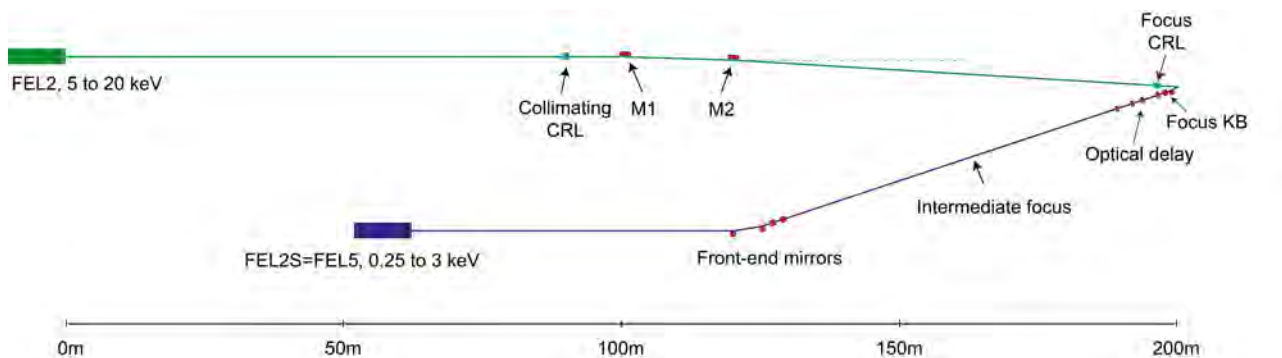
Figure 3.14: Layout of beamlines combining output of FEL-2 (hard X-ray) and its associated soft X-ray FEL (equivalent to FEL-5), separated by 3.2 m to a common interaction point.
