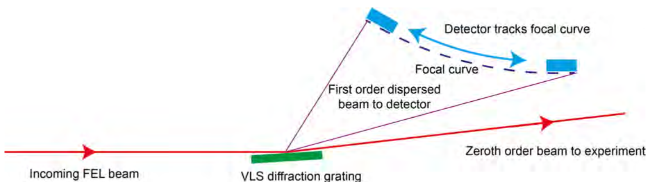
Figure 7.14: Concept of the VLS spectrometer for on-line spectrum measurement in the soft x-ray region
