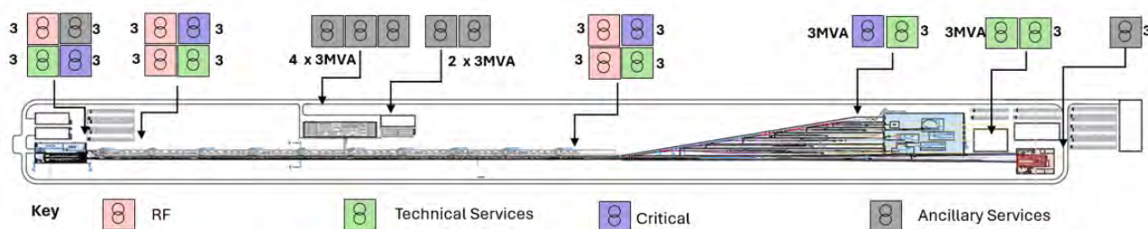
Figure 13.26: Electrical distribution scheme: Transformer locations and type
