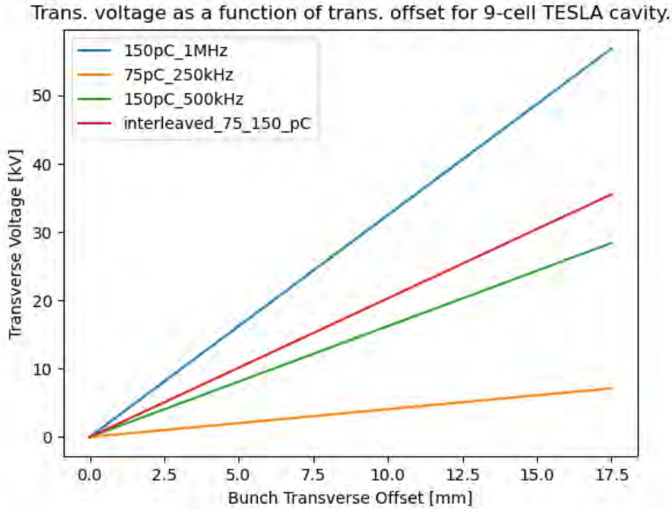
Figure 5.13: The transverse voltage delivered by the constituent 150 & 75 pC bunches as a function of radial offset and the sum of these being the V_{\perp}(r_{\perp}) of the composite beam. The case of a 150 pC beam running at a bunch repetition rate of 1 MHz is shown for reference.
