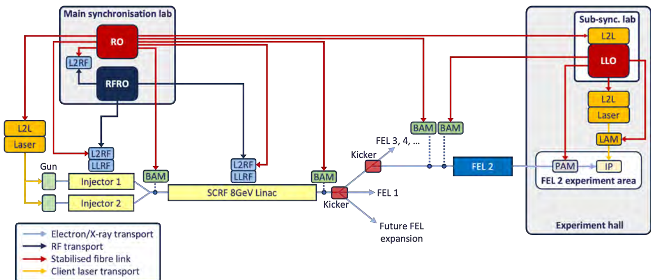
Figure 11.1: Example XFEL synchronisation architecture, as applied to the UK XFEL concept. This figure is for illustrative purposes only and does not reflect a final design decision. RO: Optical Reference Oscillator; RFRO: RF Reference Oscillator; LLO: Local Laser Oscillator; L2L: Laser-to-Laser synchronisation; L2RF: Laser-to-RF synchronisation; BAM: Beam Arrival Monitor; PAM: Photon Arrival Monitor; IP: Interaction point (laser and X-ray).
