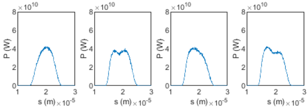
Figure 6.23: Hybrid Self-Seeding/HB-SASE pulses at median position of maximum 6D brightness.
