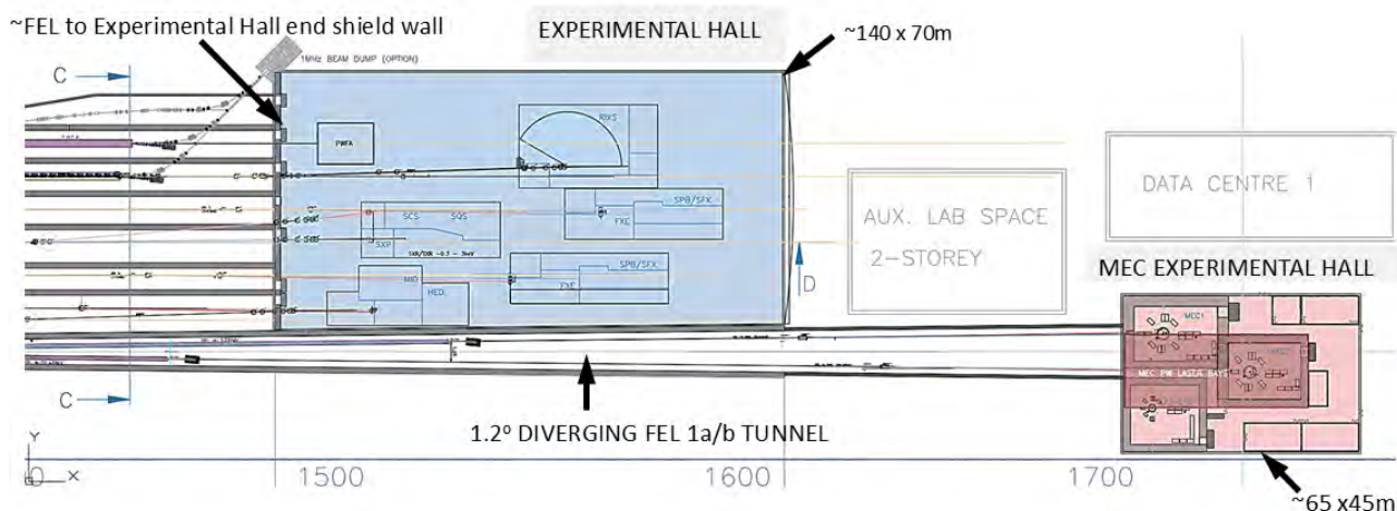
Figure 13.13: Experimental Halls in Plan (Spanning from 1.4km to 1.8km S.P.)
