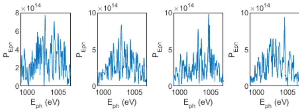
Figure 6.16: SASE Spectra at median position of maximum 6D brightness.
