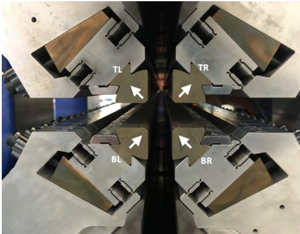
Figure 6.32: View looking along the electron beam axis of an APPLE-X Undulator. Credit: M.Calvi - SwissFEL talk 2021
