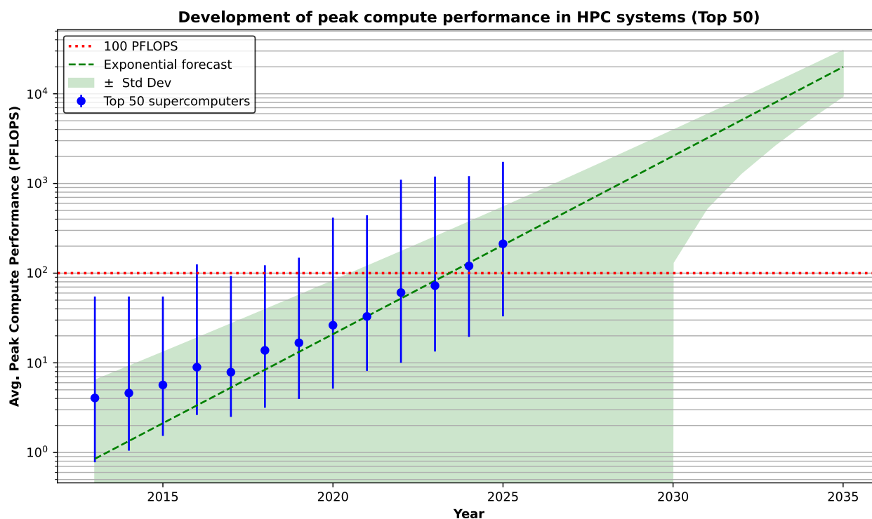
Figure 12.3: Nominal 100 PFLOP HPC facility compared to Top 500 HPC rankings.
