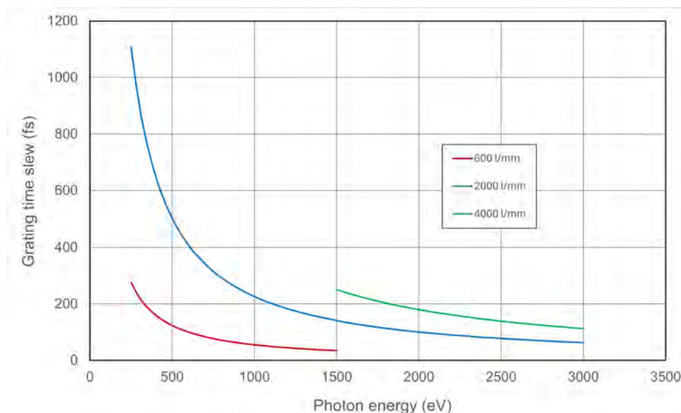
Figure 7.9: Time slew from the pulse front tilt of the RIXS monochromator concept
