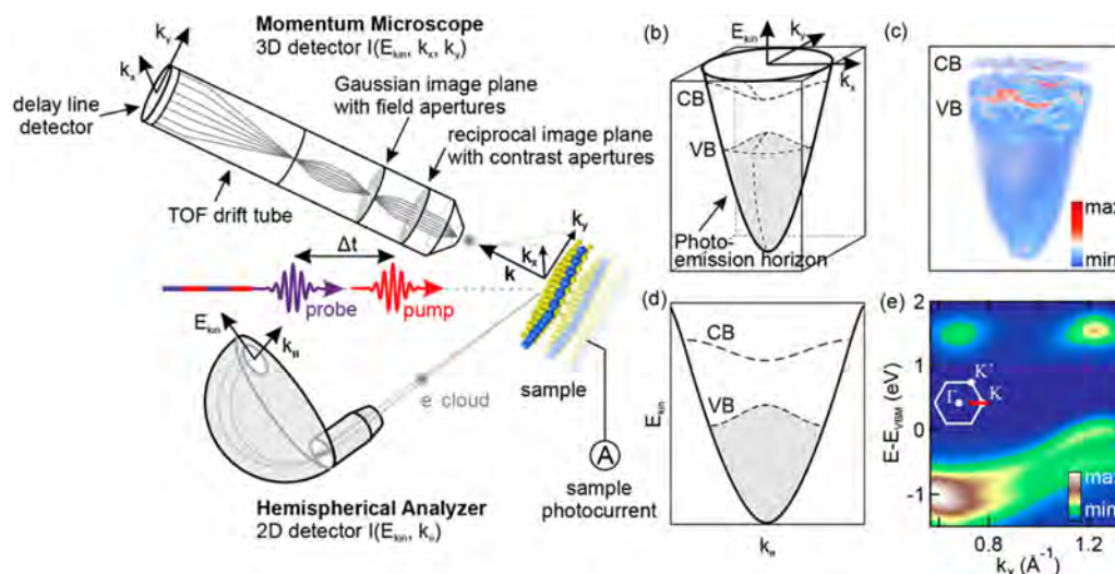
Figure 8.6: Schematic of two common detection techniques for trARPES measurements - the hemispherical analyser and the momentum microscope - illustrated here for a sample of bulk tungsten diselenide. Adapted from J. Maklar et al. Rev. Sci. Instrum. 91, 123112 (2020). Reproduced under terms of the Creative Commons Attribution License 3.0 BY
