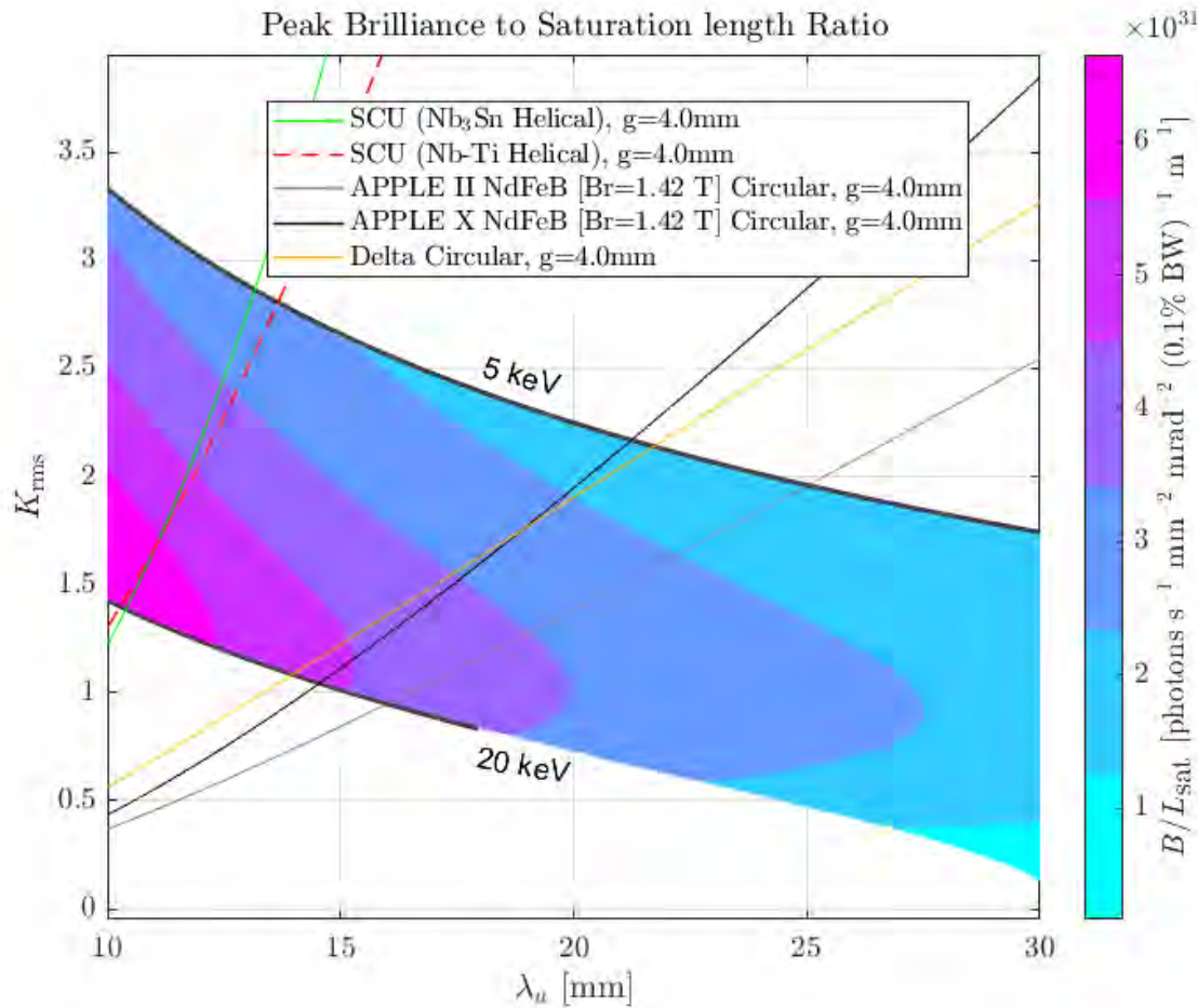
Figure 6.35: Undulator Technology Options for FEL-2
