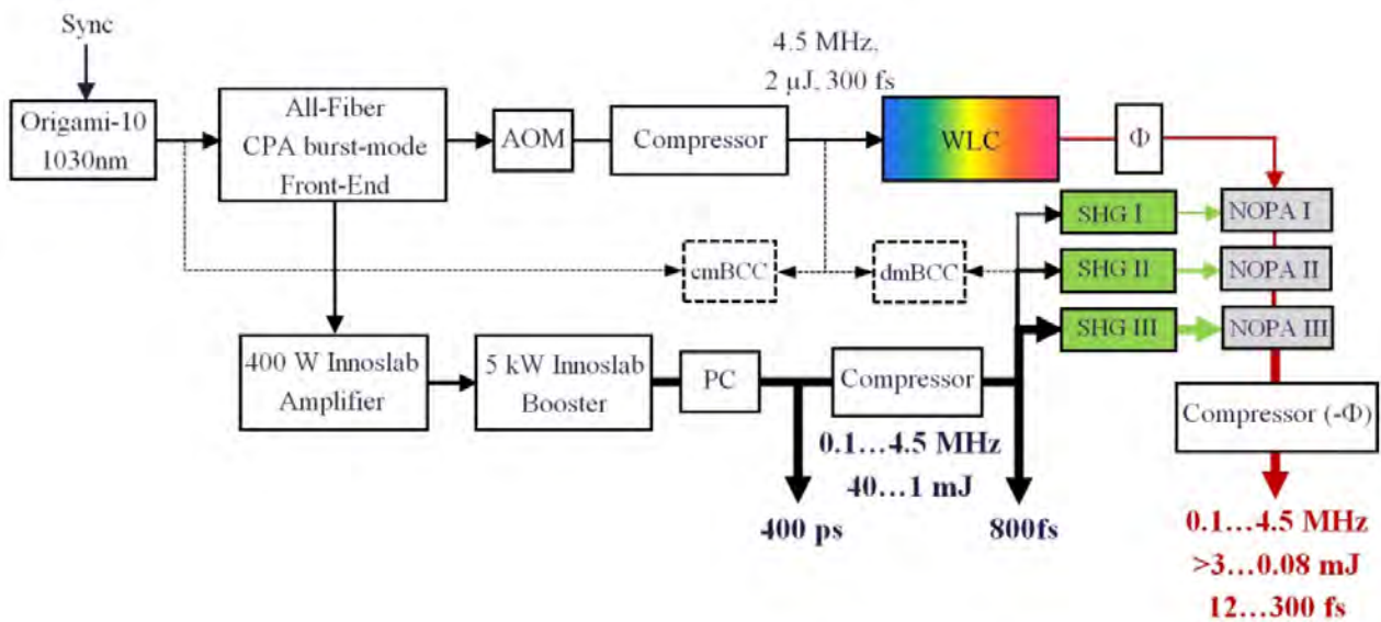
Figure 9.5: Schematic of the PP-laser prototype: AOM (Acousto-Optical Modulator), PC (Pockels cell), SHG (Second Harmonic Generation), \Phi (dispersion management with multi-bounce chirped mirrors and/or material), cmBCC (common mode Balanced Cross Correlator), dmBCC (differential mode Balanced Cross Correlator), NOPA (Non-collinear Optical Parametric Amplifier). Seed and pump beams are controlled by beam pointing stabilization systems. Replicated from [7].
