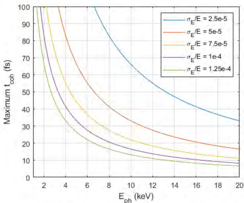
Figure 6.14: Estimate of maximum coherence time vs FEL photon energy, for different beam energy spreads.
