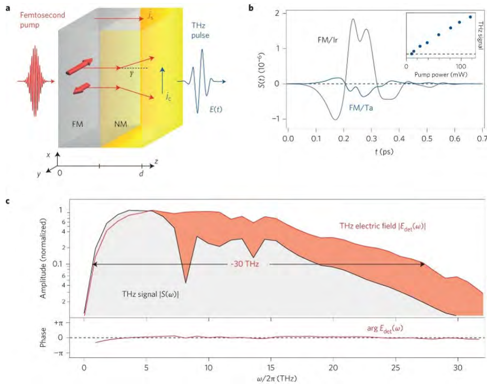
Figure 9.14: Replicated from [30]. “Metallic spintronic terahertz emitter. a, Principle of operation. A femtosecond laser pulse excites electrons in the metal stack, thereby changing their band velocity and launching a current along the z direction. Because in the FM layer the mobility of spin-up (majority) electrons is significantly higher than that of spin-down (minority) electrons, the z current is spin-polarized. In the NM layer, spin-orbit interaction deflects spin-up and spin-down electrons in opposite directions and transforms the spin current j_s into an ultrafast transverse charge current j_c = \gamma j_s , leading to the emission of a terahertz electromagnetic transient. b, Typical electrooptic signal S(t) of terahertz pulses obtained from photoexcited Ta- and Ir-capped \text{Co}_{20}\text{Fe}_{60}\text{B}_{20} thin films and detected by a 50\text{-}\mu\text{m} -thick GaP crystal. Inset: Terahertz signal amplitude as a function of incident pump power. c, Fourier spectra of terahertz signal S(t) and the extracted transient terahertz electric field E_{\text{det}}(t) incident on the electrooptic detector. Both spectra are normalized to peak amplitude 1. The double-headed arrow illustrates the 30 THz large bandwidth of the emitter. The flat spectral phase indicates that the terahertz pulse is Fourier-limited.”
