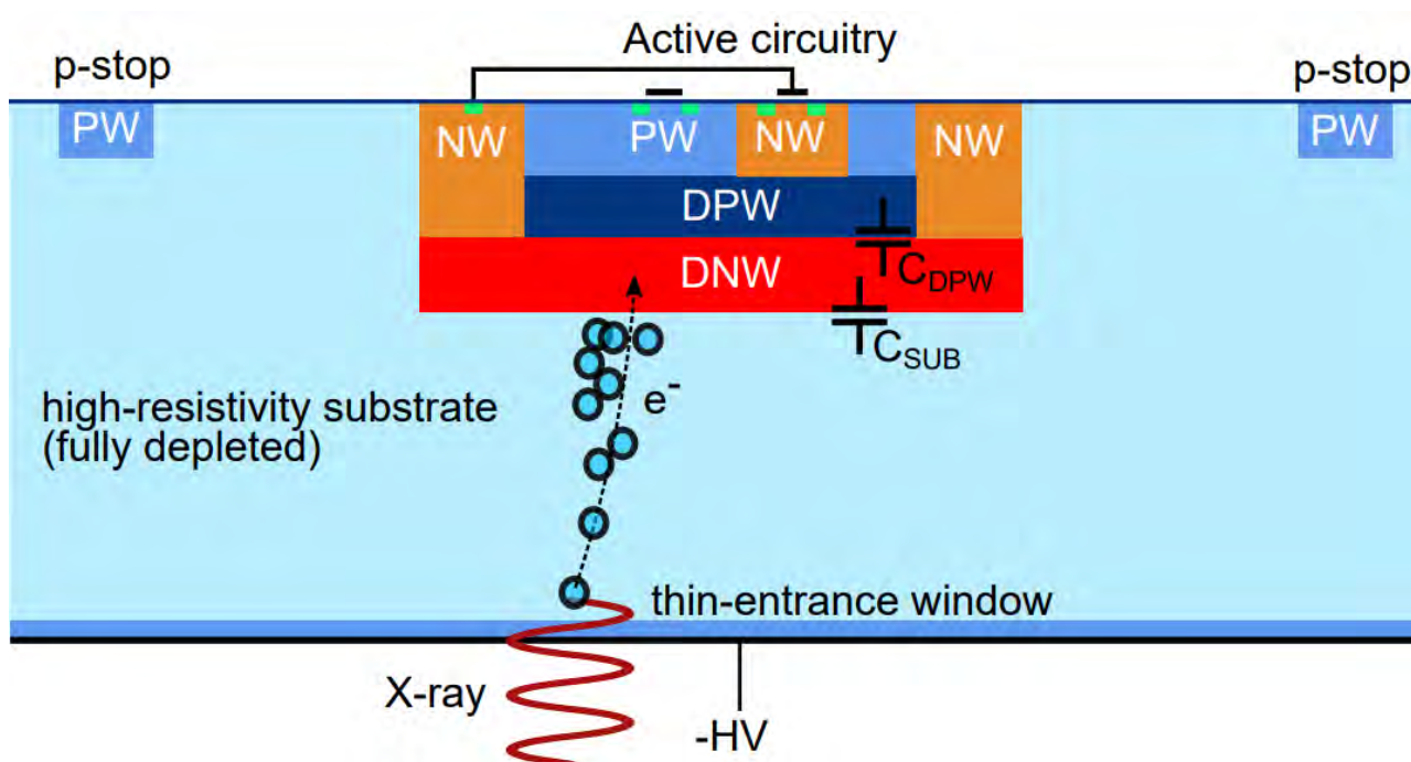
Figure 10.4: Cross section of ePix-M. Credit: L. Rota
