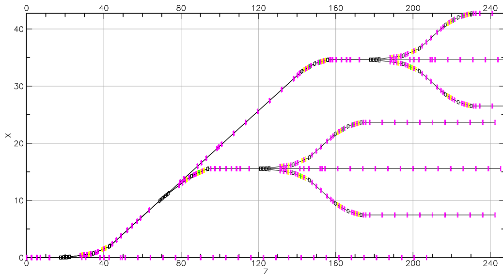
Figure 5.28: Trident spreader layout.
