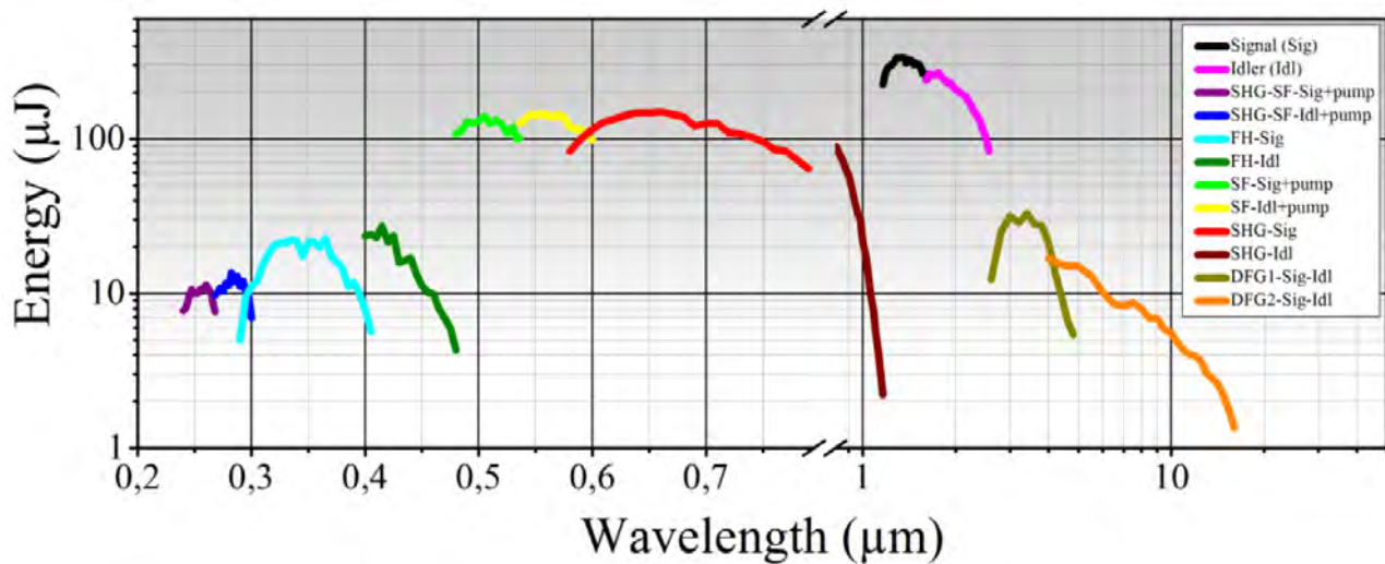
Figure 9.6: Illustrative tuning range from a TOPAS system pumped at 800 nm.[7]
