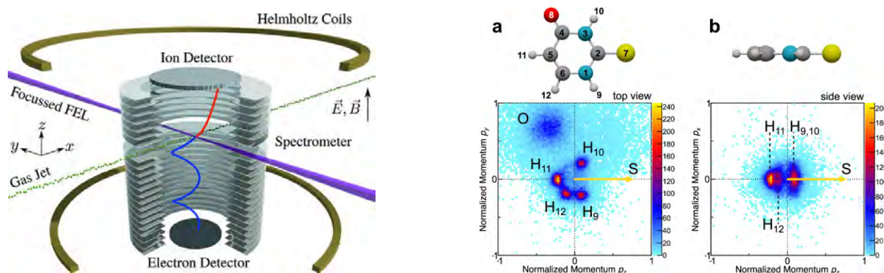
Figure 8.3: (Left) - Principle of operation of a reaction microscope. Reproduced from G. Schmid et al. J. Synchrotron Rad. 26 , 854-867 2953 (2019) (Right) - Coulomb explosion momentum-space images of 2-thiouracil obtained from the COLTRIMS reaction microscope at SQS on European XFEL. (a) Top view projection of the measured momentum-space data of the oxygen ions and the protons (b) "Side view" projection of the measured proton momenta. Figure adapted from T. Jahnke et al. Nat Comms. 16 2074 (2025).
