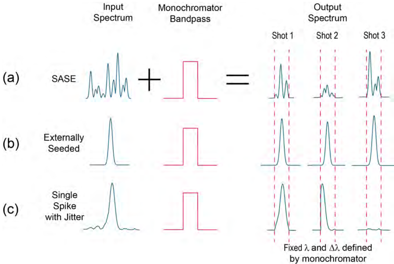
Figure 7.4: How a monochromator can interact with a FEL source. In (a) the source operates in SASE mode; the monochromator will define a narrower spectral range and stabilise the central wavelength at the expense of increased jitter in the pulse energy. In (b) with an externally seeded source, the FEL pulse is stable in both central wavelength and pulse width and the monochromator has no worthwhile effect. In (c) with a single-spike mode, there is jitter in the central wavelength and unwanted spectral contamination. However, the jitter prevents the monochromator from removing the contamination without also modifying the core pulse.
