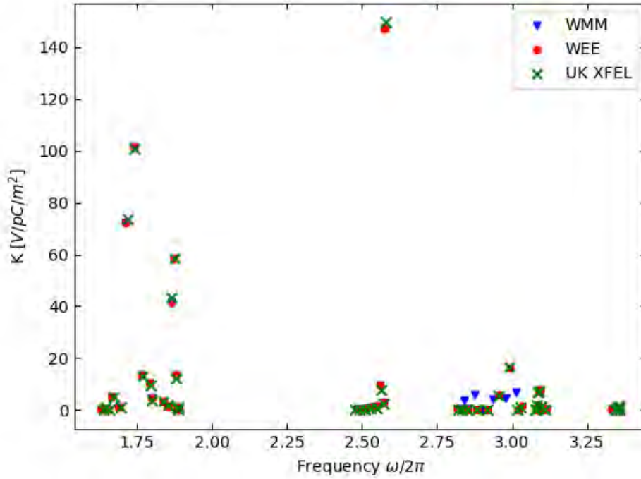
Figure 5.10: Plot comparing the frequencies and kick factors of each mode in the first six dipole passbands to published results [31].
