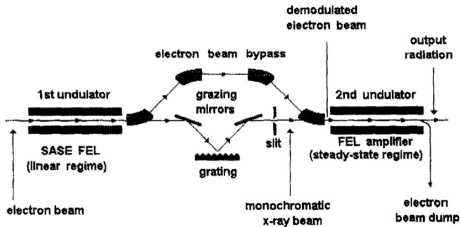
Figure 6.4: Schematic of the original self-seeding concept. Reproduced from [17].
