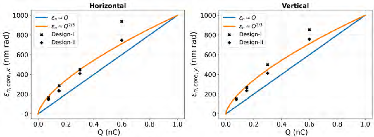
Figure 4.14: Final horizontal and vertical core emittances for Design-I and Design-II across all simulated bunch charges. Emittance values are compared with two theoretical scaling laws (shown as blue and orange lines).
