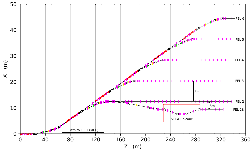
Figure 3.8: Spreader layout for the nominal case. In the full version, this layout is reflected about the z-axis. The FEL-2 line includes an RF deflector to an adjacent undulator line for two-colour operation.
