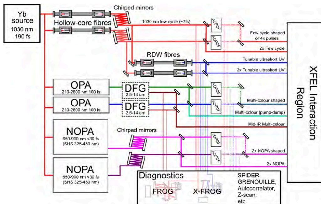
Figure 3.19: Proposed optical arrangement of systems and diagnostics available at an ideal ultrafast XFEL beamline, with an example of an Yb pump laser. Figure reproduced from [65].
