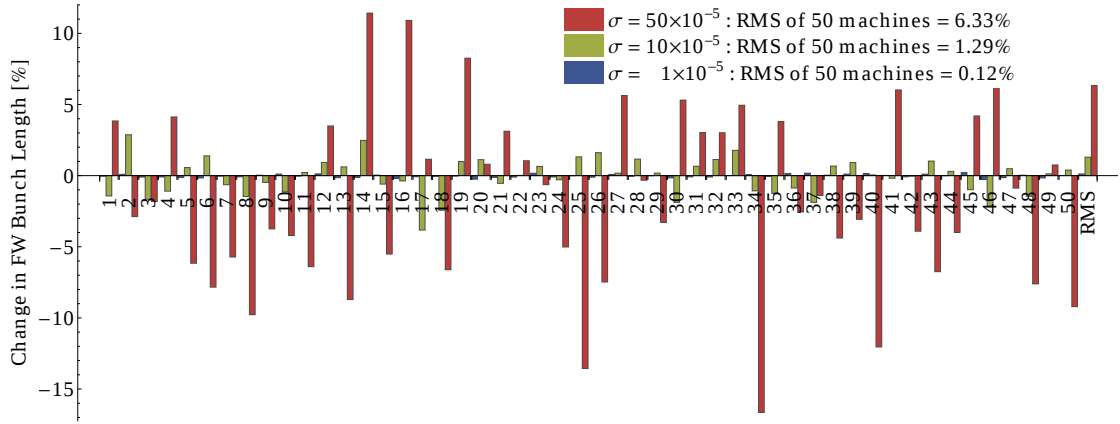
Figure 8: Change in FW bunch length for three sets of 50 machines with Gaussian distributed errors in quadrupole field strength with standard deviation shown. We see that the derived RMS of the 50 machines (final column) rises linearly with the standard deviation of the errors.
