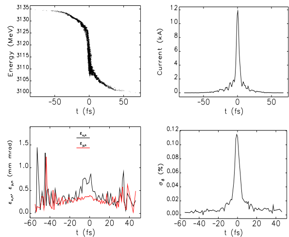
Figure 2: Baseline (SPF) final bunch properties: (1) longitudinal phase space, (2) current profile, (3) slice emittances & (4) slice energy spread.
