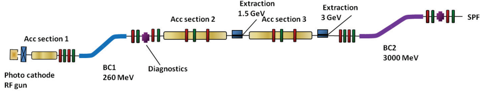
Figure 1: Layout of the Max-IV linac.
