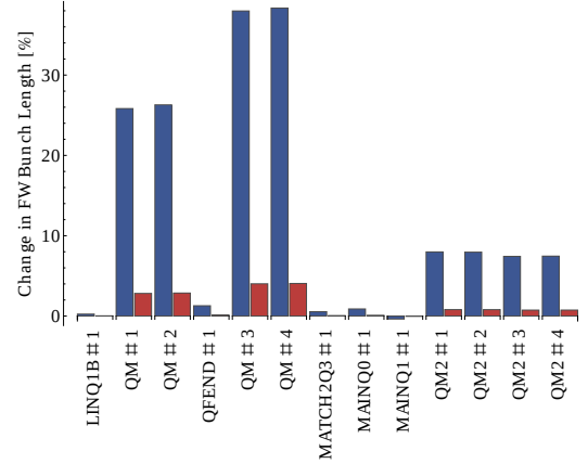
Figure 3: Change in FW bunch length from nominal on variation of quadrupole field strength by +0.5% (blue) and +0.05% (red). Only machines where change \geq 0.02\% shown. The largest 8 are within the two bunch compressors (with BC1 dominating).
