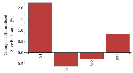
Figure 7: Change in normalised slice emittance at peak current slice from nominal on variation of sextupole field strength by +0.5%.
