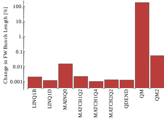
Figure 5: Change in FW bunch length on addition of +0.5% normal 12-pole field error to labelled quadrupole. Only machines where change \geq 0.001\% shown.
