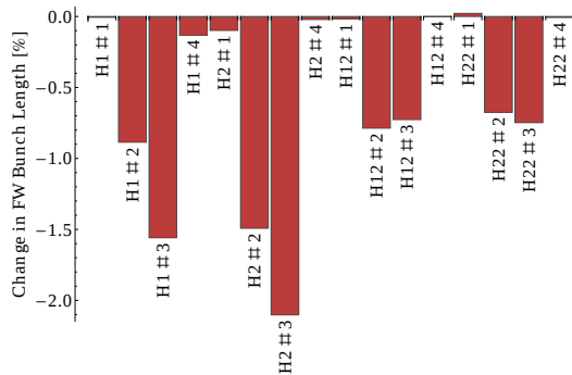
Figure 6: Change in FW bunch length under a 10 \mu\text{rad} dipole roll. Each dipole is treated independently.
