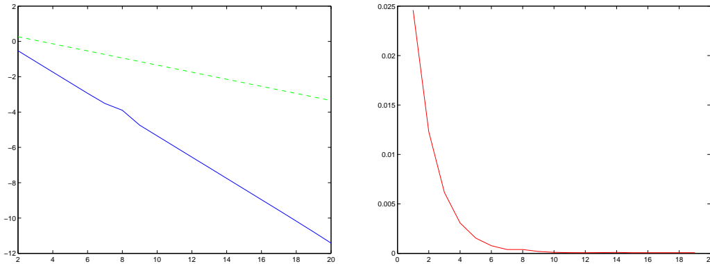
Figure 3.1: Evaluation of \tau(n) and \theta(n) (dashed) (left, in \log_{10} scale) and \delta(n) (right) as functions of n .
