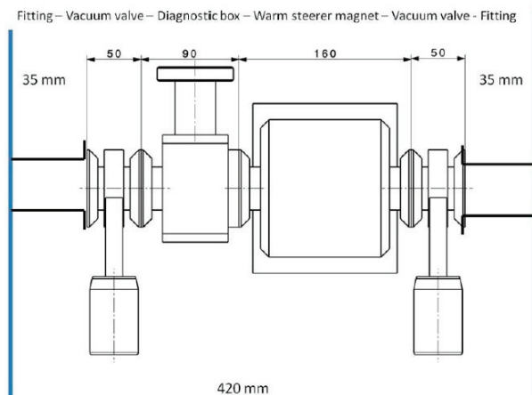
Figure 7: Layout of the inter cryomodule region.
