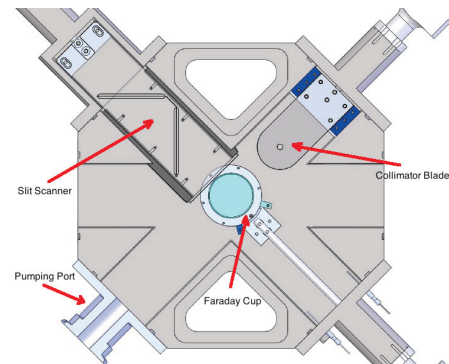
Figure 2: 3D model of the diagnostic box (Developed by AVS).
