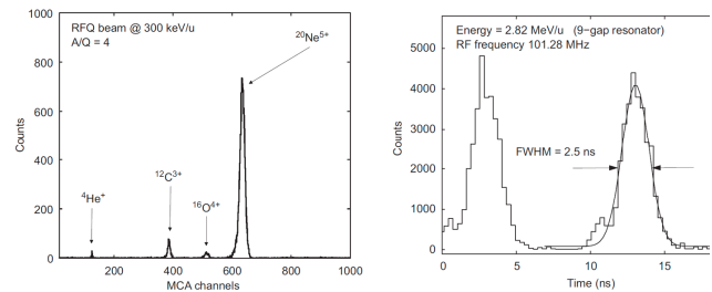
Figure 5: Energy and time spectrum of the Si-det. [4]
