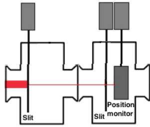
Figure 6: Operating principle of the emittance meter.
