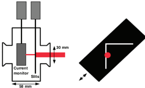
Figure 4: Operating principle of the profile monitor based on a slit scanner and the FC.
