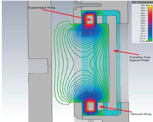
Figure 3: Simulation of the potential distribution in the Faraday Cup.
