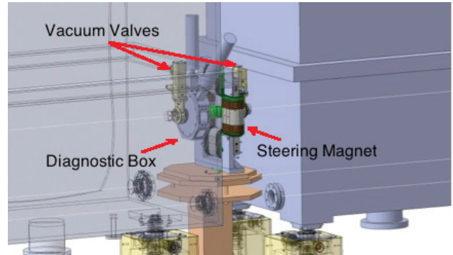
Figure 1: 3D model of a diagnostic box in the region between cryomodules.
