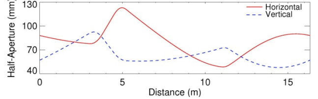
Figure 7: Horizontal and vertical half apertures over one superperiod of the ISIS synchrotron.
