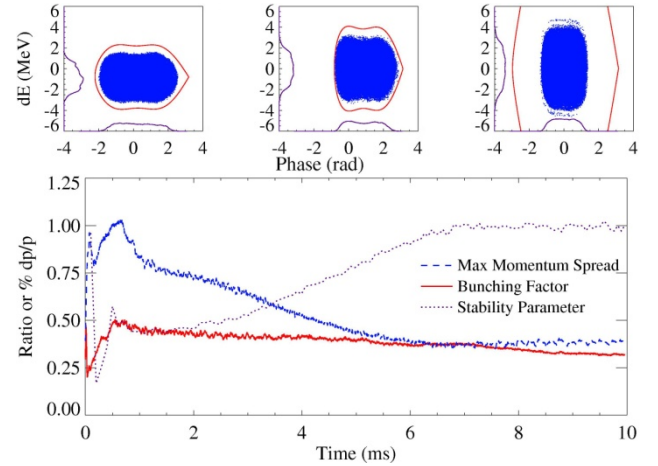
Figure 6: Phase space at the end of injection, 5 and 10 ms and evolution of bunching factor, stability parameter (Eq. 2) and maximum dp/p for injection scheme three.
