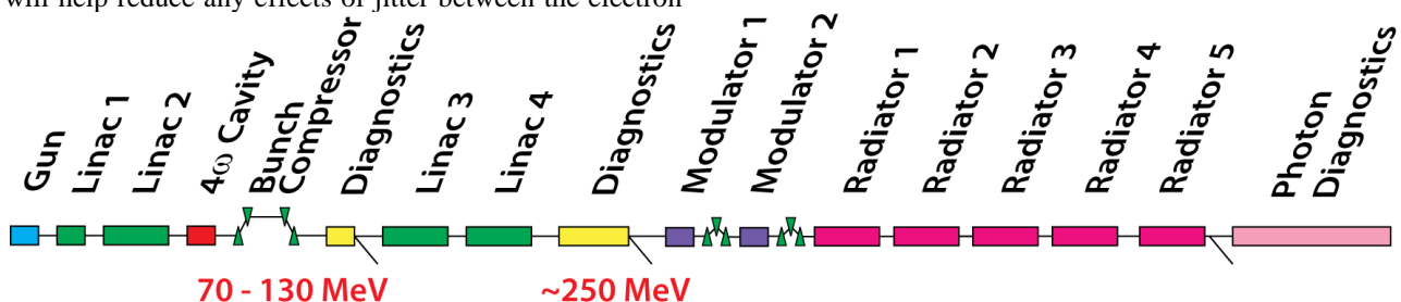
Figure 1: CLARA Schematic
