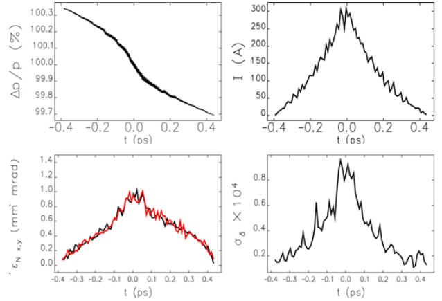
Figure 7: Short pulse velocity bunched beam (Top left) Longitudinal phase space (top right) Current profile (bottom left) Normalised slice emittances (40 fs slices) (Bottom right) slice energy spread
