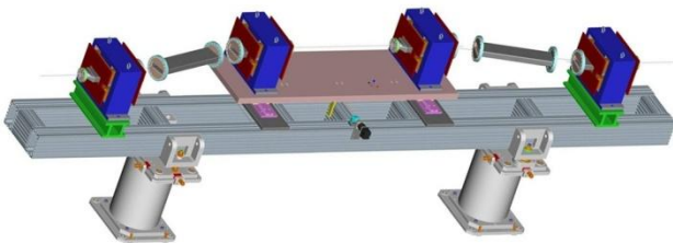
Figure 4: Variable bunch compressor
