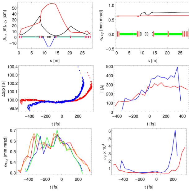
Figure 6: (Top left) \beta_{x,y} (black, red) and \eta_x , (top right) emittance ( x,y ), (middle left) Longitudinal phase space (blue - optimised for 200 fs flat top, red - optimised for 300 fs flat top). (middle right) Current profile (40 fs slices, optimised for 200 fs flat top, red - optimised for 300 fs flat top). (bottom left) Normalised slice emittances (40 fs slices): horizontal / vertical (blue / red - optimised for 200 fs flat top, green / orange - optimised for 300 fs flat top) (bottom right) Slice energy spread (20 fs slices) optimised for 200 fs flat top, red - optimised for 300 fs flat top.
