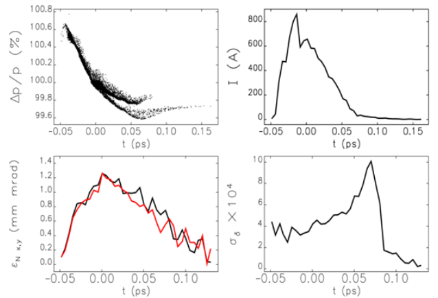
Figure 8: Ultra-short pulse velocity bunched beam (Top left) Longitudinal phase space (top right) Current profile (bottom left) Normalised slice emittances (40 fs slices) (Bottom right) slice energy spread
