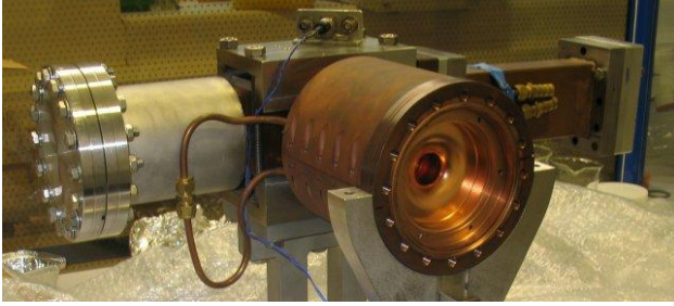
Figure 2: The EBTF/ALPHA-X photoinjector gun.
