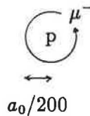
Muonic hydrogen
