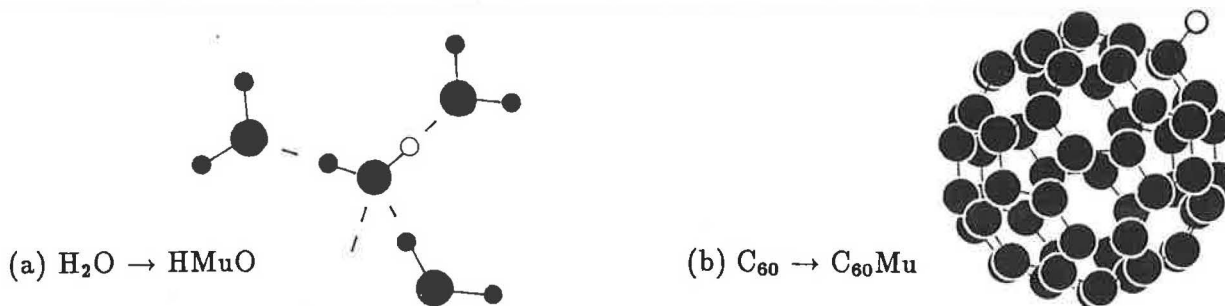
Muonium substituted in a closed shell molecule (a) and incorporated in an open-shell molecule (b) [3].
