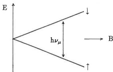
Spin- \frac{1}{2} energy levels.
