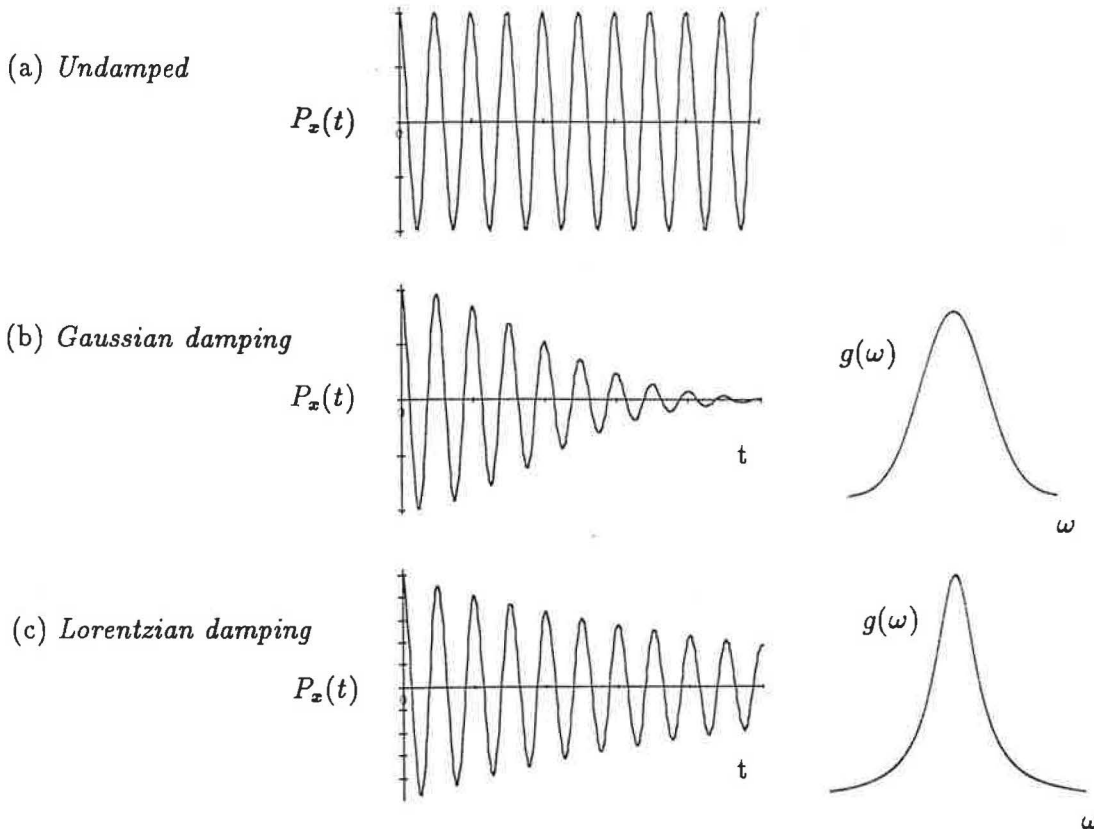
Time and frequency domain signals.
