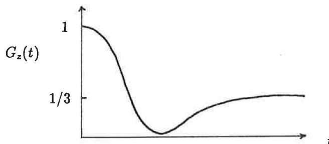
Kubo-Toyabe zero-field relaxation function.
