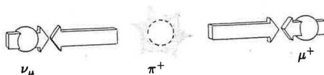
Pion decay to spin-polarized muons (2)
