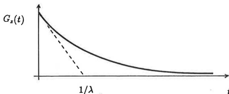
Single exponential relaxation.
