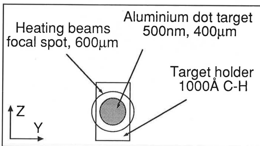
Fig.1(b) Schematic of the dot targets used for the experiment
